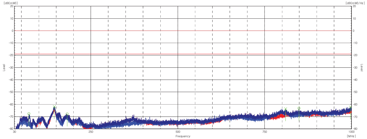
[30 MHz - 1 GHz]
