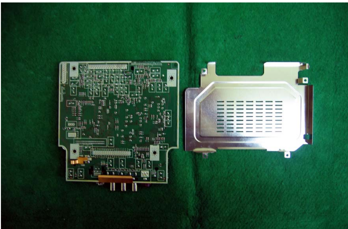
DVD PCB View (Bottom)
