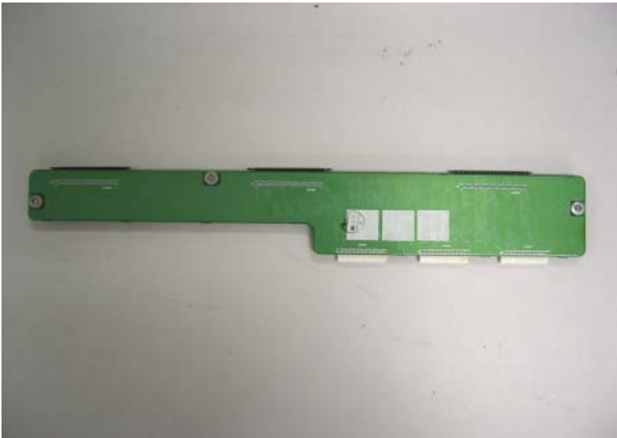
X buffer low board bottom view
