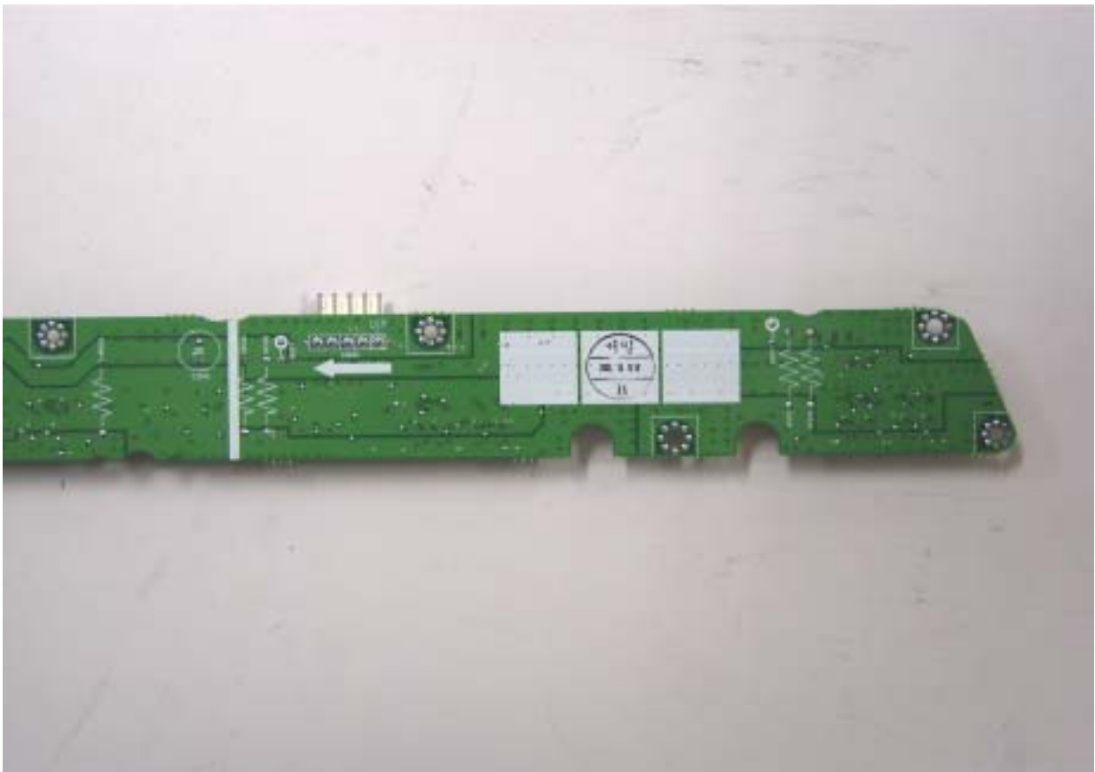
E buffer board bottom view
