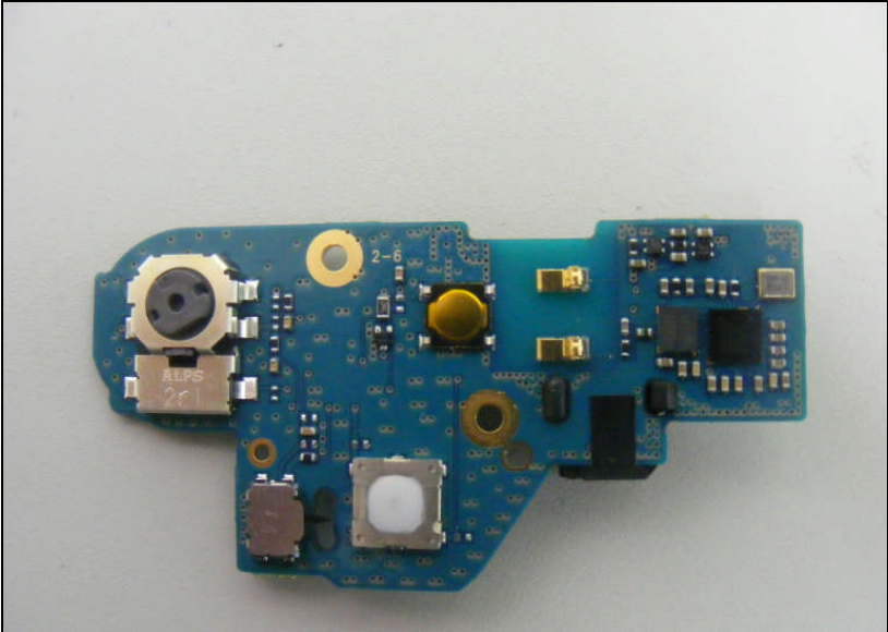
Bottom view of Sub-PCB 2
