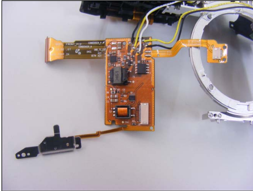
Bottom view of FPCB2
