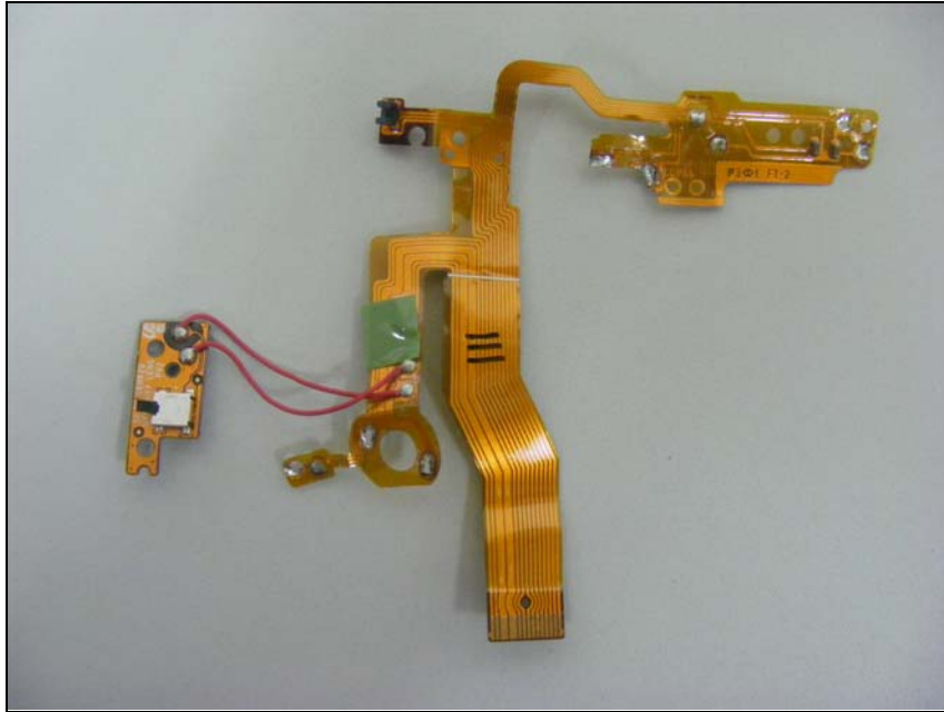
Top view of FPCB1
