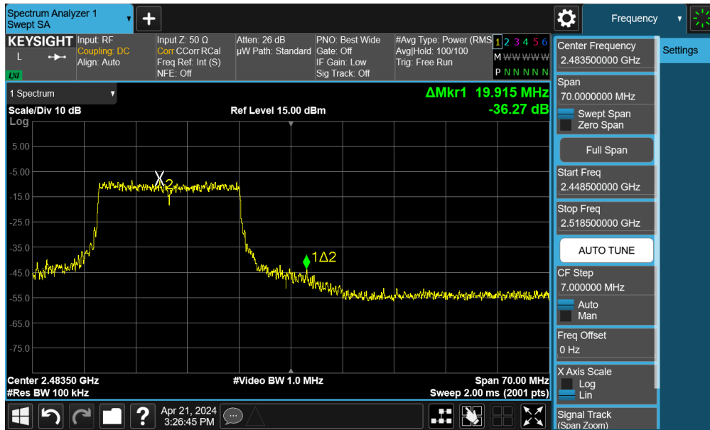
Plot 7-44. Band Edge Plot SISO ANT2 (802.11be OFDMA – 242 Tones – Ch. 12)
