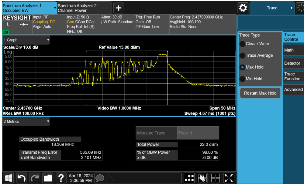
Plot 7-15. 6dB Bandwidth Plot MIMO ANT2 (802.11be OFDMA – 26Tones – Ch. 6)
