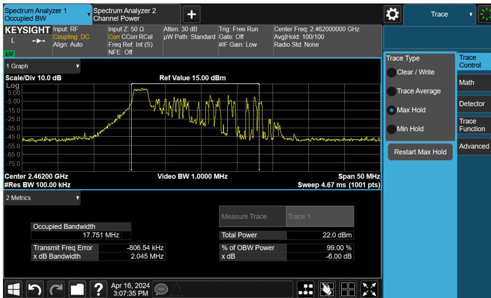
Plot 7-16. 6dB Bandwidth Plot MIMO ANT2 (802.11be OFDMA – 26Tones – Ch. 11)
