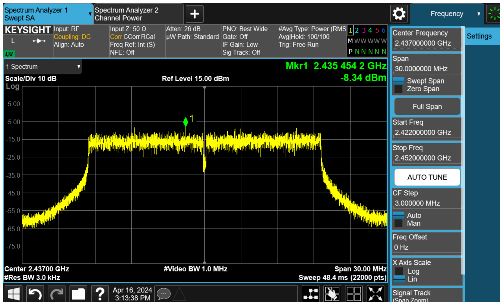
Plot 7-36. Power Spectral Density Plot MIMO ANT2 (802.11be OFDMA – 242 Tones – Ch. 6)
