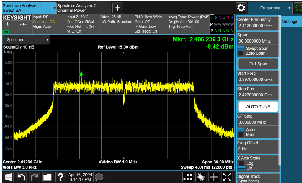
Plot 7-35. Power Spectral Density Plot MIMO ANT2 (802.11be OFDMA – 242 Tones – Ch. 1)
