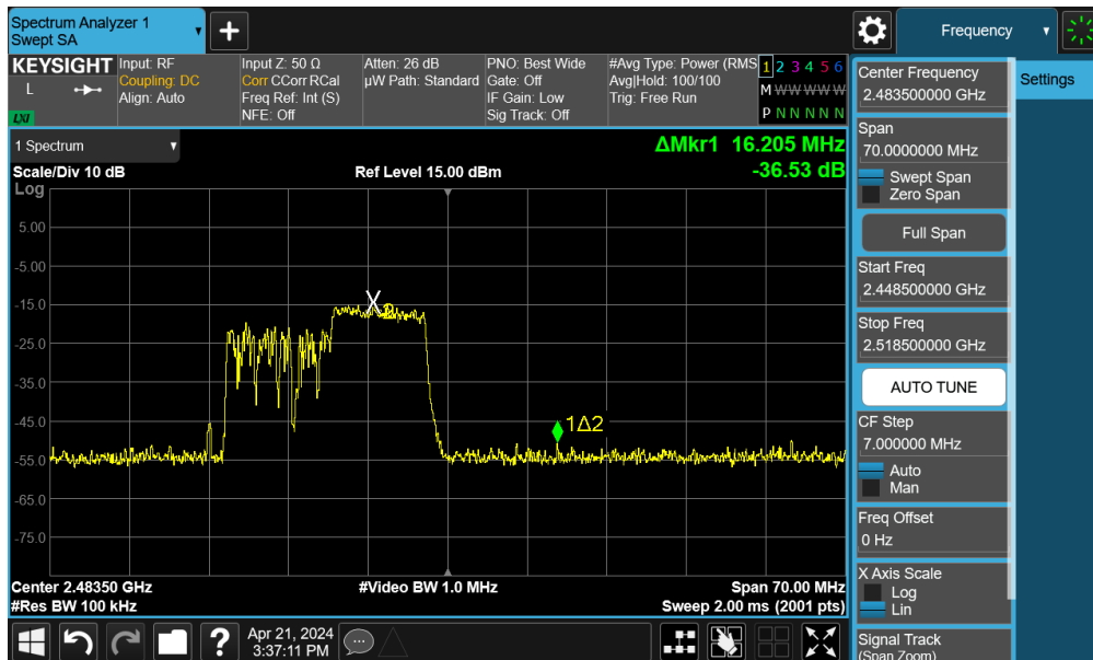
Plot 7-49. Band Edge Plot MIMO ANT1 (802.11be OFDMA – 106 Tones – Ch. 13)
