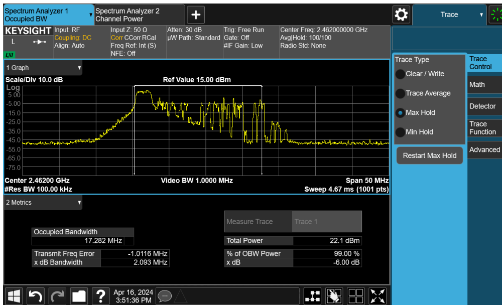
Plot 7-10. 6dB Bandwidth Plot MIMO ANT1 (802.11be OFDMA – 26Tones – Ch. 11)
