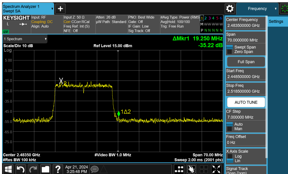
Plot 7-45. Band Edge Plot SISO ANT2 (802.11be OFDMA – 242 Tones – Ch. 13)
