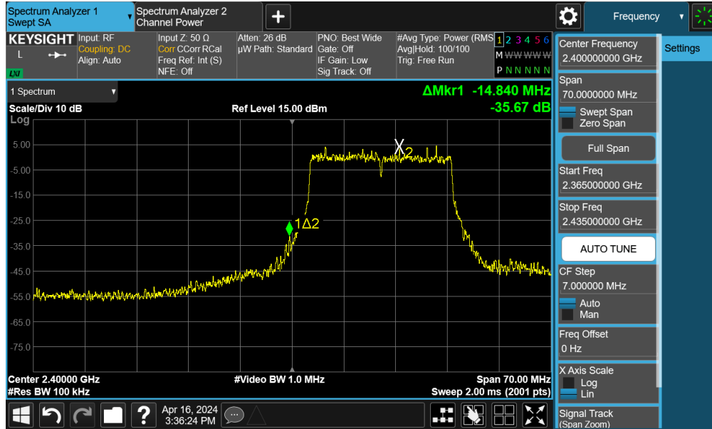
Plot 7-42. Band Edge Plot SISO ANT2 (802.11be OFDMA – 242 Tones – Ch. 1)
