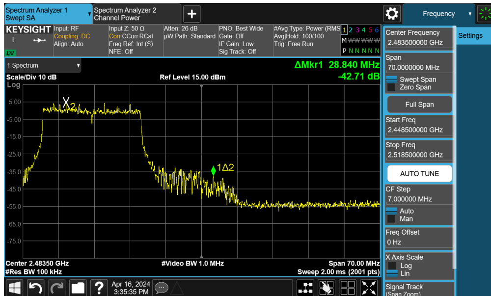
Plot 7-43. Band Edge Plot SISO ANT2 (802.11be OFDMA – 242 Tones – Ch. 11)
