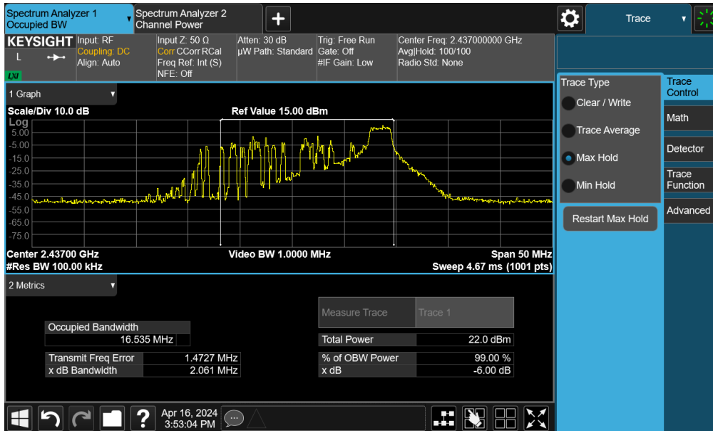
Plot 7-9. 6dB Bandwidth Plot MIMO ANT1 (802.11be OFDMA – 26Tones – Ch. 6)
