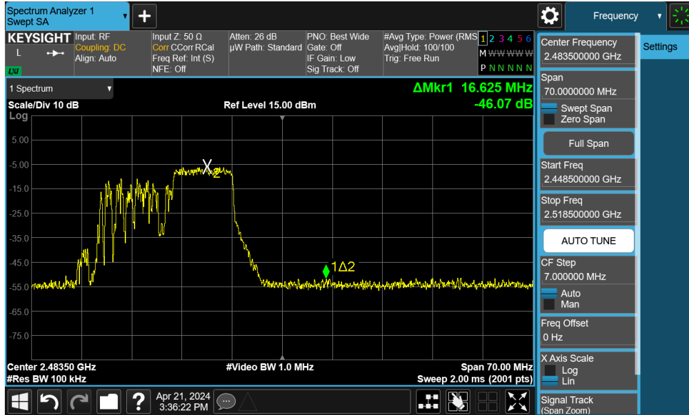
Plot 7-48. Band Edge Plot MIMO ANT1 (802.11be OFDMA – 106 Tones – Ch. 12)
