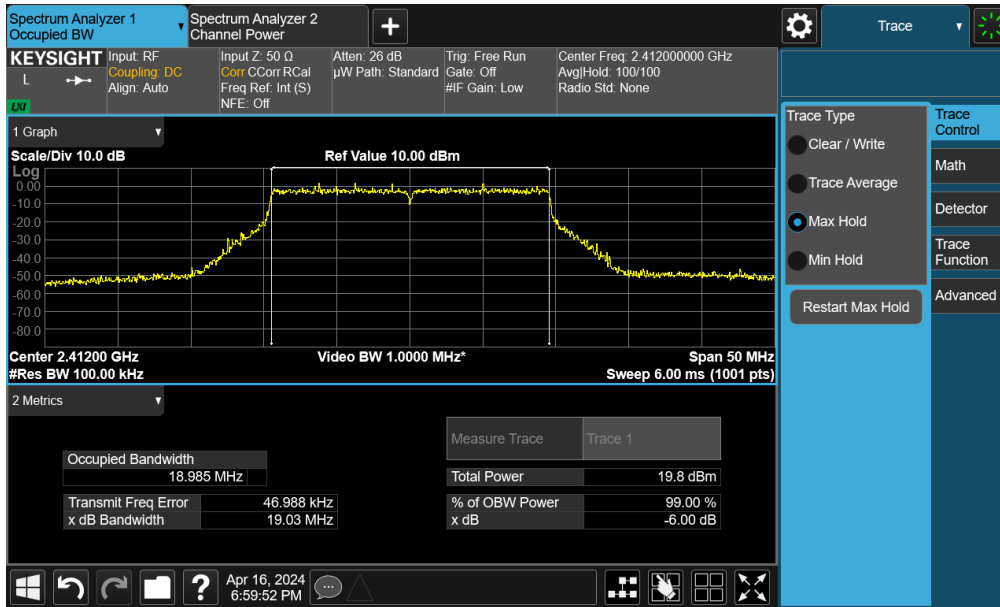
Plot 7-5. 6dB Bandwidth Plot SISO ANT2 (802.11be OFDMA – 242 Tones – Ch. 1)
