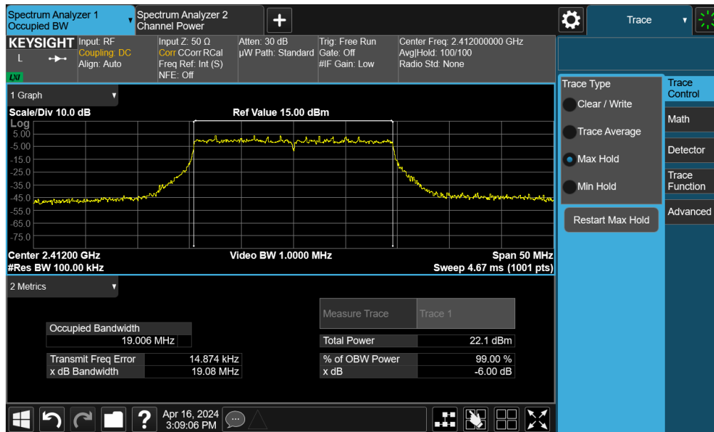
Plot 7-17. 6dB Bandwidth Plot MIMO ANT2 (802.11be OFDMA – 242Tones – Ch. 1)
