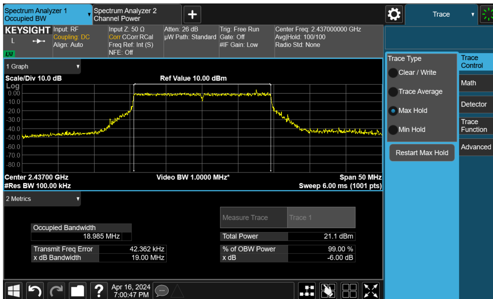
Plot 7-6. 6dB Bandwidth Plot SISO ANT2 (802.11be OFDMA – 242 Tones – Ch. 6)
