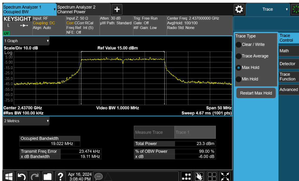
Plot 7-18. 6dB Bandwidth Plot MIMO ANT2 (802.11be OFDMA – 242Tones – Ch. 6)
