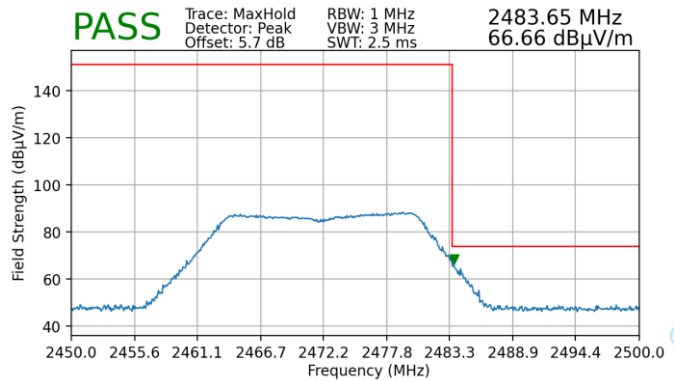
Plot 7-160. Radiated Restricted Upper Band Edge Measurement SISO ANT2 (Peak)
