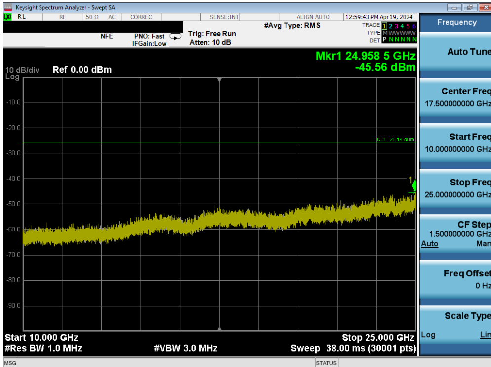
Plot 7-123. Conducted Spurious Plot SISO ANT2 (802.11b – Ch. 1)
