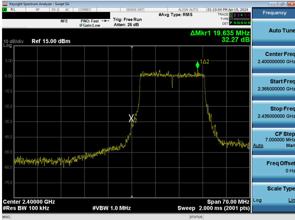
Plot 7-86. Band Edge Plot SISO ANT2 (802.11ax/be (2.4GHz) – Ch. 1)
