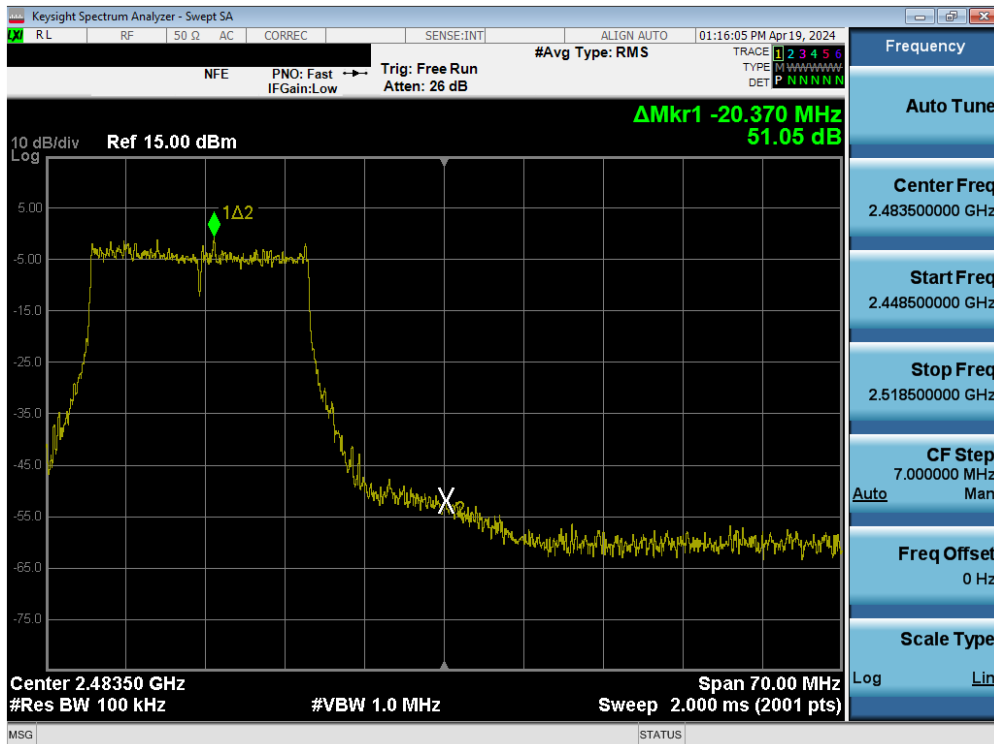
Plot 7-87. Band Edge Plot SISO ANT2 (802.11ax/be (2.4GHz) – Ch. 11)
