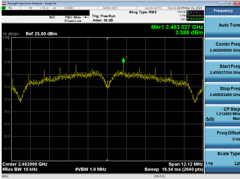
Plot 7-64. Power Spectral Density Plot MIMO ANT2 (802.11b – Ch. 11)
