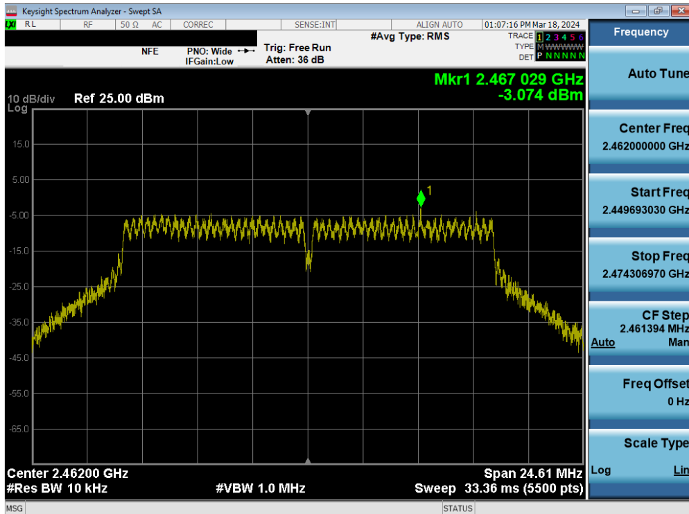
Plot 7-67. Power Spectral Density Plot MIMO ANT2 (802.11g – Ch. 11)
