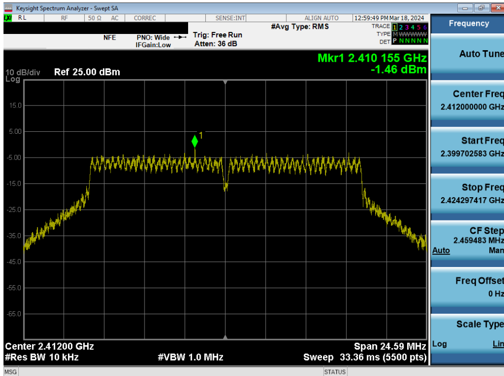
Plot 7-65. Power Spectral Density Plot MIMO ANT2 (802.11g – Ch. 1)
