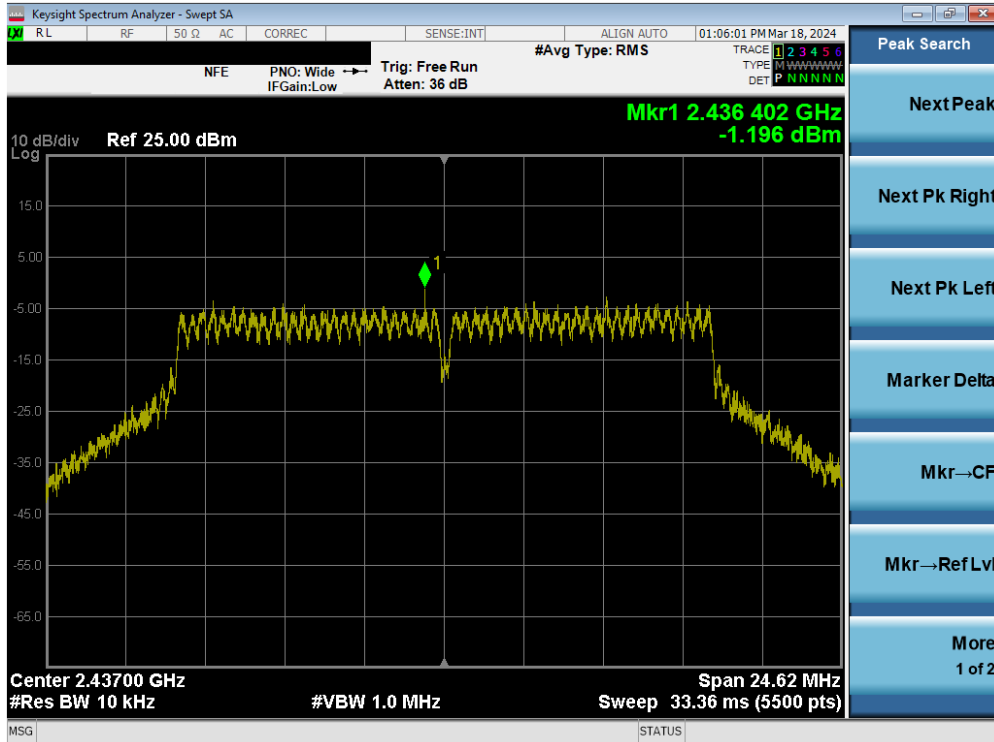
Plot 7-66. Power Spectral Density Plot MIMO ANT2 (802.11g – Ch. 6)
