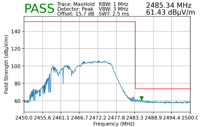
Plot 7-174. Radiated Restricted Upper Band Edge Measurement MIMO (Peak – 106+26 Tones)
