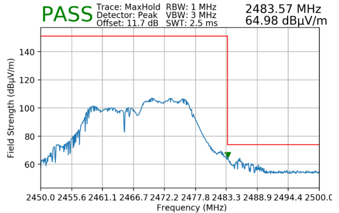
Plot 7-142. Radiated Restricted Upper Band Edge Measurement SISO ANT2 (Peak – 106 Tones)
