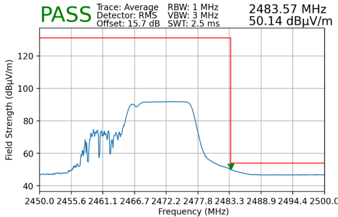
Plot 7-149. Radiated Restricted Upper Band Edge Measurement SISO ANT2 (Average – 106+26 Tones)
