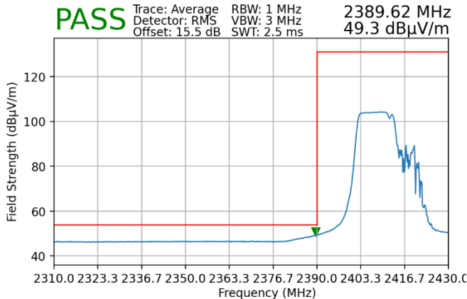
Plot 7-145. Radiated Restricted Lower Band Edge Measurement SISO ANT2 (Average – 106+26 Tones)
