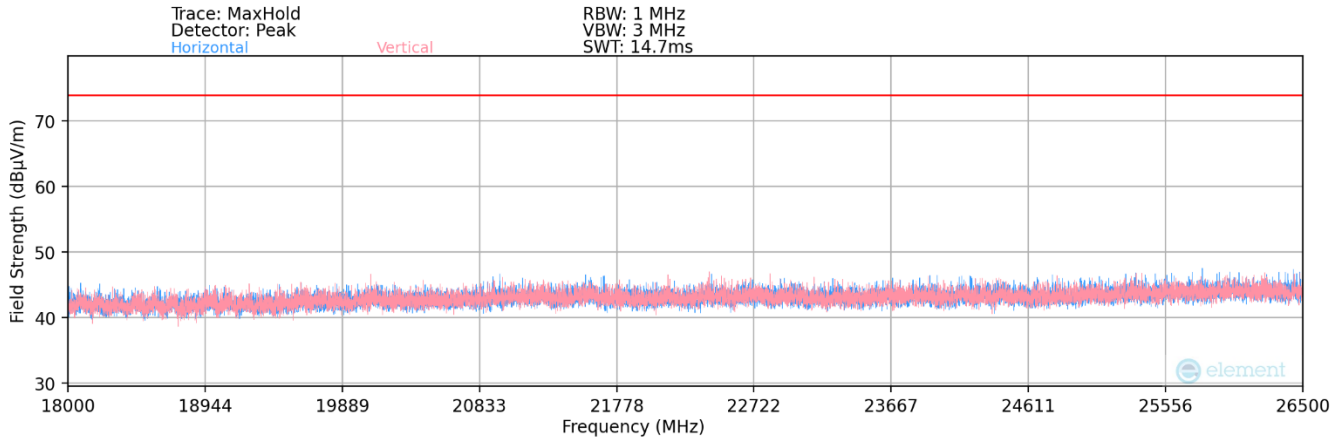
Plot 7-124. Radiated Spurious Plot above 18GHz SISO ANT2 (802.11ax/be OFDMA – 26 Tones)
