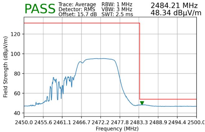
Plot 7-173. Radiated Restricted Upper Band Edge Measurement MIMO (Average – 106+26 Tones)
