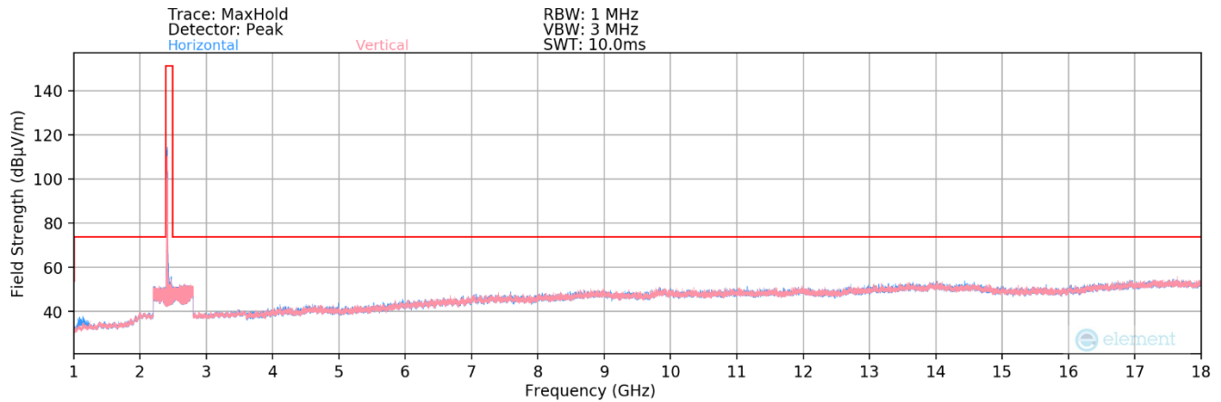
Plot 7-121. Radiated Spurious Plot above 1GHz SISO ANT2 (802.11ax/be OFDMA – 26 Tones – Ch. 1)
