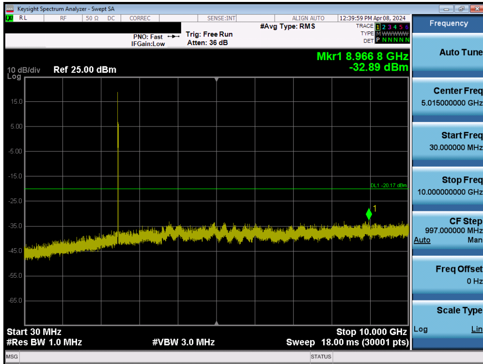
Plot 7-113. Conducted Spurious Plot MIMO ANT2 (802.11ax/be OFDMA – 26 Tones – Ch. 11)
