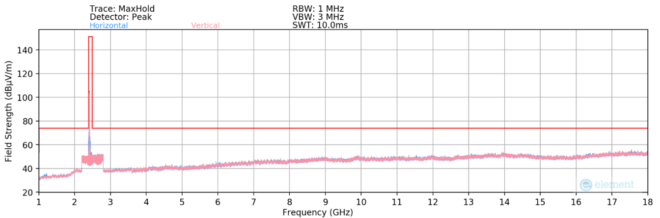
Plot 7-125. Radiated Spurious Plot above 1GHz SISO ANT2 (802.11ax/be OFDMA – 242 Tones – Ch. 1)
