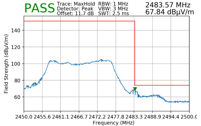
Plot 7-186. Radiated Restricted Upper Band Edge Measurement MIMO (Peak – 242 Tones)
