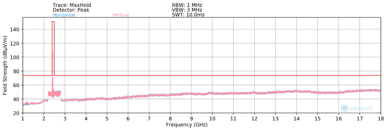
Plot 7-133. Radiated Spurious Plot above 1GHz MIMO (802.11ax/be OFDMA – 242 Tones – Ch. 1)
