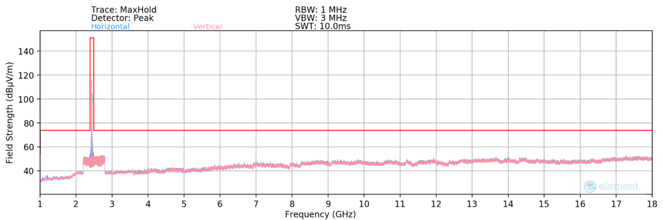
Plot 7-130. Radiated Spurious Plot above 1GHz MIMO (802.11ax/be OFDMA – 26 Tones – Ch. 6)
