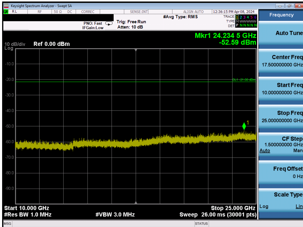
Plot 7-110. Conducted Spurious Plot MIMO ANT2 (802.11ax/be OFDMA – 26 Tones – Ch. 1)
