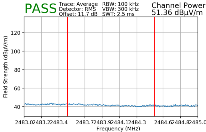
Plot 7-157. Radiated Restricted Upper Band Edge Measurement SISO ANT2 (Average – 242 Tones)
