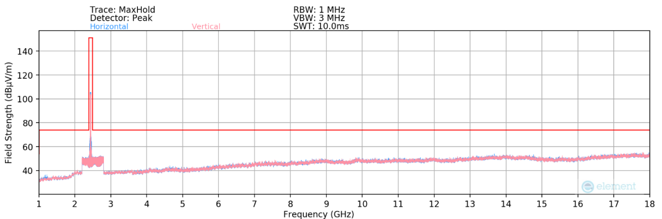
Plot 7-126. Radiated Spurious Plot above 1GHz SISO ANT2 (802.11ax/be OFDMA – 242 Tones – Ch. 6)
