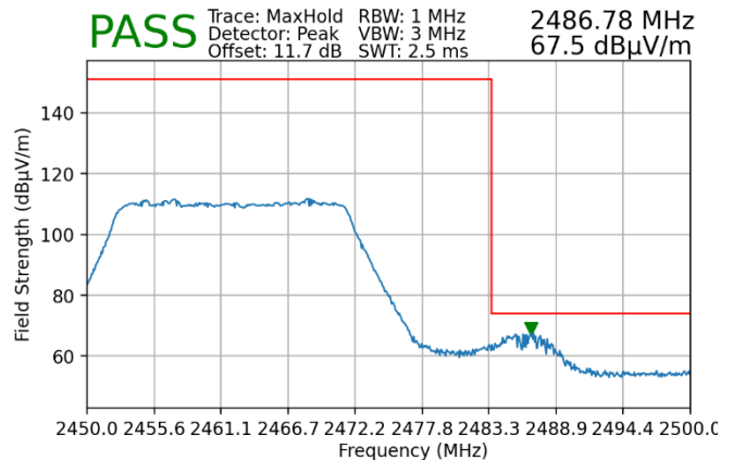
Plot 7-156. Radiated Restricted Upper Band Edge Measurement SISO ANT2 (Peak – 242 Tones)
