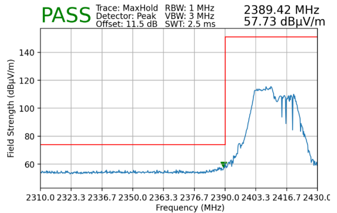
Plot 7-138. Radiated Restricted Lower Band Edge Measurement SISO ANT2 (Peak – 106 Tones)
