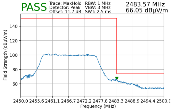
Plot 7-158. Radiated Restricted Upper Band Edge Measurement SISO ANT2 (Peak – 242 Tones)
