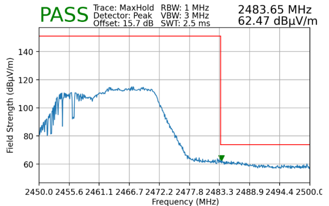
Plot 7-148. Radiated Restricted Upper Band Edge Measurement SISO ANT2 (Peak – 106+26 Tones)
