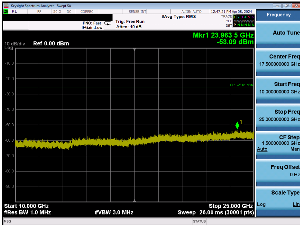
Plot 7-120. Conducted Spurious Plot MIMO ANT2 (802.11ax/be OFDMA – 242 Tones – Ch. 11)
