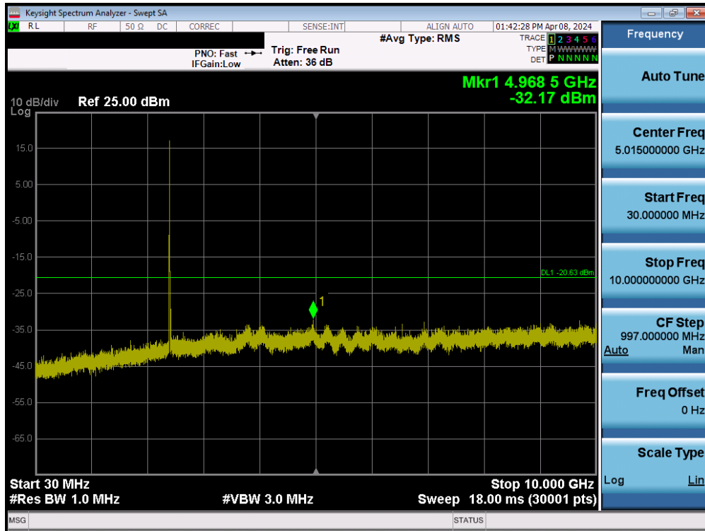
Plot 7-109. Conducted Spurious Plot MIMO ANT1 (802.11ax/be OFDMA – 26 Tones – Ch. 1)
