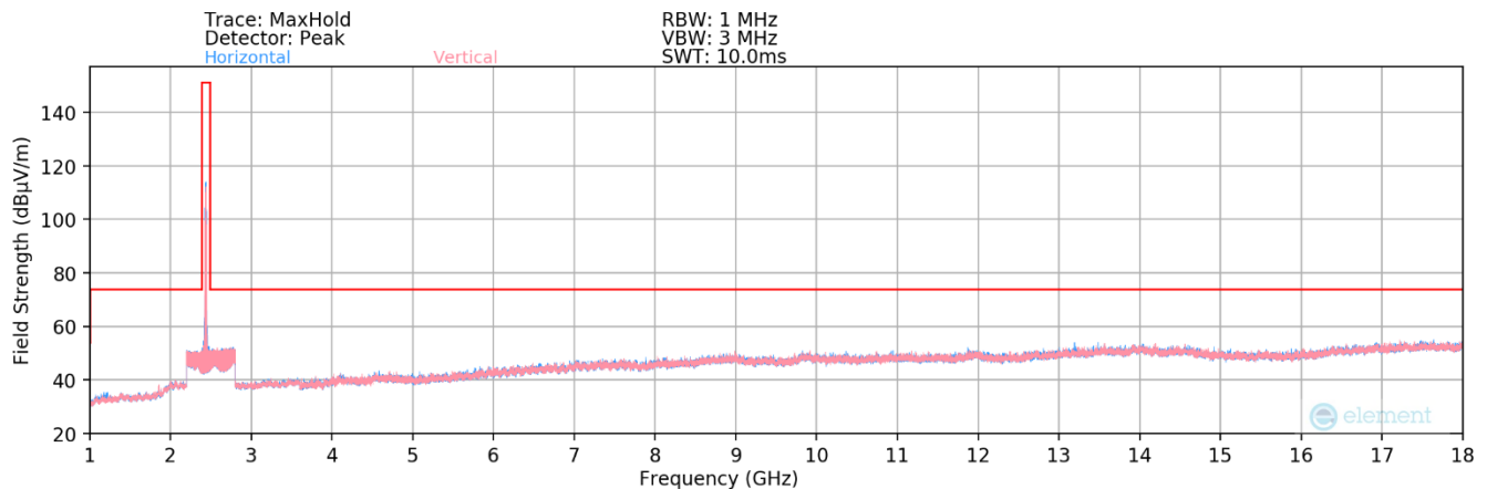
Plot 7-122. Radiated Spurious Plot above 1GHz SISO ANT2 (802.11ax/be OFDMA – 26 Tones – Ch. 6)
