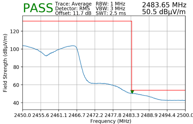
Plot 7-181. Radiated Restricted Upper Band Edge Measurement MIMO (Average – 242 Tones)
