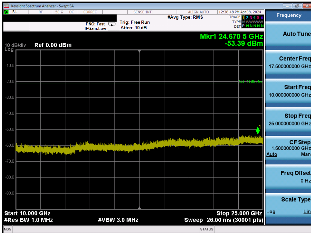
Plot 7-112. Conducted Spurious Plot MIMO ANT2 (802.11ax/be OFDMA – 26 Tones – Ch. 6)
