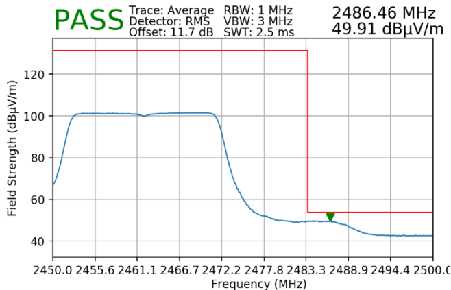
Plot 7-155. Radiated Restricted Upper Band Edge Measurement SISO ANT2 (Average – 242 Tones)
