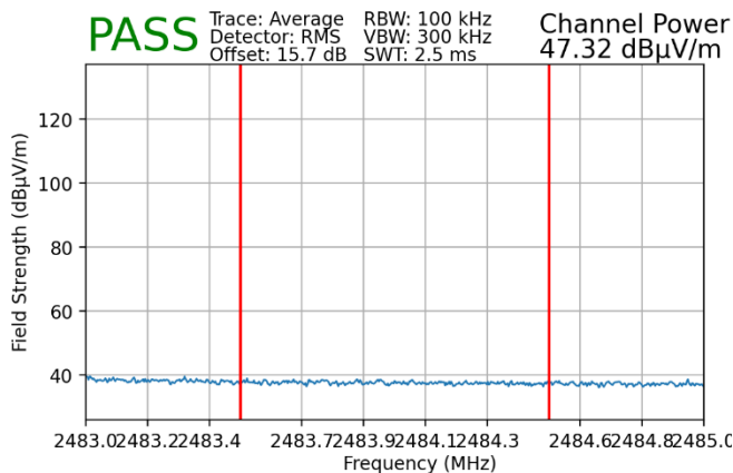
Plot 7-151. Radiated Restricted Upper Band Edge Measurement SISO ANT2 (Average – 106 Tones)
