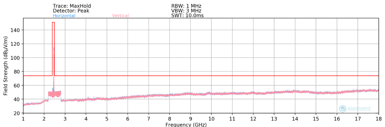
Plot 7-123. Radiated Spurious Plot above 1GHz SISO ANT2 (802.11ax/be OFDMA – 26 Tones – Ch. 11)
