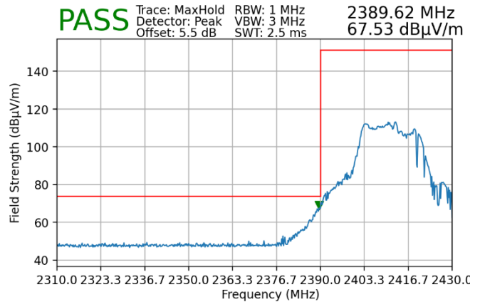
Plot 7-170. Radiated Restricted Lower Band Edge Measurement MIMO (Peak – 106+26 Tones)
