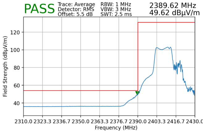
Plot 7-169. Radiated Restricted Lower Band Edge Measurement MIMO (Average – 106+26 Tones)
