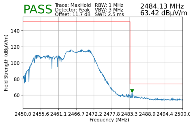
Plot 7-140. Radiated Restricted Upper Band Edge Measurement SISO ANT2 (Peak – 106 Tones)
