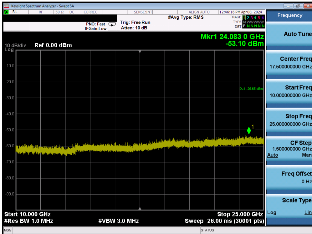
Plot 7-118. Conducted Spurious Plot MIMO ANT2 (802.11ax/be OFDMA – 242 Tones – Ch. 6)
