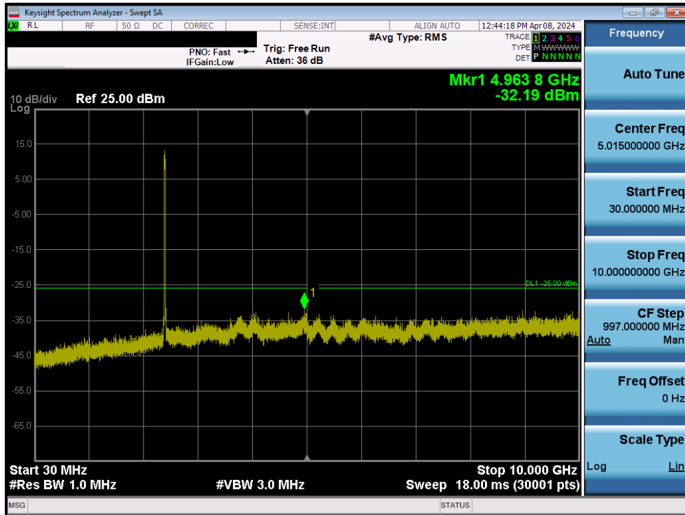
Plot 7-115. Conducted Spurious Plot MIMO ANT2 (802.11ax/be OFDMA – 242 Tones – Ch. 1)
