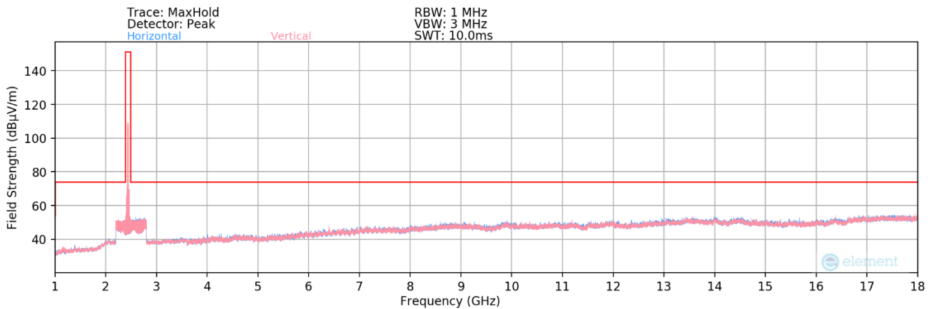
Plot 7-134. Radiated Spurious Plot above 1GHz MIMO (802.11ax/be OFDMA – 242 Tones – Ch. 6)
