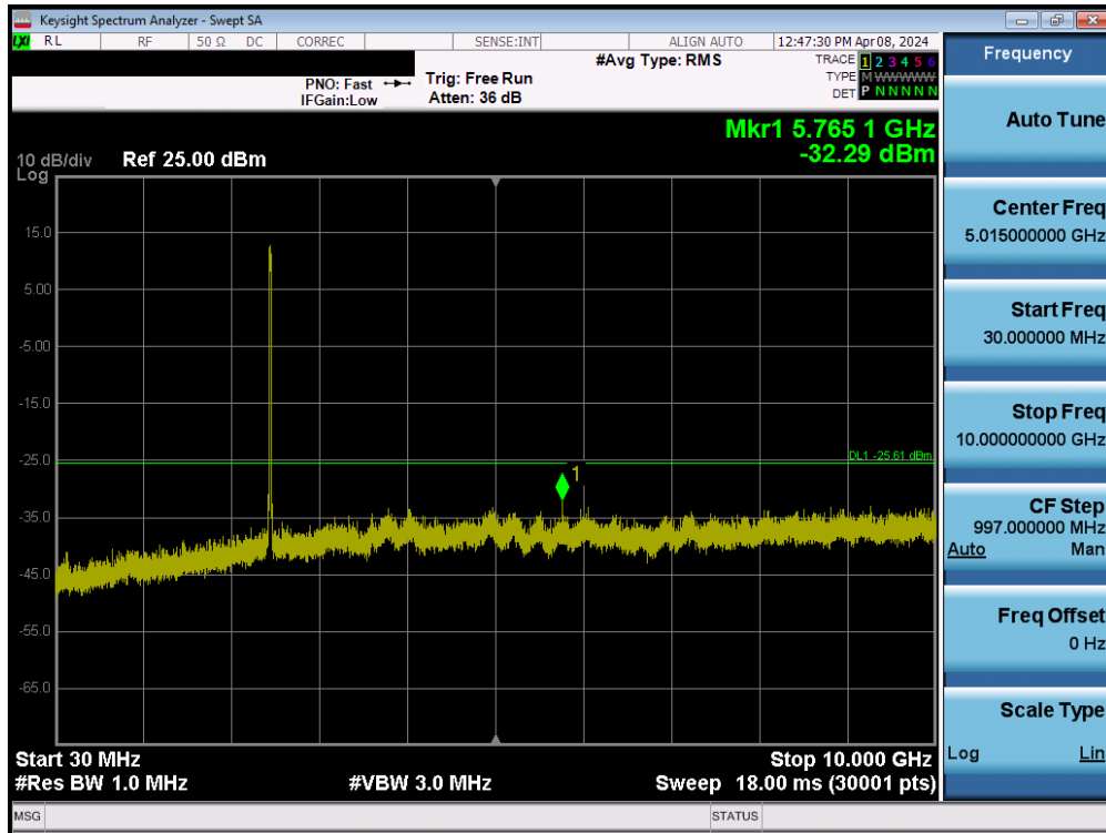
Plot 7-119. Conducted Spurious Plot MIMO ANT2 (802.11ax/be OFDMA – 242 Tones – Ch. 11)
