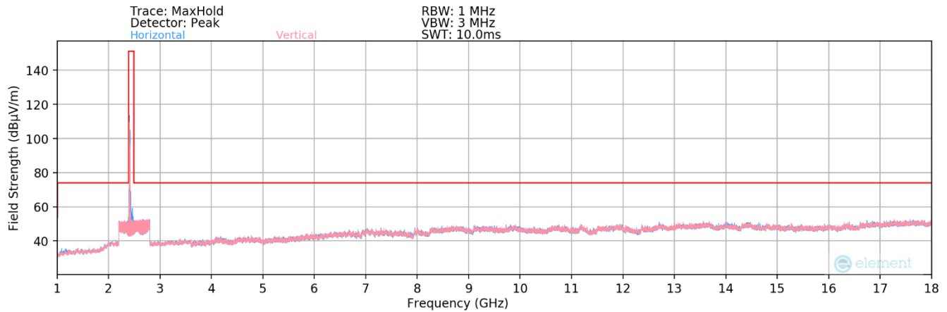
Plot 7-129. Radiated Spurious Plot above 1GHz MIMO (802.11ax/be OFDMA – 26 Tones – Ch. 1)
