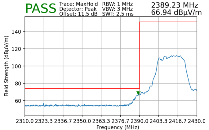
Plot 7-178. Radiated Restricted Lower Band Edge Measurement MIMO (Peak – 242 Tones)
