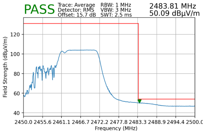
Plot 7-147. Radiated Restricted Upper Band Edge Measurement SISO ANT2 (Average – 106+26 Tones)
