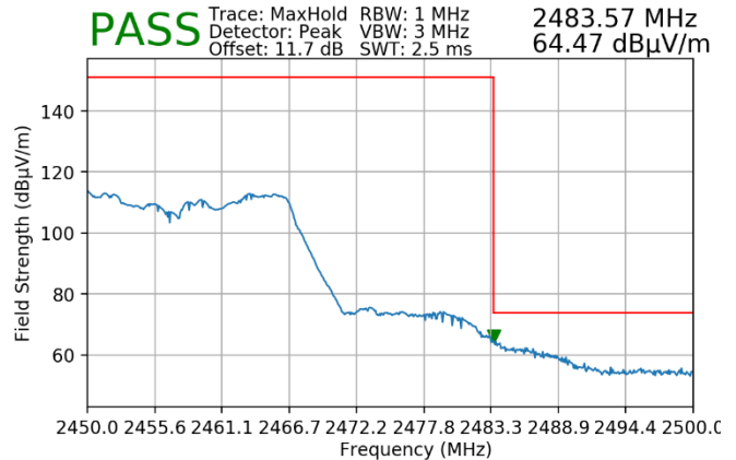
Plot 7-182. Radiated Restricted Upper Band Edge Measurement MIMO (Peak – 242 Tones)
