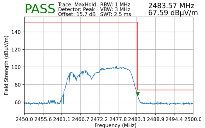
Plot 7-176. Radiated Restricted Upper Band Edge Measurement MIMO (Peak – 106+26 Tones)
