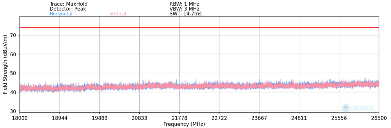
Plot 7-132. Radiated Spurious Plot above 18GHz MIMO (802.11ax/be OFDMA – 26 Tones)
