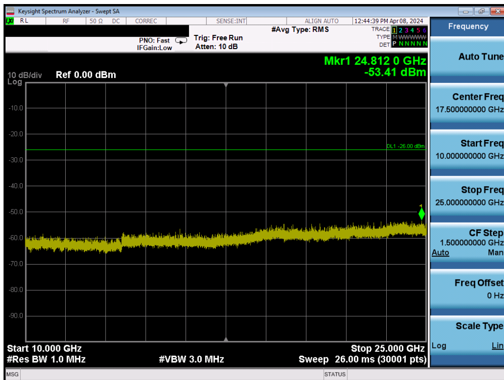
Plot 7-116. Conducted Spurious Plot MIMO ANT2 (802.11ax/be OFDMA – 242 Tones – Ch. 1)
