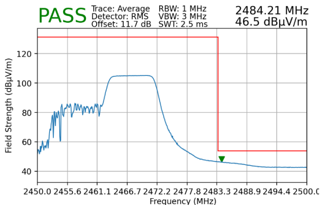
Plot 7-139. Radiated Restricted Upper Band Edge Measurement SISO ANT2 (Average – 106 Tones)
