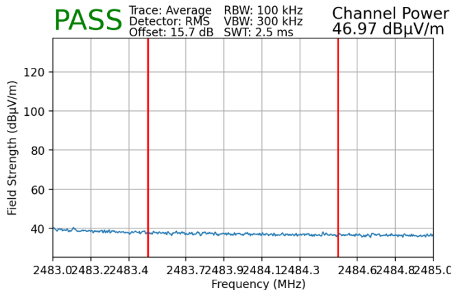
Plot 7-175. Radiated Restricted Upper Band Edge Measurement MIMO (Average – 106+26 Tones)
