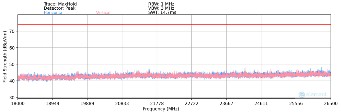
Plot 7-128. Radiated Spurious Plot above 18GHz SISO ANT2 (802.11ax/be OFDMA – 242 Tones)
