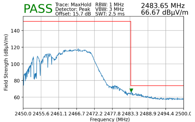
Plot 7-172. Radiated Restricted Upper Band Edge Measurement MIMO (Peak – 106+26 Tones)
