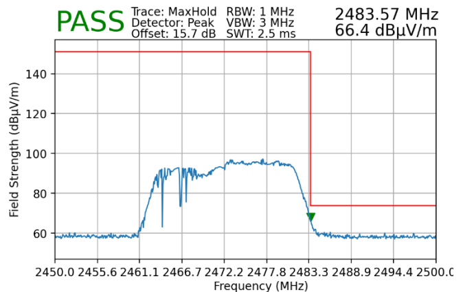
Plot 7-152. Radiated Restricted Upper Band Edge Measurement SISO ANT2 (Peak – 106 Tones)
