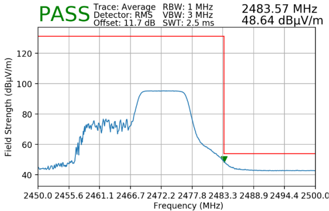
Plot 7-141. Radiated Restricted Upper Band Edge Measurement SISO ANT2 (Average – 106 Tones)
