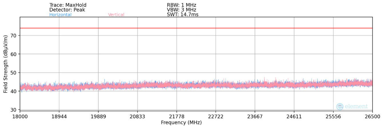
Plot 7-136. Radiated Spurious Plot above 18GHz MIMO (802.11ax/be OFDMA – 242 Tones)
