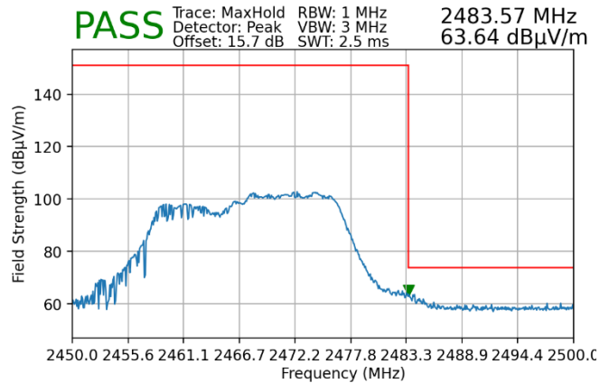
Plot 7-150. Radiated Restricted Upper Band Edge Measurement SISO ANT2 (Peak – 106+26 Tones)
