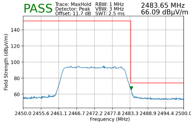
Plot 7-160. Radiated Restricted Upper Band Edge Measurement SISO ANT2 (Peak – 242 Tones)
