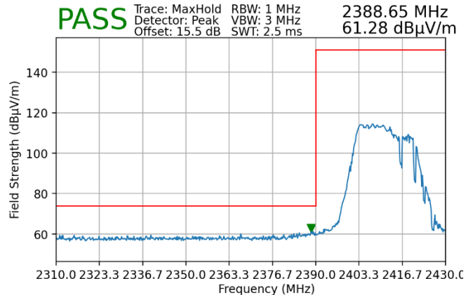
Plot 7-146. Radiated Restricted Lower Band Edge Measurement SISO ANT2 (Peak – 106+26 Tones)
