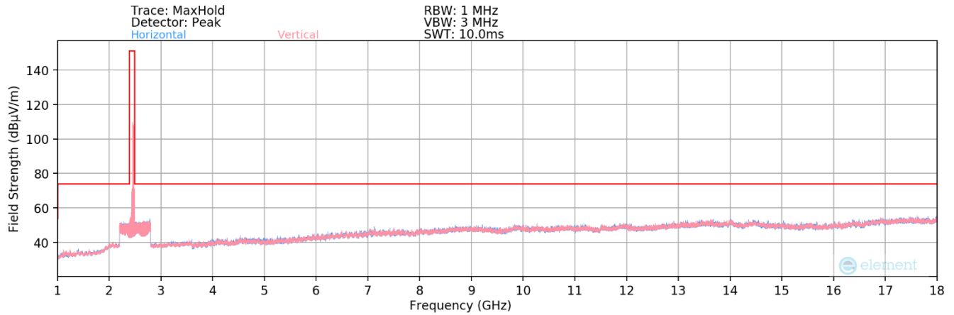
Plot 7-135. Radiated Spurious Plot above 1GHz MIMO (802.11ax/be OFDMA – 242 Tones – Ch. 11)
