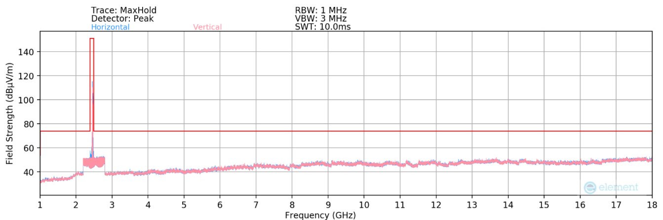
Plot 7-131. Radiated Spurious Plot above 1GHz MIMO (802.11ax/be OFDMA – 26 Tones – Ch. 11)
