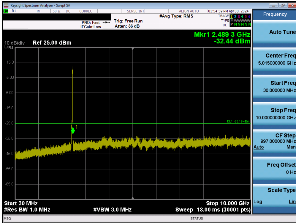
Plot 7-107. Conducted Spurious Plot MIMO ANT1 (802.11ax/be OFDMA – 242 Tones – Ch. 11)
