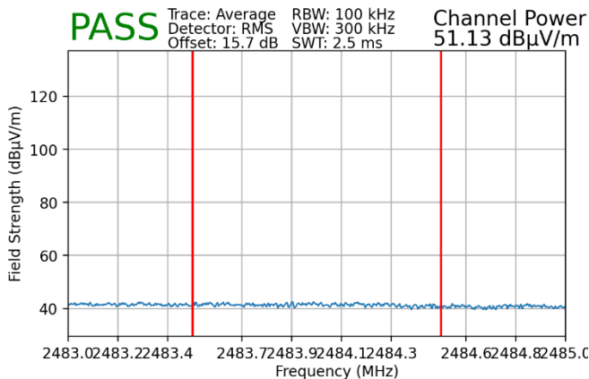
Plot 7-171. Radiated Restricted Upper Band Edge Measurement MIMO (Average – 106+26 Tones)
