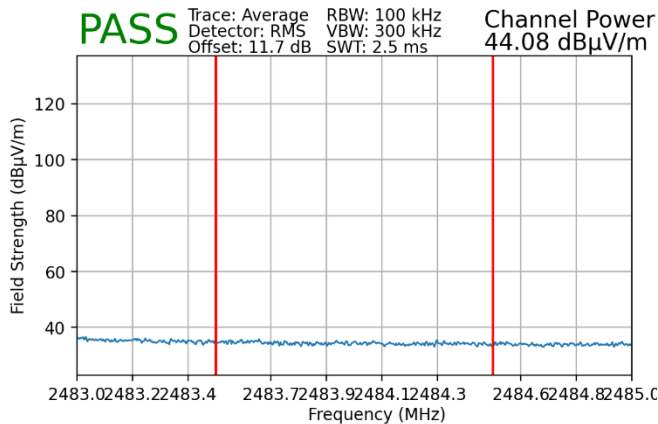
Plot 7-159. Radiated Restricted Upper Band Edge Measurement SISO ANT2 (Average – 242 Tones)
