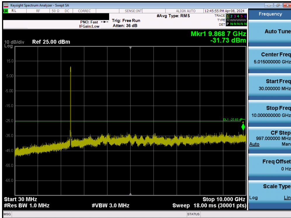
Plot 7-117. Conducted Spurious Plot MIMO ANT2 (802.11ax/be OFDMA – 242 Tones – Ch. 6)
