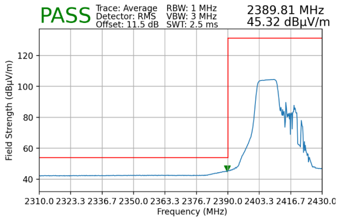
Plot 7-137. Radiated Restricted Lower Band Edge Measurement SISO ANT2 (Average – 106 Tones)
