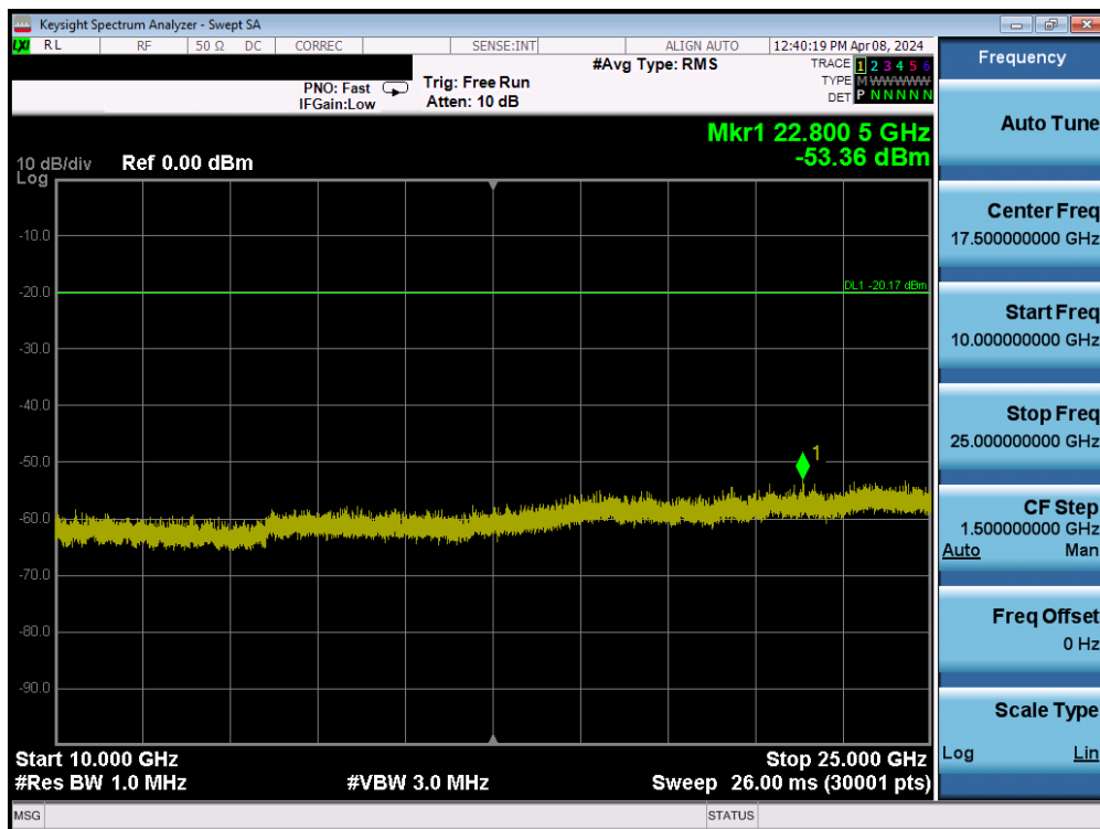
Plot 7-114. Conducted Spurious Plot MIMO ANT2 (802.11ax/be OFDMA – 26 Tones – Ch. 11)
