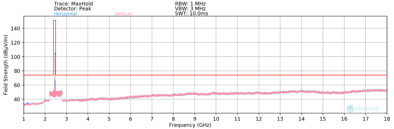
Plot 7-127. Radiated Spurious Plot above 1GHz SISO ANT2 (802.11ax/be OFDMA – 242 Tones – Ch. 11)
