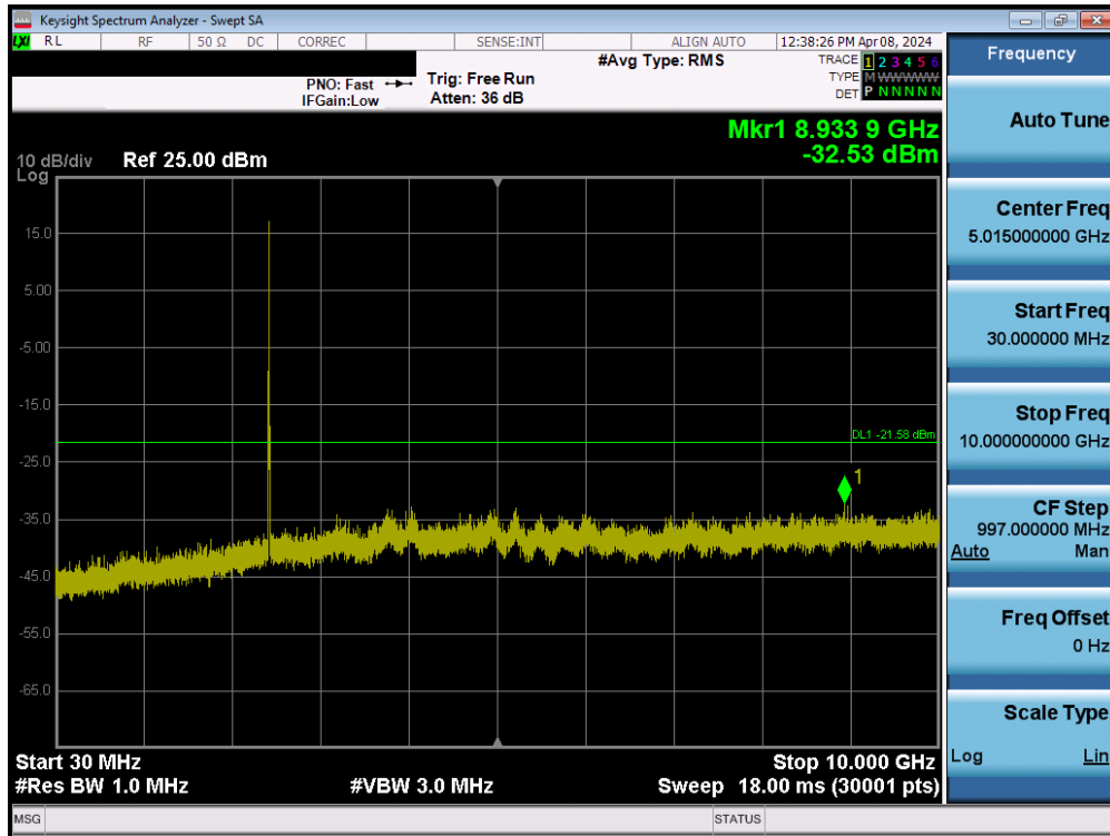
Plot 7-111. Conducted Spurious Plot MIMO ANT2 (802.11ax/be OFDMA – 26 Tones – Ch. 6)
