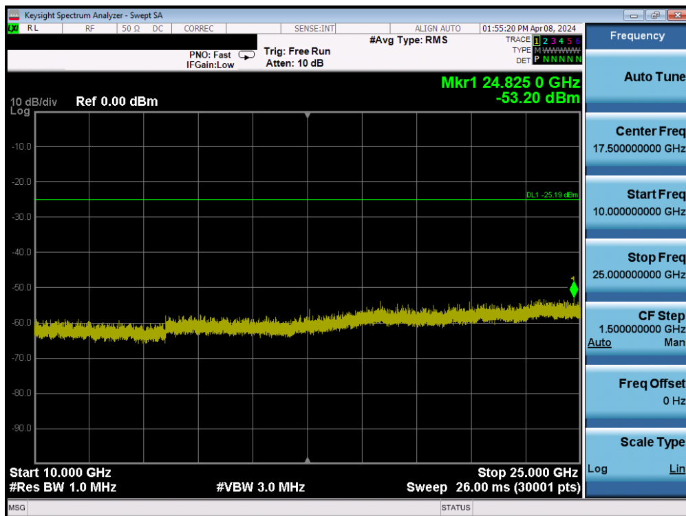
Plot 7-108. Conducted Spurious Plot MIMO ANT1 (802.11ax/be OFDMA – 242 Tones – Ch. 11)
