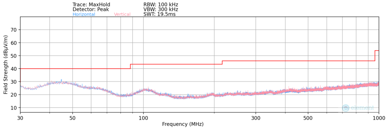
Plot 7-165. Radiated Spurious Plot below 1GHz (2.4GHz -6GHz)
