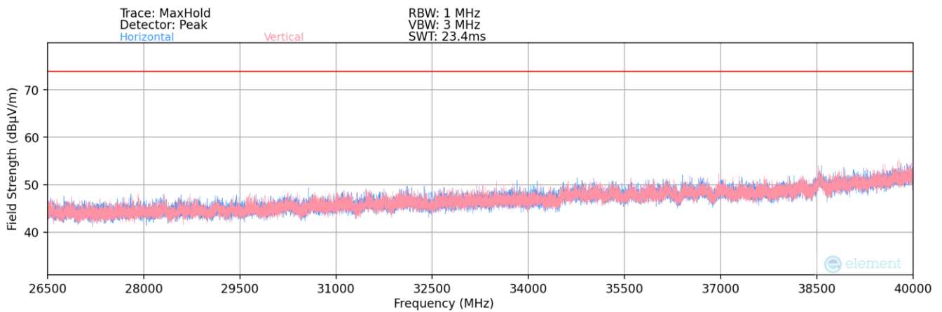
Plot 7-164. Radiated Spurious Plot above 26.5GHz (2.4GHz – 5GHz)
