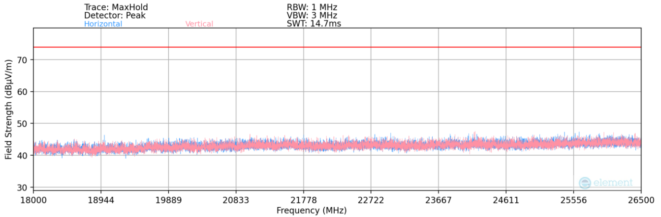
Plot 7-167. Radiated Spurious Plot 18GHz – 26.5GHz (2.4GHz –6GHz)
