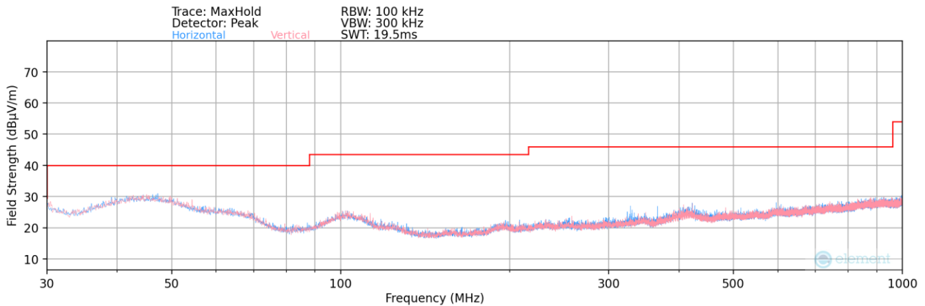
Plot 7-161. Radiated Spurious Plot below 1GHz (2.4GHz – 5GHz)
