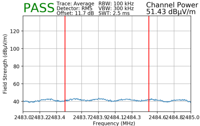
Plot 7-189. Radiated Restricted Upper Band Edge Measurement MIMO (Average)
