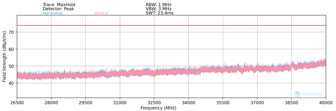
Plot 7-168. Radiated Spurious Plot above 26.5GHz (2.4GHz –6GHz)
