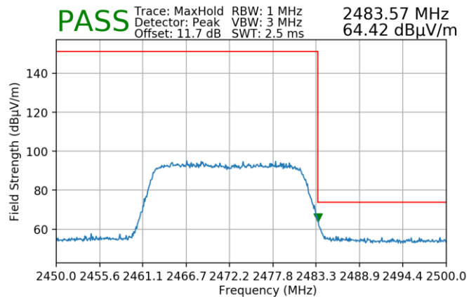
Plot 7-180. Radiated Restricted Upper Band Edge Measurement SISO ANT2 (Peak)
