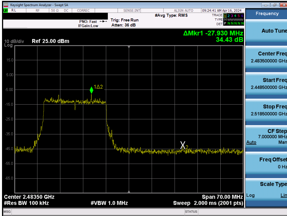
Plot 7-131. Band Edge Plot MIMO ANT2 (802.11ax/be (2.4GHz) – Ch. 12)
