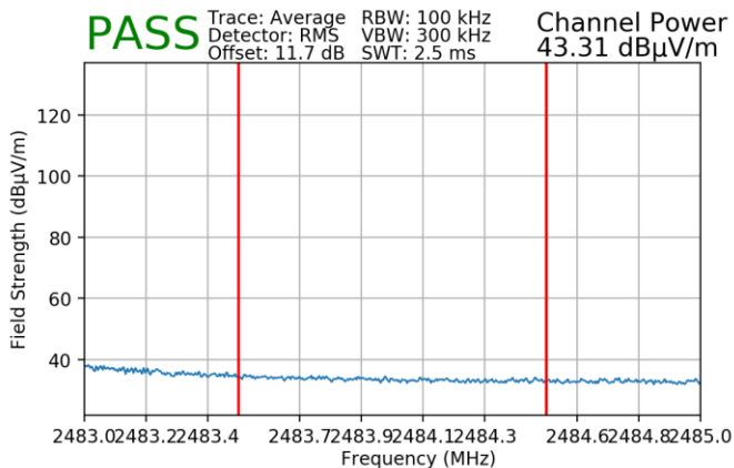
Plot 7-191. Radiated Restricted Upper Band Edge Measurement MIMO (Average)
