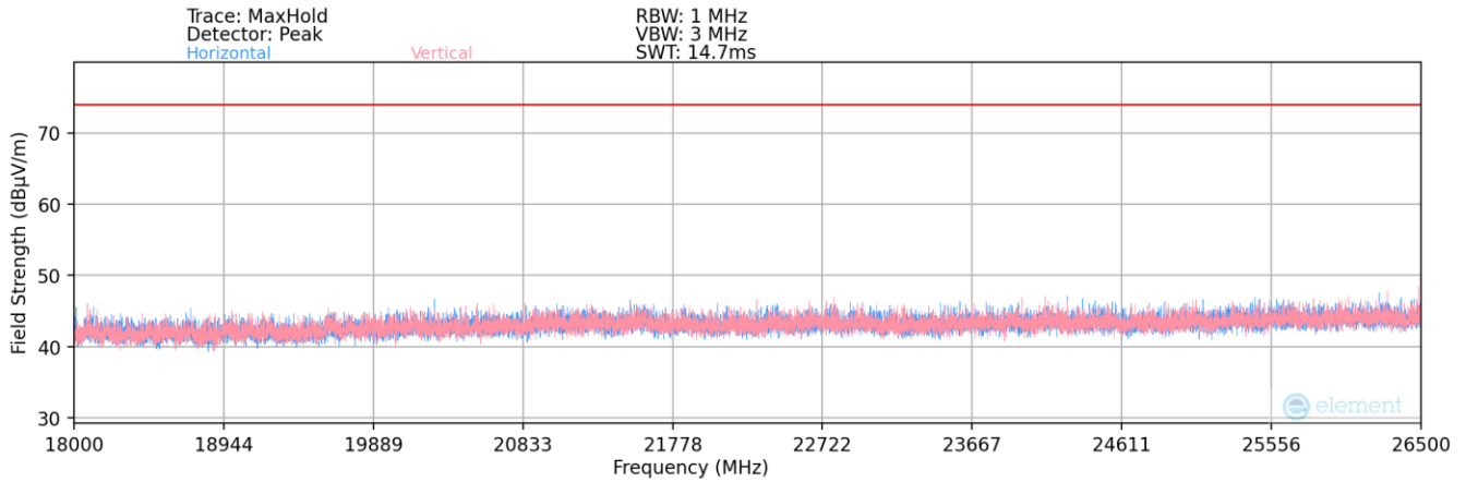
Plot 7-163. Radiated Spurious Plot 18GHz – 26.5GHz (2.4GHz – 5GHz)
