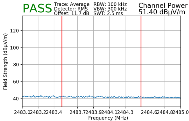
Plot 7-177. Radiated Restricted Upper Band Edge Measurement SISO ANT2 (Average)
