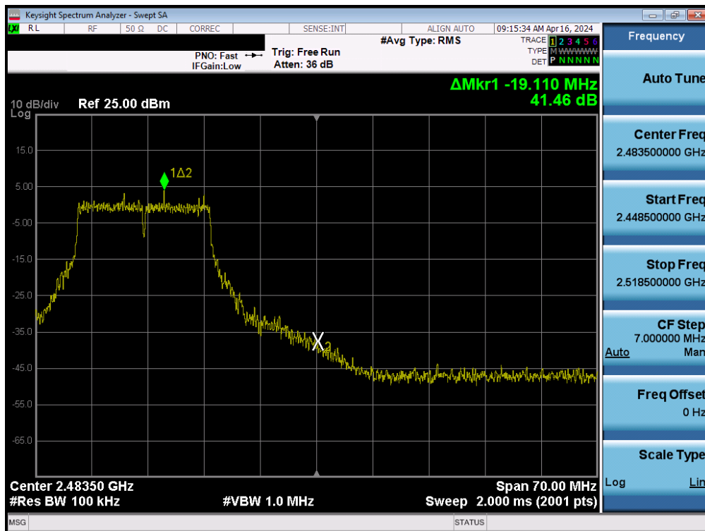
Plot 7-120. Band Edge Plot MIMO ANT2 (802.11g – Ch. 11)
