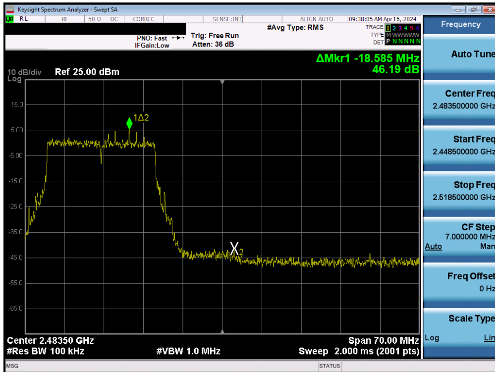
Plot 7-130. Band Edge Plot MIMO ANT2 (802.11ax/be (2.4GHz) – Ch. 11)
