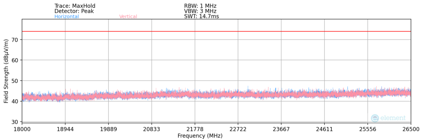
Plot 7-160. Radiated Spurious Plot above 18GHz MIMO
