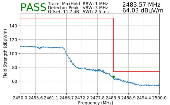
Plot 7-186. Radiated Restricted Upper Band Edge Measurement MIMO (Peak)
