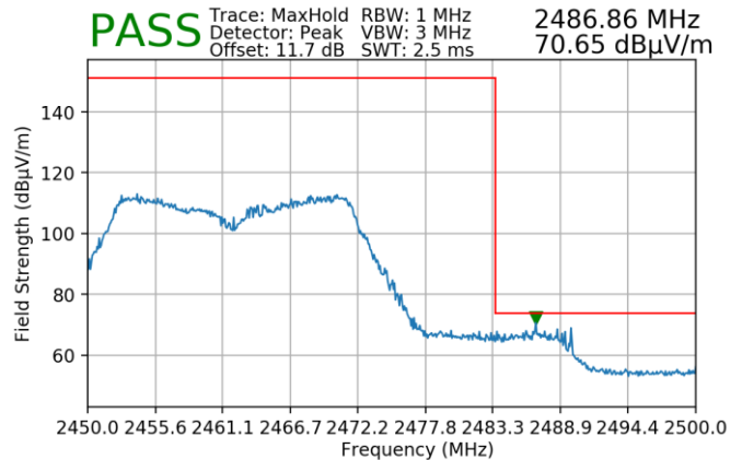
Plot 7-188. Radiated Restricted Upper Band Edge Measurement MIMO (Peak)
