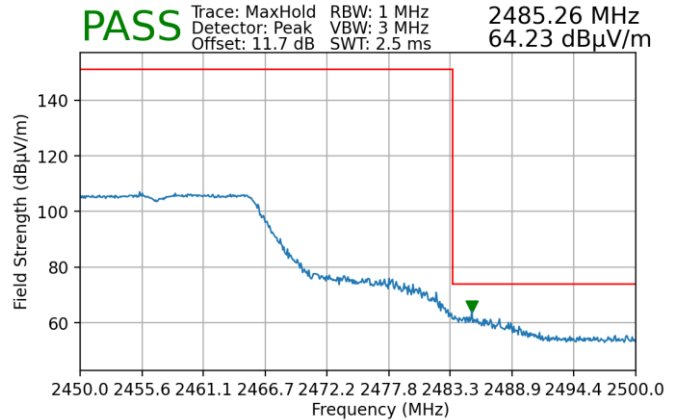
Plot 7-174. Radiated Restricted Upper Band Edge Measurement SISO ANT2 (Peak)
