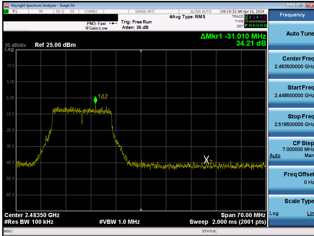
Plot 7-121. Band Edge Plot MIMO ANT2 (802.11g – Ch. 12)
