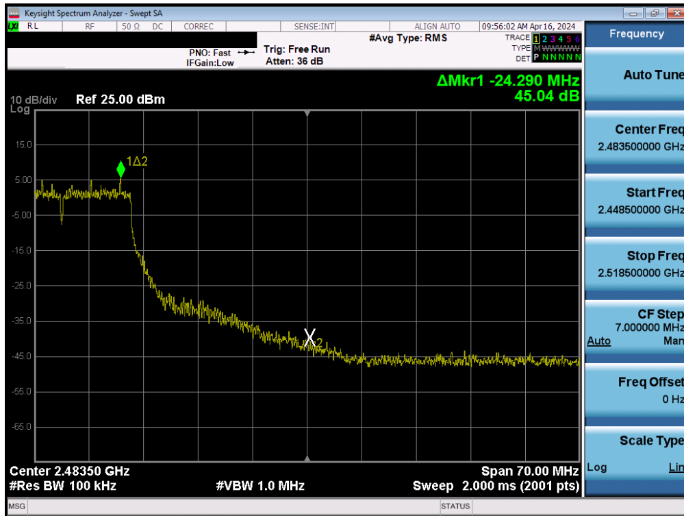
Plot 7-124. Band Edge Plot MIMO ANT2 (802.11n (2.4GHz) – Ch. 9)
