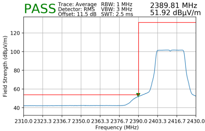
Plot 7-169. Radiated Restricted Lower Band Edge Measurement SISO ANT2 (Average)
