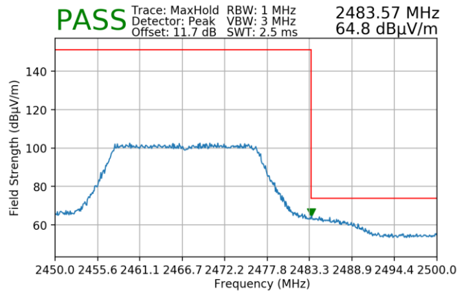
Plot 7-178. Radiated Restricted Upper Band Edge Measurement SISO ANT2 (Peak)
