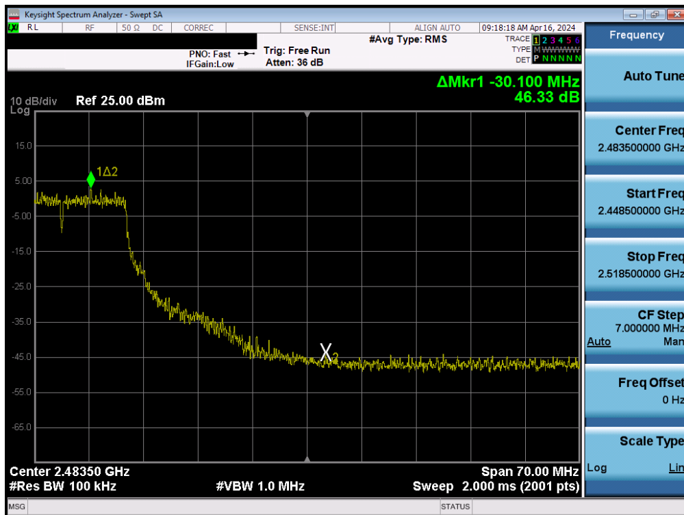
Plot 7-118. Band Edge Plot MIMO ANT2 (802.11g - Ch. 9)
