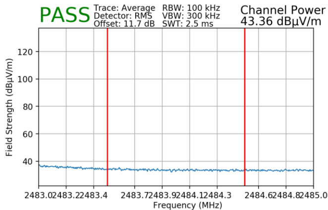
Plot 7-179. Radiated Restricted Upper Band Edge Measurement SISO ANT2 (Average)
