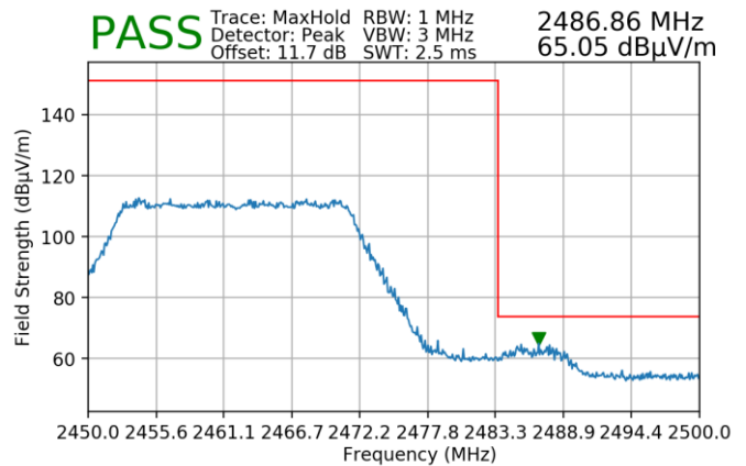
Plot 7-176. Radiated Restricted Upper Band Edge Measurement SISO ANT2 (Peak)
