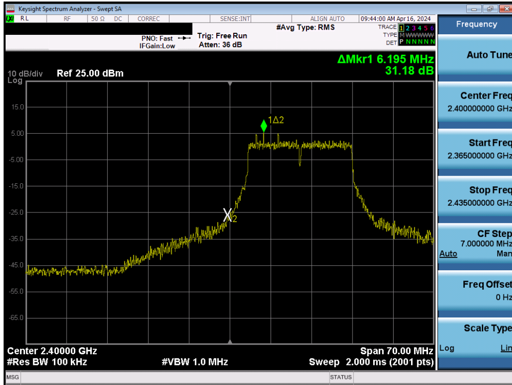
Plot 7-123. Band Edge Plot MIMO ANT2 (802.11n (2.4GHz) – Ch. 1)
