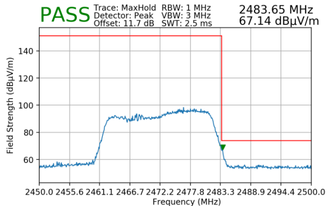
Plot 7-192. Radiated Restricted Upper Band Edge Measurement MIMO (Peak)
