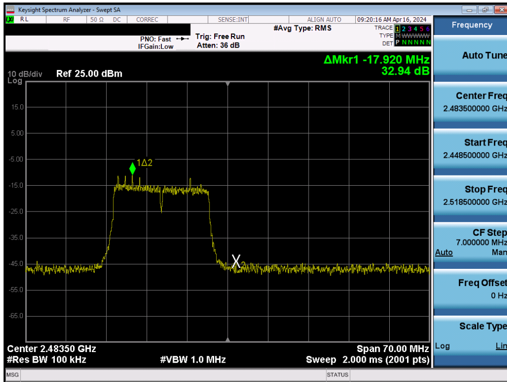
Plot 7-122. Band Edge Plot MIMO ANT2 (802.11g – Ch. 13)
