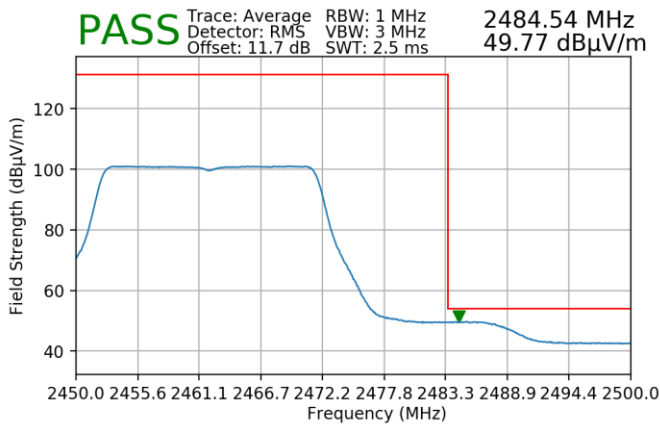
Plot 7-175. Radiated Restricted Upper Band Edge Measurement SISO ANT2 (Average)
