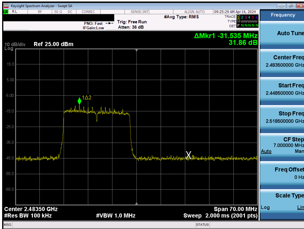
Plot 7-132. Band Edge Plot MIMO ANT2 (802.11ax/be (2.4GHz) – Ch. 13)
