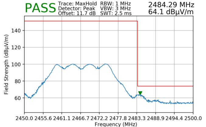
Plot 7-190. Radiated Restricted Upper Band Edge Measurement MIMO (Peak)
