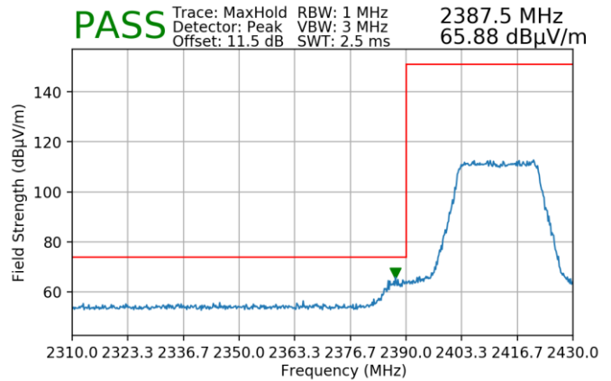
Plot 7-170. Radiated Restricted Lower Band Edge Measurement SISO ANT2 (Peak)
