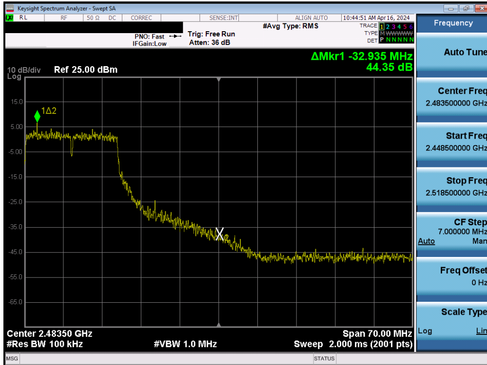
Plot 7-99. Band Edge Plot MIMO ANT1 (802.11g – Ch. 10)
