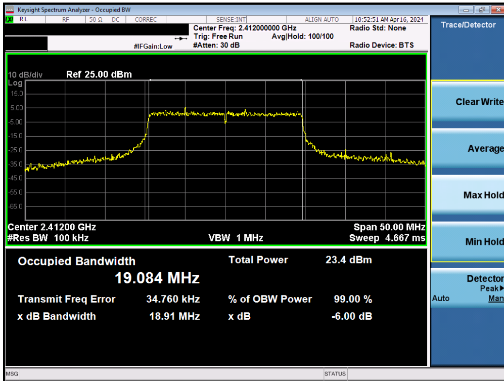
Plot 7-22. 6dB Bandwidth Plot MIMO ANT1 (802.11ax/be (2.4GHz) – Ch. 1)
