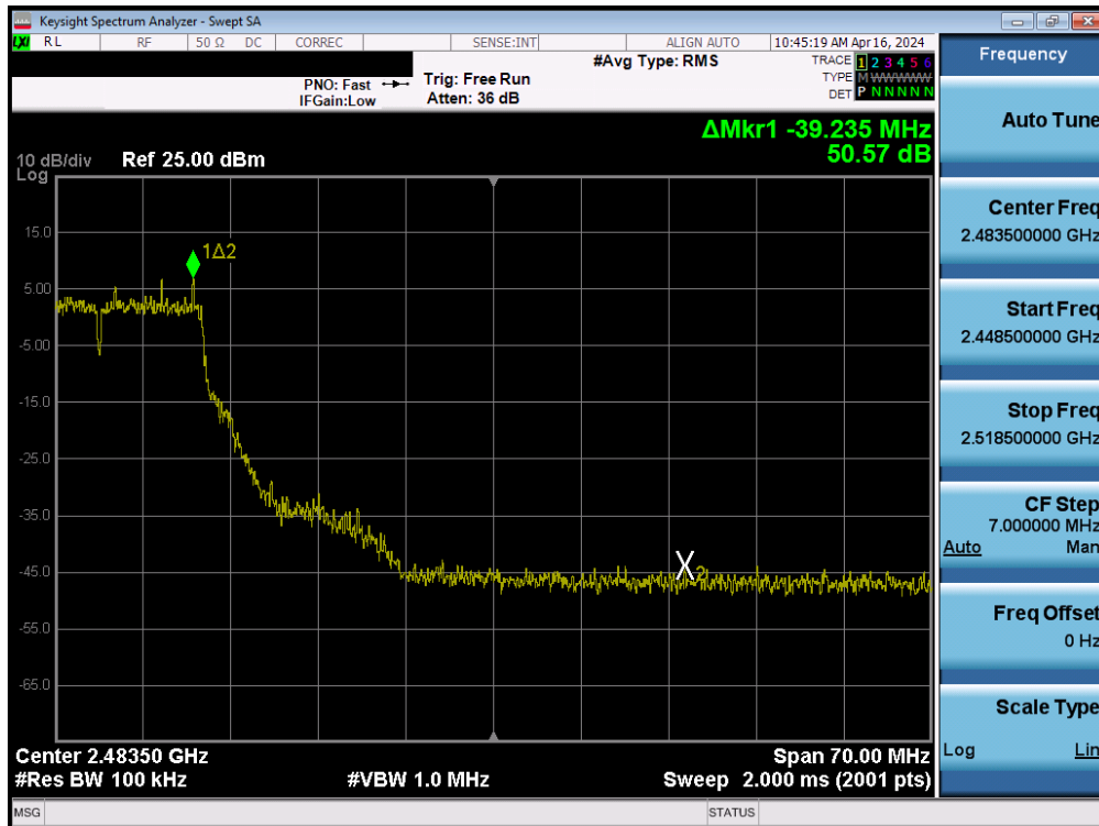
Plot 7-98. Band Edge Plot MIMO ANT1 (802.11g - Ch. 9)
