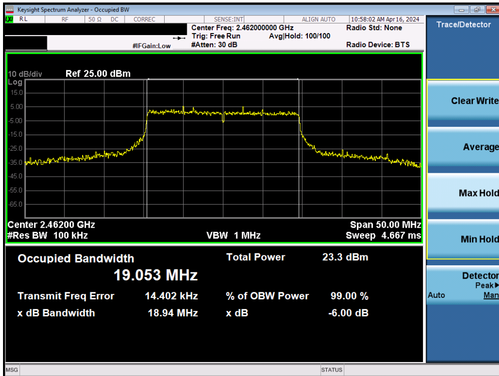
Plot 7-24. 6dB Bandwidth Plot MIMO ANT1 (802.11ax/be (2.4GHz) – Ch. 11)
