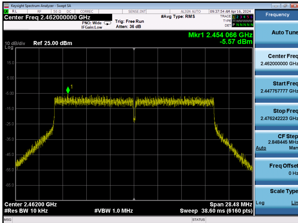
Plot 7-72. Power Spectral Density Plot MIMO ANT2 (802.11ax/be (2.4GHz) – Ch. 11)
