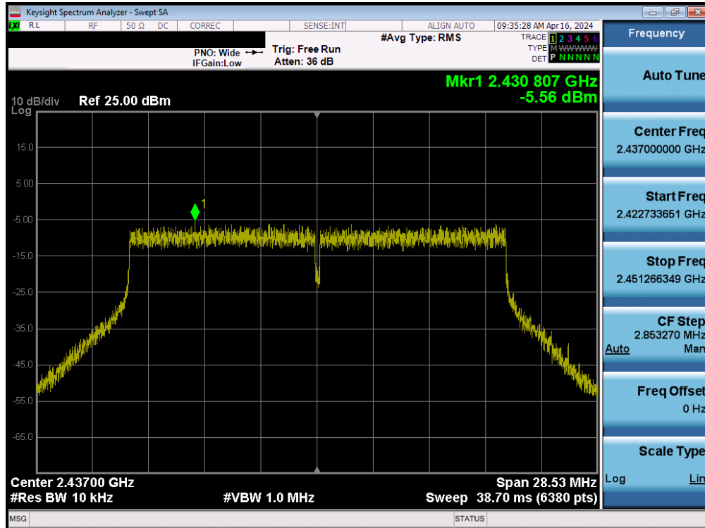
Plot 7-71. Power Spectral Density Plot MIMO ANT2 (802.11ax/be (2.4GHz) – Ch. 6)
