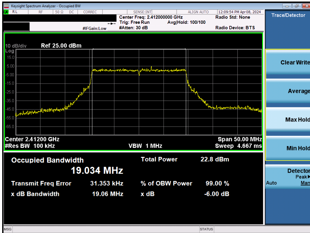
Plot 7-10. 6dB Bandwidth Plot SISO ANT2 (802.11ax/be (2.4GHz) – Ch. 1)
