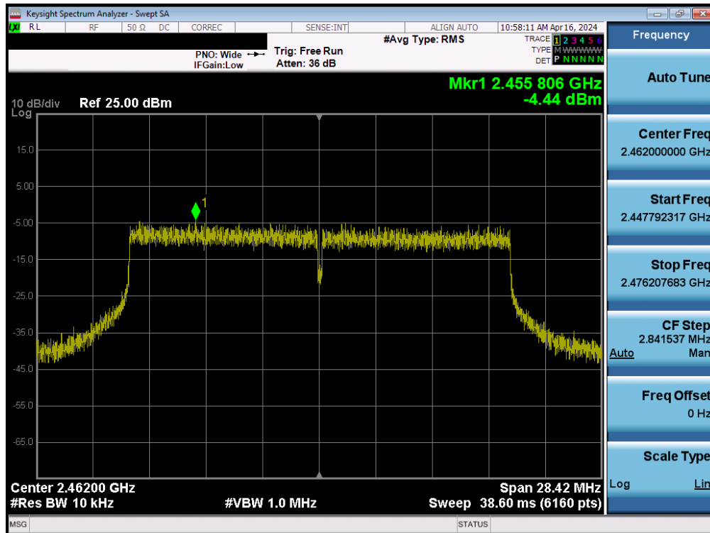
Plot 7-60. Power Spectral Density Plot MIMO ANT1 (802.11ax/be (2.4GHz) – Ch. 11)
