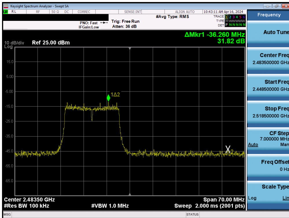
Plot 7-102. Band Edge Plot MIMO ANT1 (802.11g – Ch. 13)
