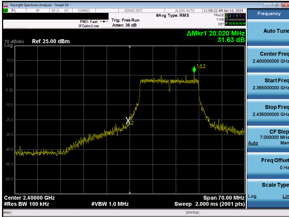
Plot 7-103. Band Edge Plot MIMO ANT1 (802.11n (2.4GHz) – Ch. 1)
