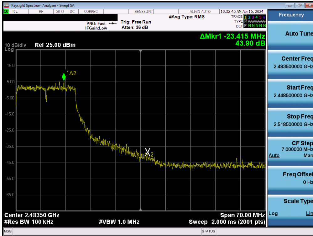
Plot 7-79. Band Edge Plot SISO ANT2 (802.11g – Ch. 10)
