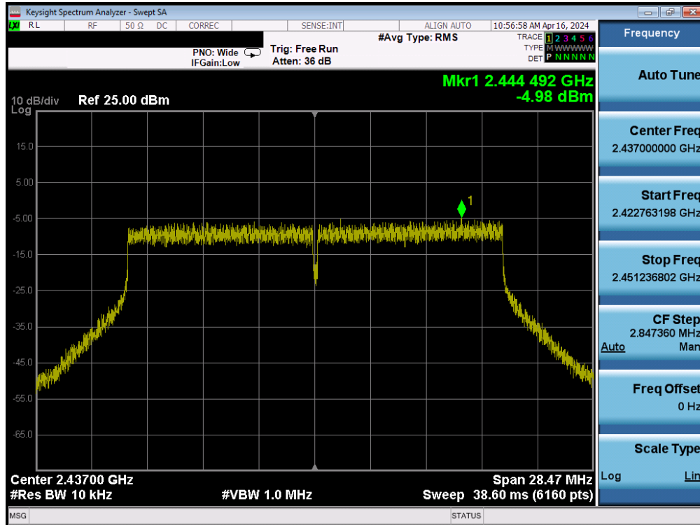
Plot 7-59. Power Spectral Density Plot MIMO ANT1 (802.11ax/be (2.4GHz) – Ch. 6)
