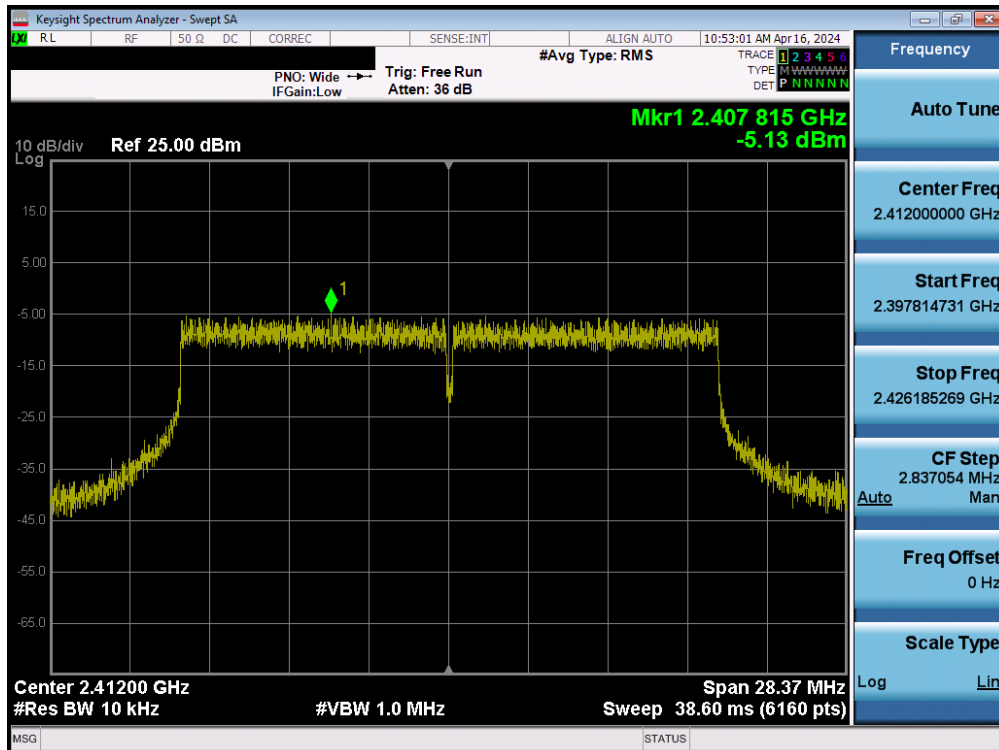
Plot 7-58. Power Spectral Density Plot MIMO ANT1 (802.11ax/be (2.4GHz) – Ch. 1)
