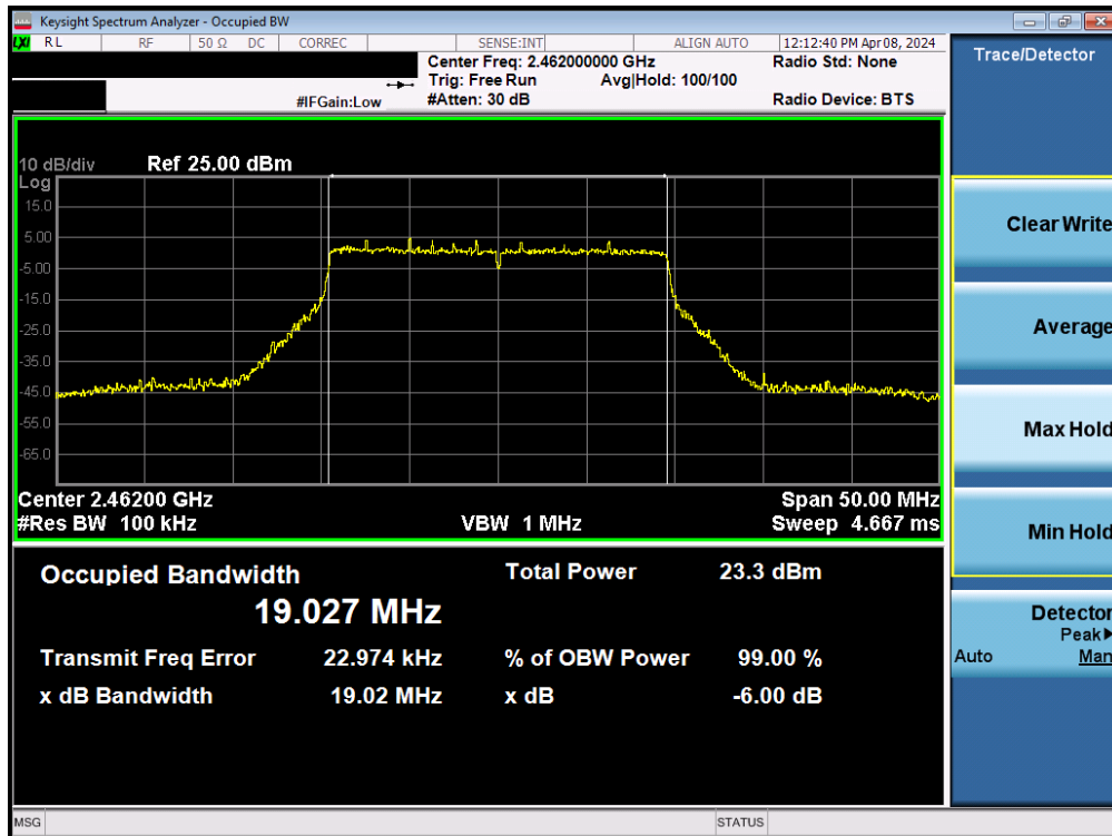
Plot 7-12. 6dB Bandwidth Plot SISO ANT2 (802.11ax/be (2.4GHz) – Ch. 11)
