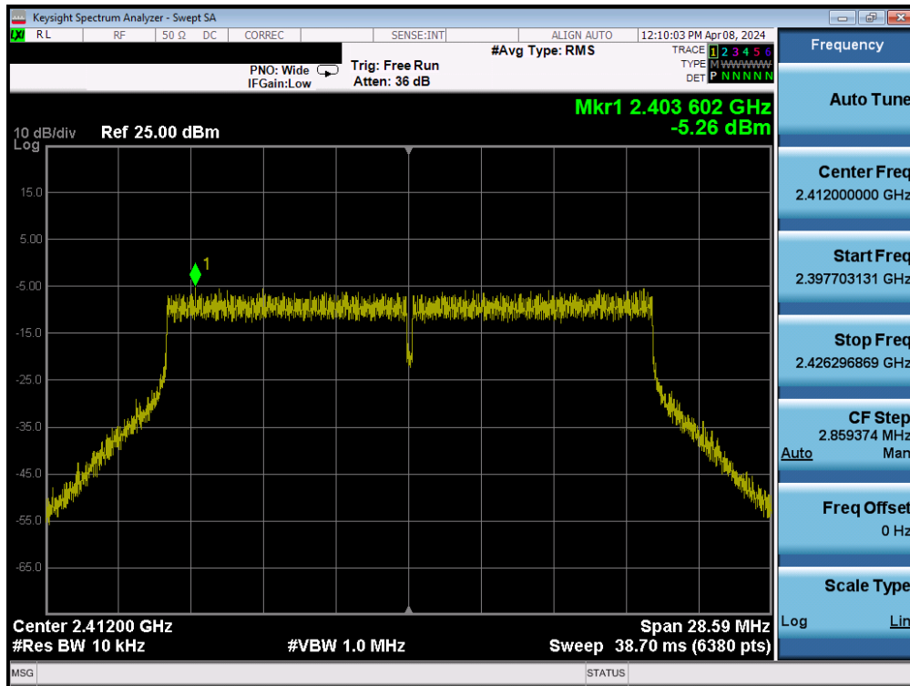
Plot 7-46. Power Spectral Density Plot SISO ANT2 (802.11ax/be (2.4GHz) – Ch. 1)
