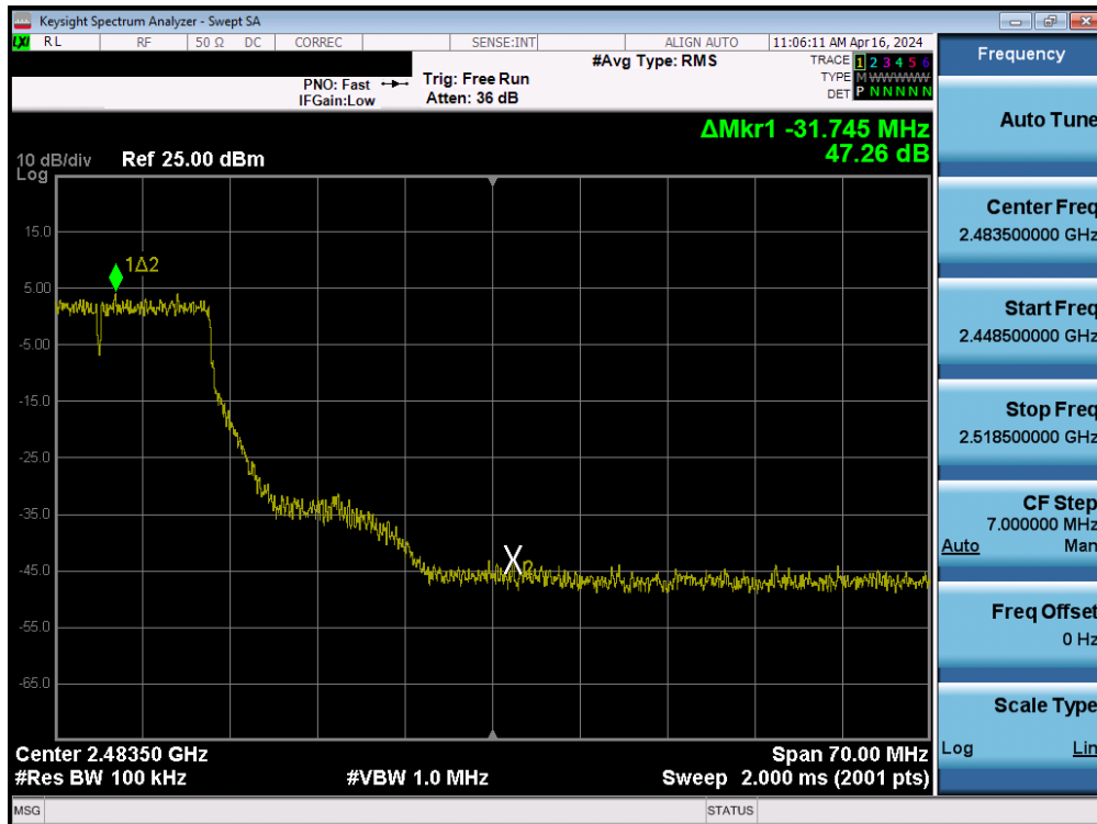
Plot 7-104. Band Edge Plot MIMO ANT1 (802.11n (2.4GHz) – Ch. 9)
