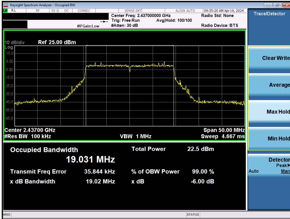
Plot 7-35. 6dB Bandwidth Plot MIMO ANT2 (802.11ax/be (2.4GHz) – Ch. 6)
