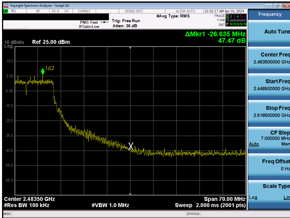
Plot 7-78. Band Edge Plot SISO ANT2 (802.11g - Ch. 9)
