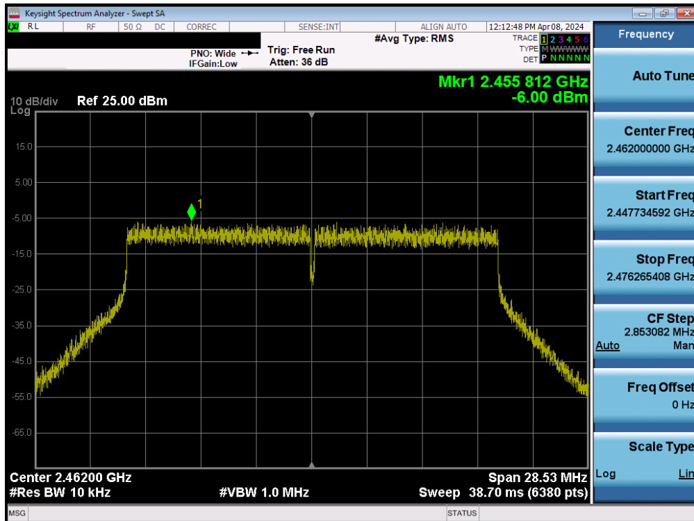
Plot 7-48. Power Spectral Density Plot SISO ANT2 (802.11ax/be (2.4GHz) – Ch. 11)
