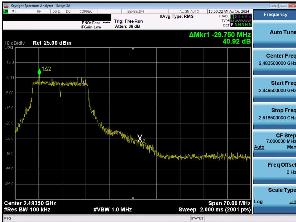
Plot 7-100. Band Edge Plot MIMO ANT1 (802.11g – Ch. 11)
