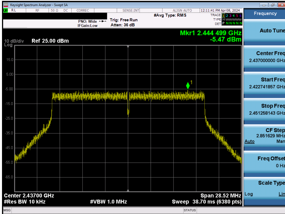
Plot 7-47. Power Spectral Density Plot SISO ANT2 (802.11ax/be (2.4GHz) – Ch. 6)
