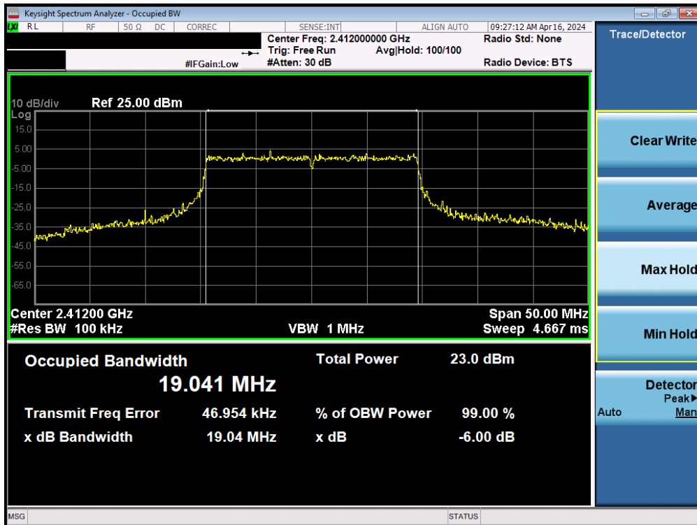
Plot 7-34. 6dB Bandwidth Plot MIMO ANT2 (802.11ax/be (2.4GHz) – Ch. 1)
