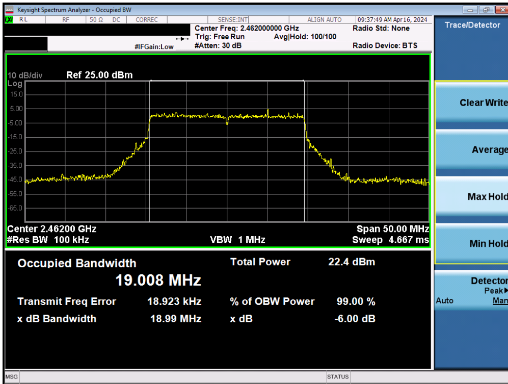
Plot 7-36. 6dB Bandwidth Plot MIMO ANT2 (802.11ax/be (2.4GHz) – Ch. 11)
