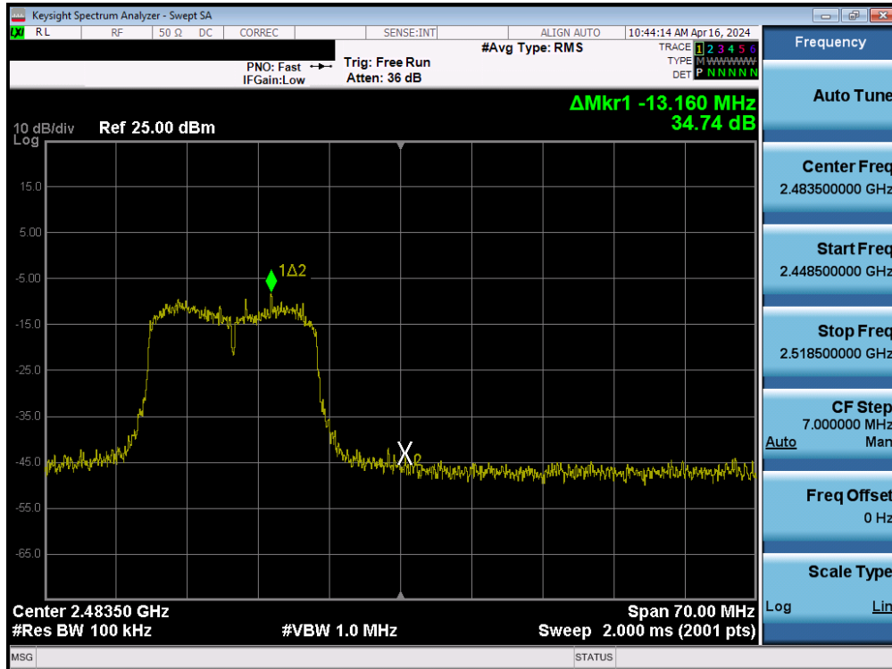
Plot 7-101. Band Edge Plot MIMO ANT1 (802.11g – Ch. 12)
