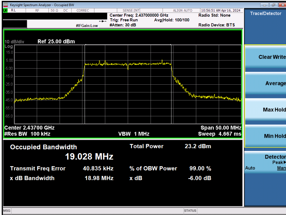
Plot 7-23. 6dB Bandwidth Plot MIMO ANT1 (802.11ax/be (2.4GHz) – Ch. 6)
