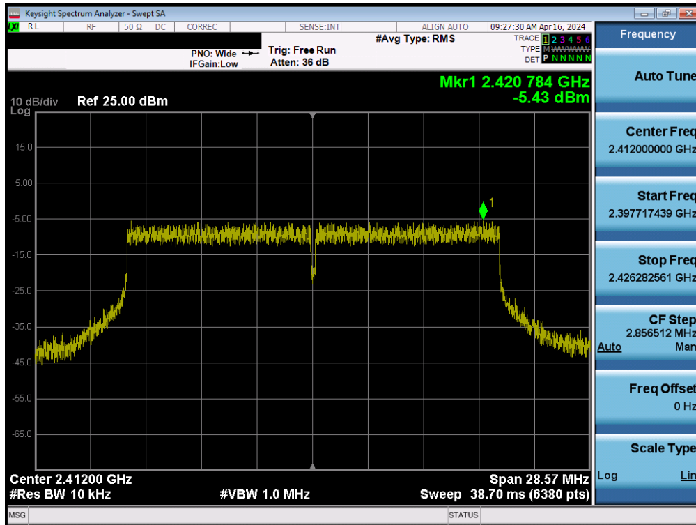
Plot 7-70. Power Spectral Density Plot MIMO ANT2 (802.11ax/be (2.4GHz) – Ch. 1)
