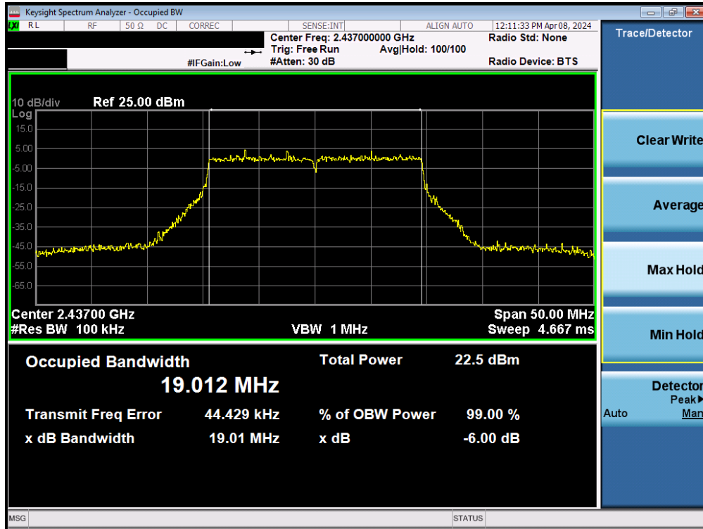
Plot 7-11. 6dB Bandwidth Plot SISO ANT2 (802.11ax/be (2.4GHz) – Ch. 6)
