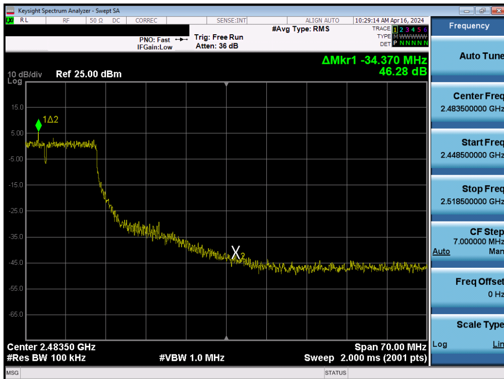
Plot 7-84. Band Edge Plot SISO ANT2 (802.11n (2.4GHz) – Ch. 9)
