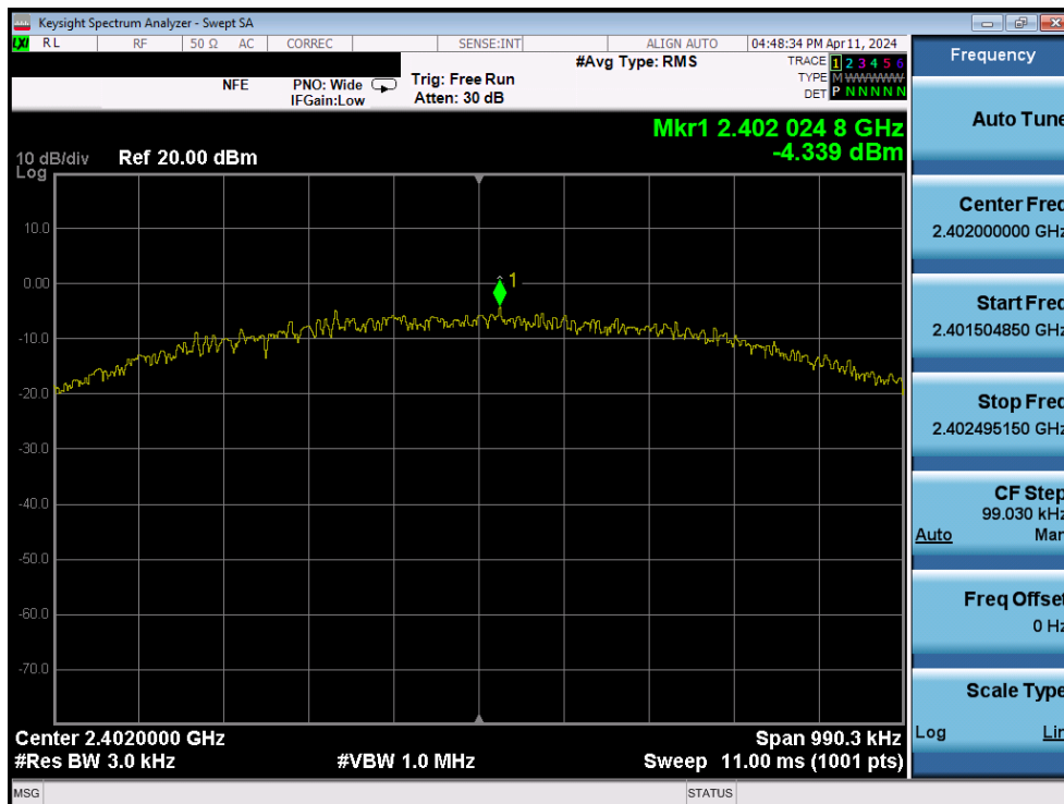
Plot 7-85. Power Spectral Density Plot (Bluetooth (LE), 1Mbps – Ch. 0) – Dual Ant2
