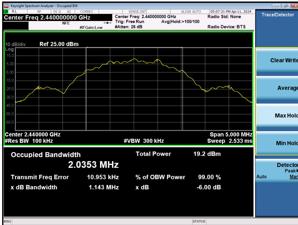
Plot 7-29. 6dB Bandwidth Plot (Bluetooth (LE), 2Mbps – Ch. 19 – Dual Ant2)
