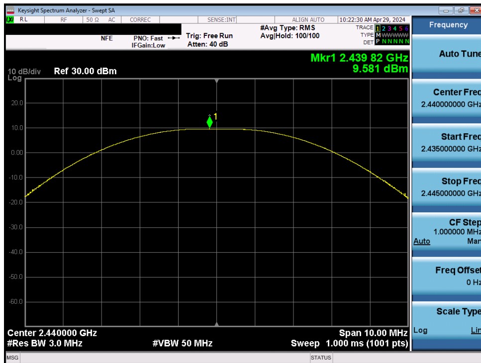
Plot 7-59. Peak Power Plot (Bluetooth (LE), 2Mbps – Ch. 19) – Dual Ant2
