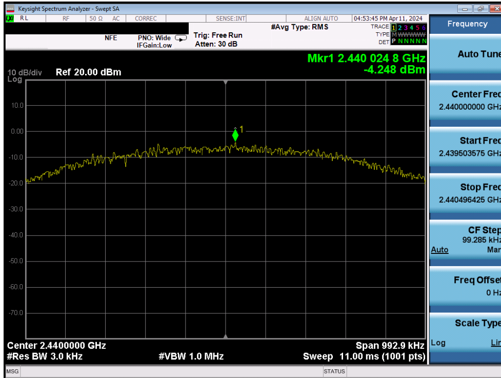
Plot 7-86. Power Spectral Density Plot (Bluetooth (LE), 1Mbps – Ch. 19) – Dual Ant2
