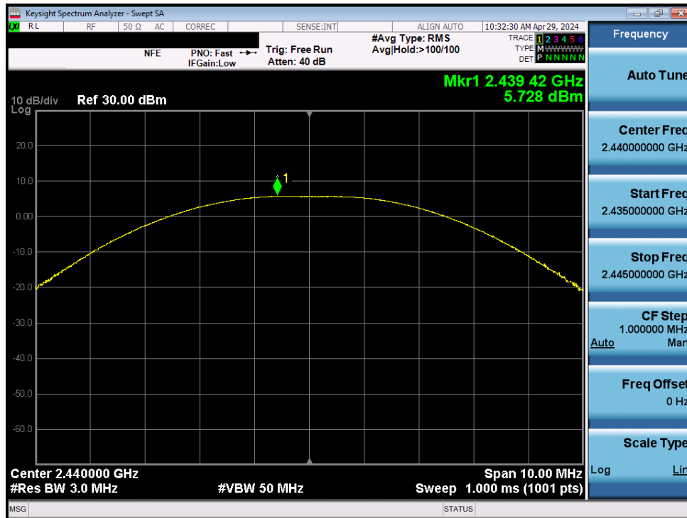
Plot 7-53. Peak Power Plot (Bluetooth (LE), 2Mbps – Ch. 19) – Dual Ant1
