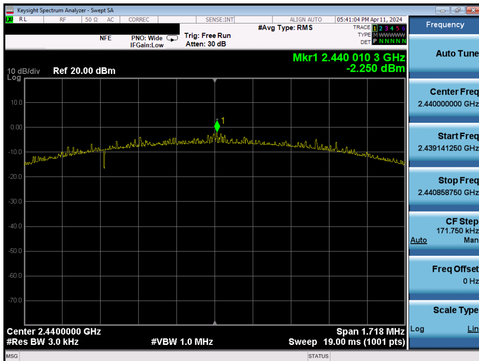
Plot 7-77. Power Spectral Density Plot (Bluetooth (LE), 2Mbps – Ch. 19) – Ant2
