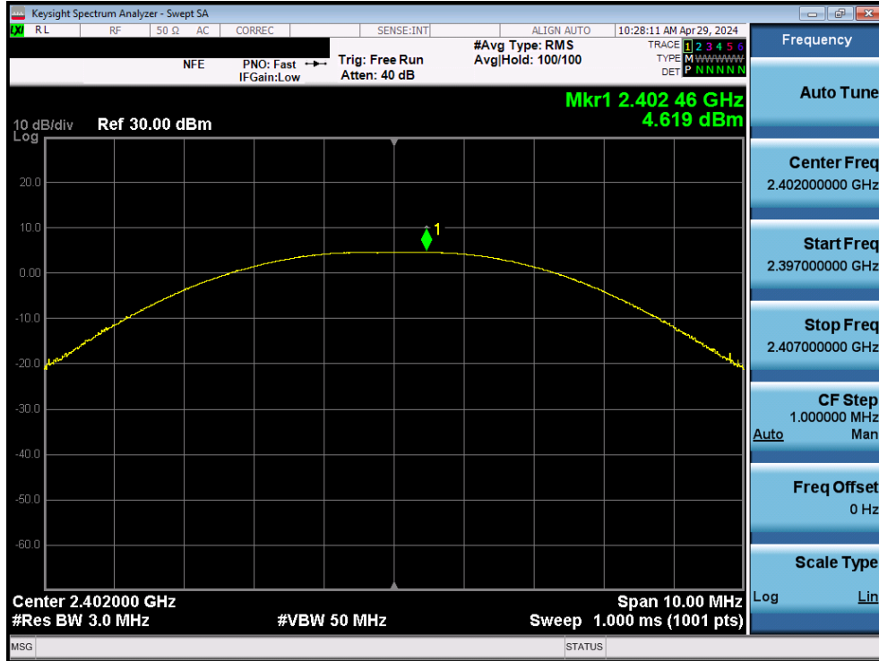
Plot 7-52. Peak Power Plot (Bluetooth (LE), 2Mbps – Ch. 0) – Dual Ant1
