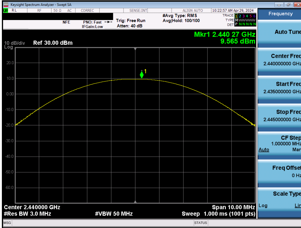
Plot 7-56. Peak Power Plot (Bluetooth (LE), 1Mbps – Ch. 19) – Dual Ant2
