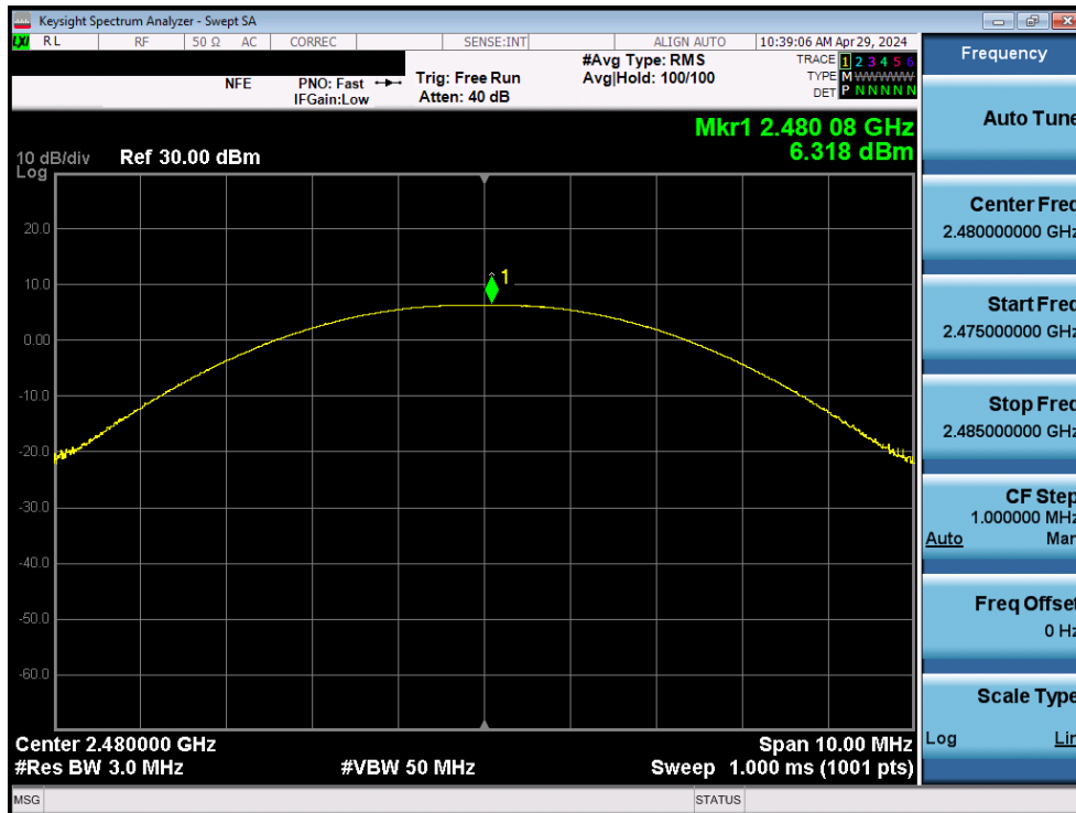
Plot 7-51. Peak Power Plot (Bluetooth (LE), 1Mbps – Ch. 39) – Dual Ant1
