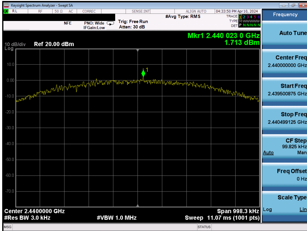
Plot 7-68. Power Spectral Density Plot (Bluetooth (LE), 1Mbps – Ch. 19) – Ant1
