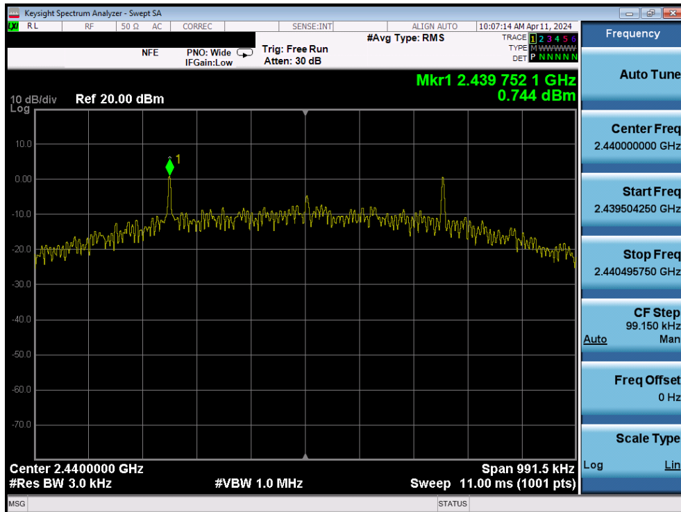
Plot 7-65. Power Spectral Density Plot (Bluetooth (LE), 500kbps – Ch. 19) – Ant1
