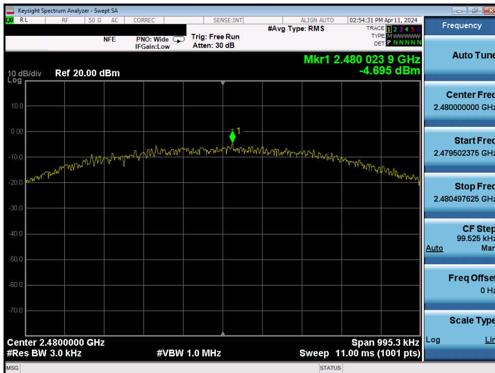
Plot 7-81. Power Spectral Density Plot (Bluetooth (LE), 1Mbps – Ch. 39) – Dual Ant1
