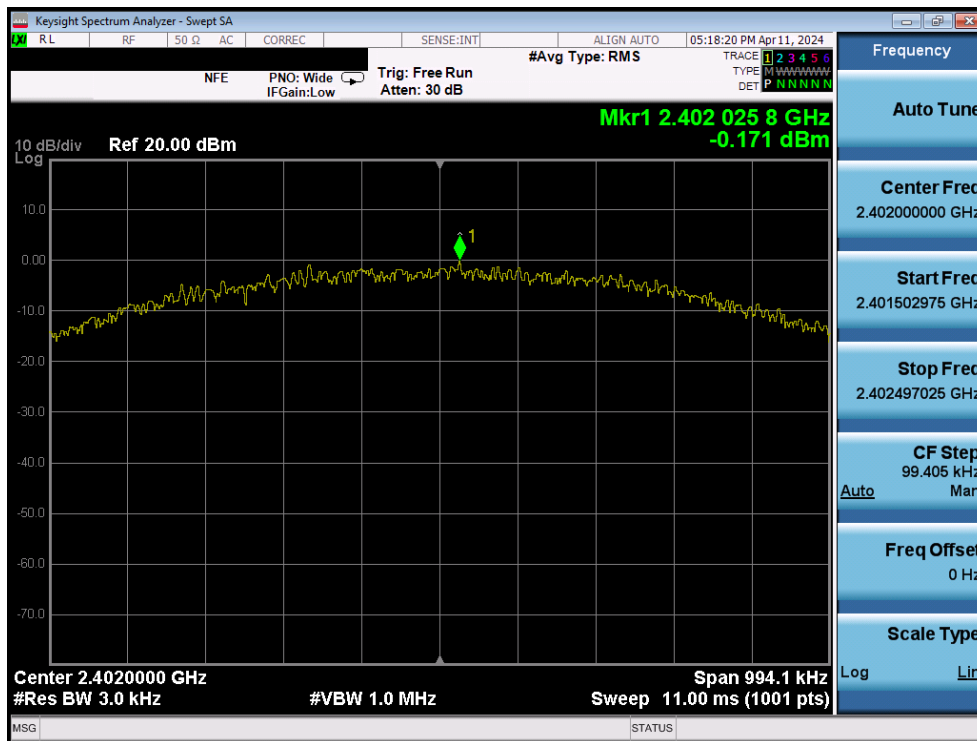
Plot 7-73. Power Spectral Density Plot (Bluetooth (LE), 1Mbps – Ch. 0) – Ant2
