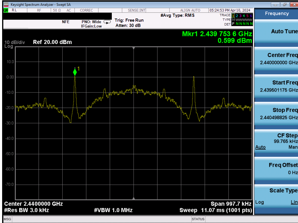
Plot 7-62. Power Spectral Density Plot (Bluetooth (LE), 125kbps – Ch. 19) – Ant1
