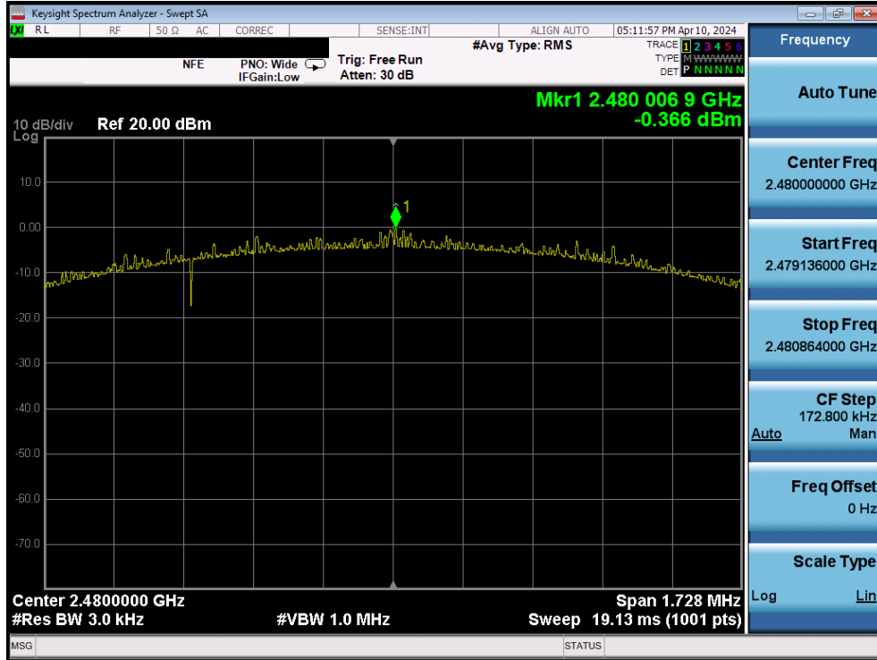
Plot 7-72. Power Spectral Density Plot (Bluetooth (LE), 2Mbps – Ch. 39) – Ant1
