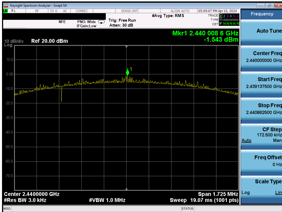
Plot 7-71. Power Spectral Density Plot (Bluetooth (LE), 2Mbps – Ch. 19) – Ant1
