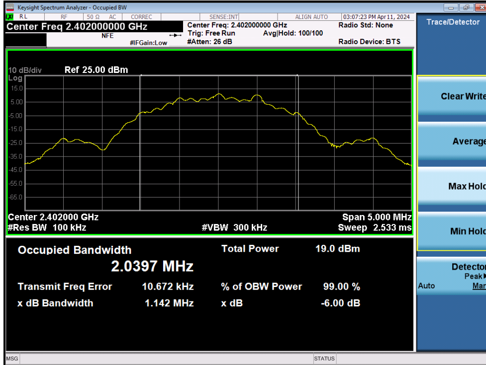
Plot 7-22. 6dB Bandwidth Plot (Bluetooth (LE), 2Mbps – Ch. 0 – Dual Ant1)
