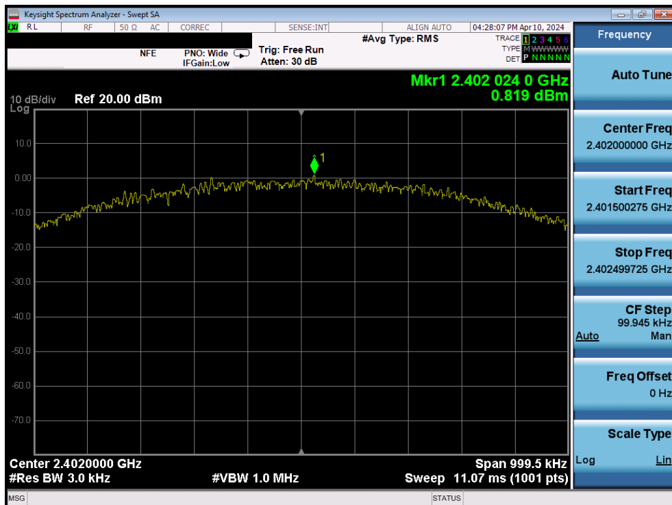
Plot 7-67. Power Spectral Density Plot (Bluetooth (LE), 1Mbps – Ch. 0) – Ant1
