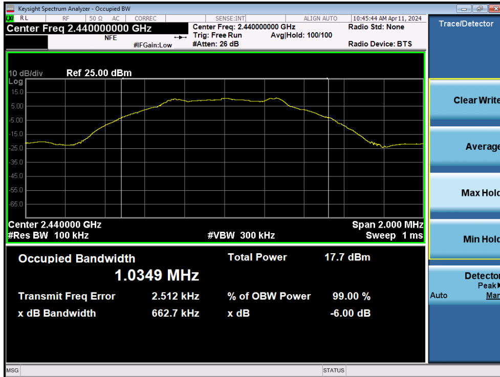
Plot 7-20. 6dB Bandwidth Plot (Bluetooth (LE), 1Mbps – Ch. 19 – Dual Ant1)
