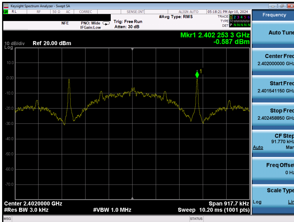
Plot 7-61. Power Spectral Density Plot (Bluetooth (LE), 125kbps – Ch. 0) – Ant1
