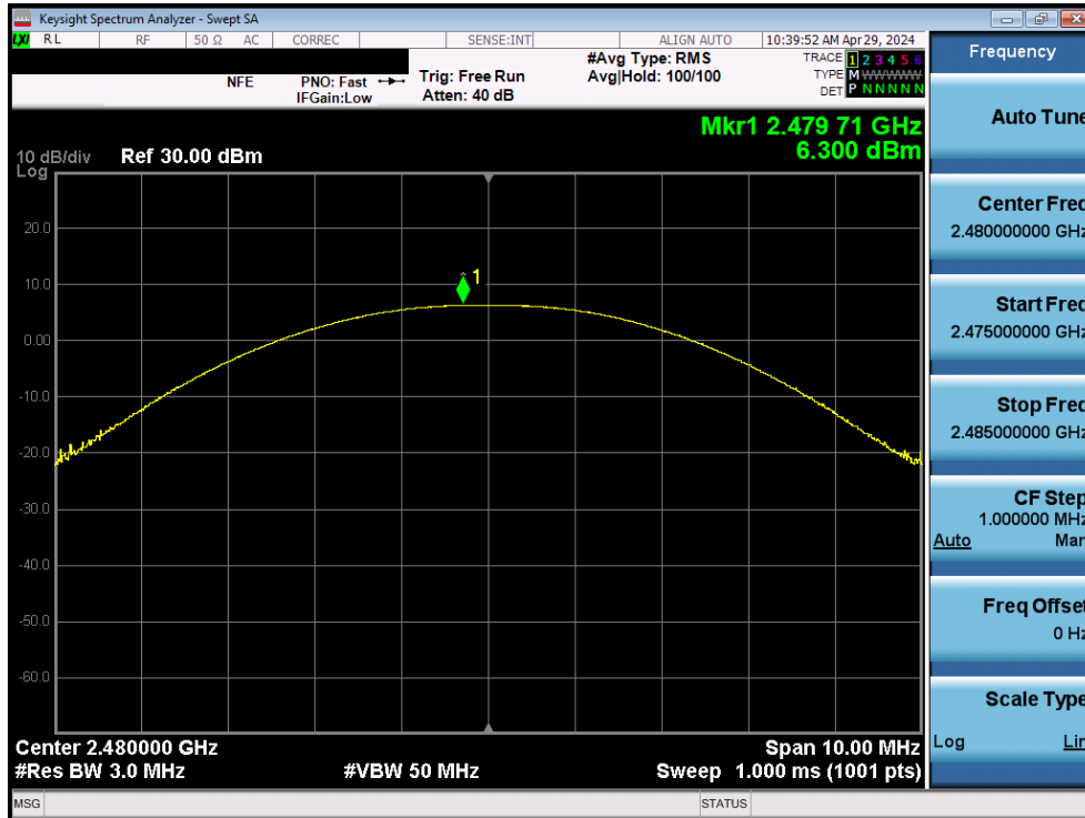
Plot 7-36. Peak Power Plot (Bluetooth (LE), 500kbps – Ch. 39) – Ant1
