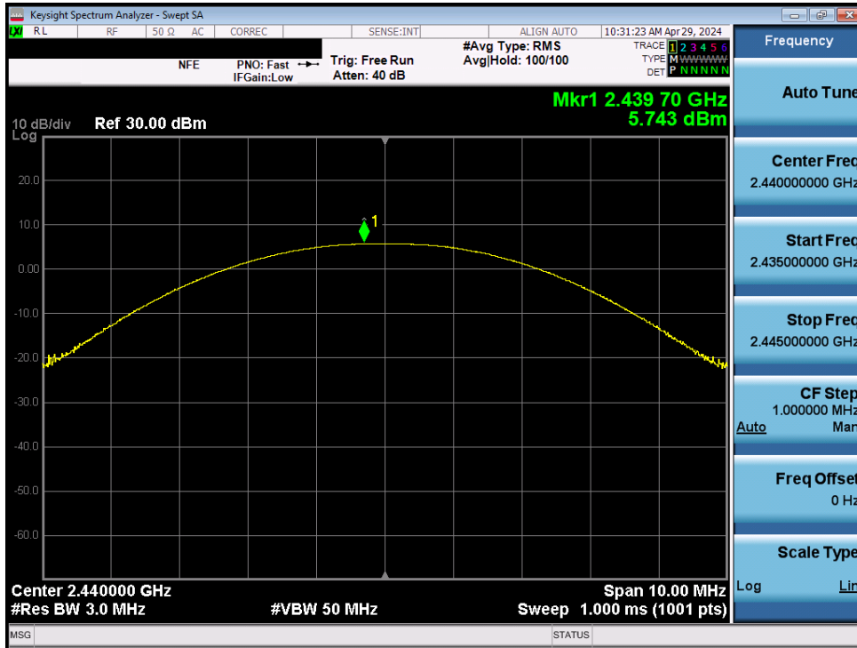
Plot 7-32. Peak Power Plot (Bluetooth (LE), 125kbps – Ch. 19) – Ant1
