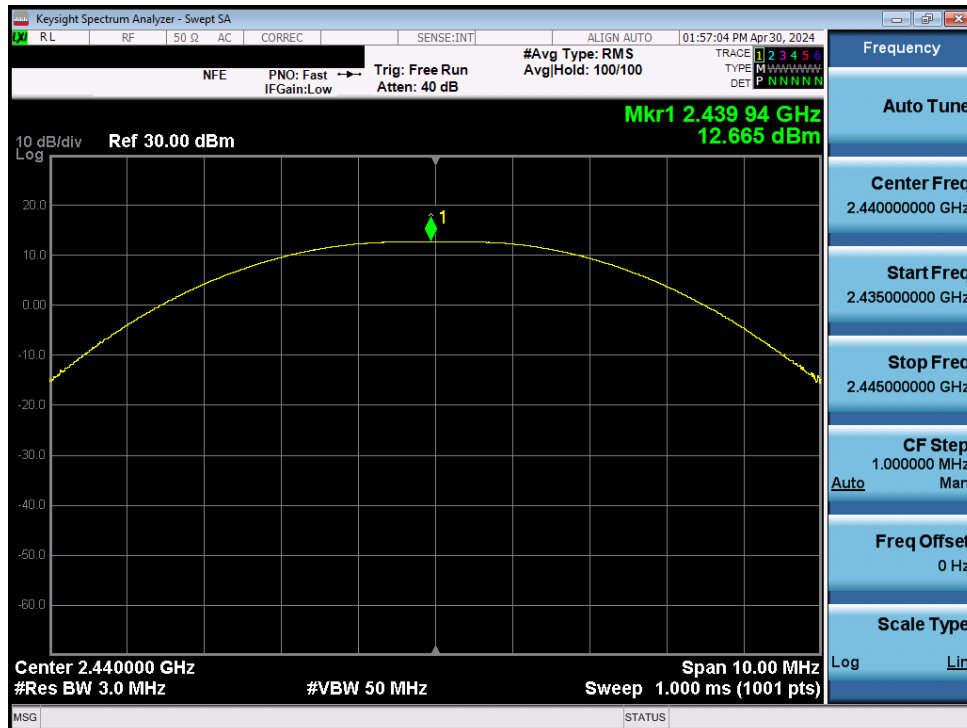
Plot 7-41. Peak Power Plot (Bluetooth (LE), 2Mbps – Ch. 19) – Ant1
