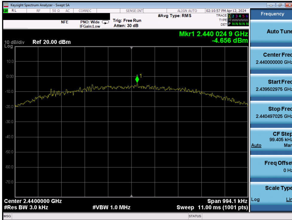
Plot 7-80. Power Spectral Density Plot (Bluetooth (LE), 1Mbps – Ch. 19) – Dual Ant1
