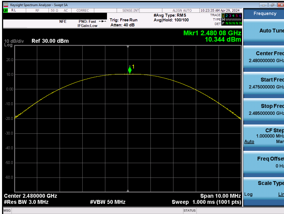
Plot 7-57. Peak Power Plot (Bluetooth (LE), 1Mbps – Ch. 39) – Dual Ant2
