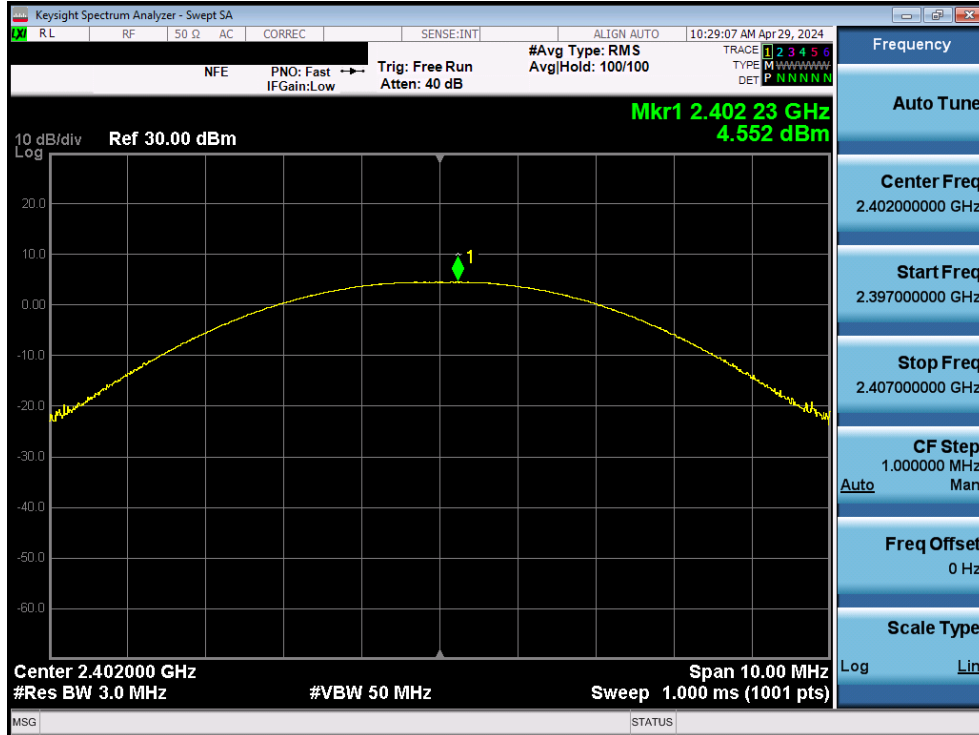
Plot 7-34. Peak Power Plot (Bluetooth (LE), 500kbps – Ch. 0) – Ant1
