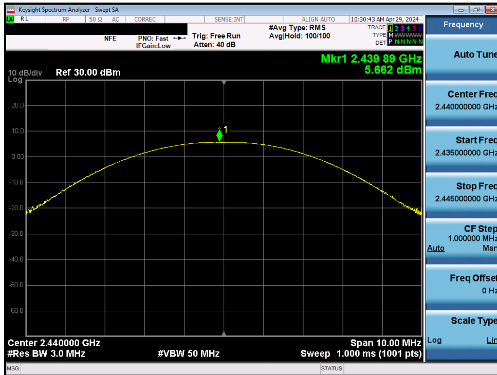
Plot 7-35. Peak Power Plot (Bluetooth (LE), 500kbps – Ch. 19) – Ant1
