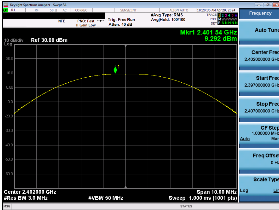
Plot 7-58. Peak Power Plot (Bluetooth (LE), 2Mbps – Ch. 0) – Dual Ant2
