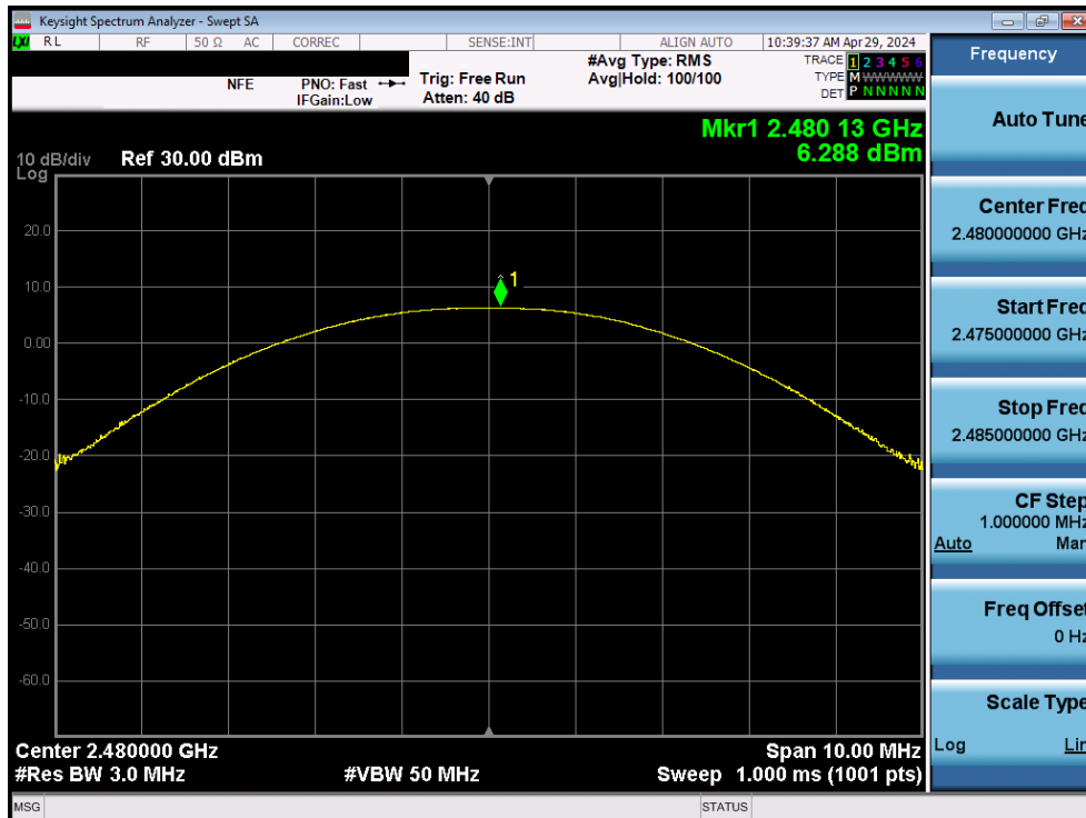
Plot 7-33. Peak Power Plot (Bluetooth (LE), 125kbps – Ch. 39) – Ant1
