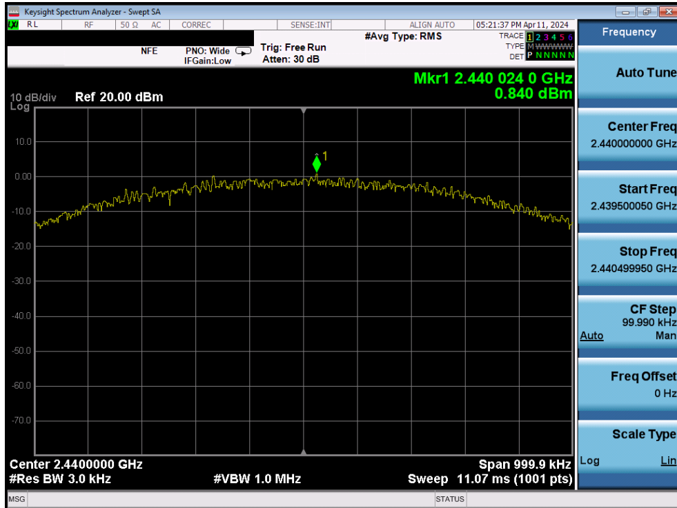
Plot 7-74. Power Spectral Density Plot (Bluetooth (LE), 1Mbps – Ch. 19) – Ant2
