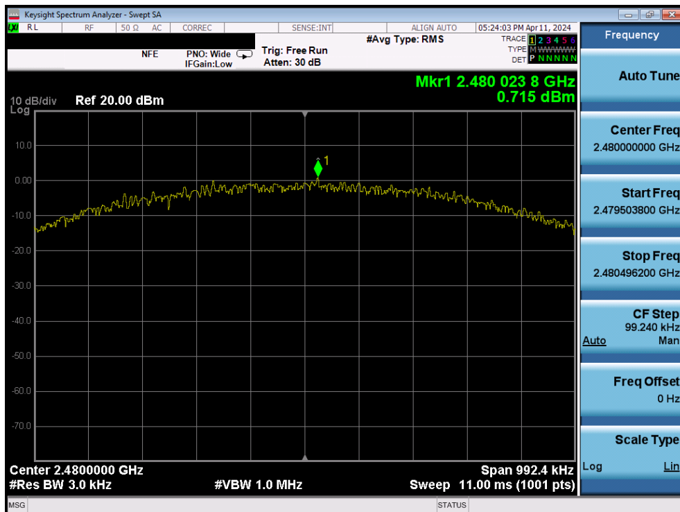
Plot 7-75. Power Spectral Density Plot (Bluetooth (LE), 1Mbps – Ch. 39) – Ant2
