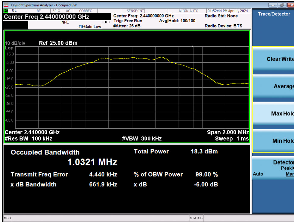
Plot 7-26. 6dB Bandwidth Plot (Bluetooth (LE), 1Mbps – Ch. 19 – Dual Ant2)
