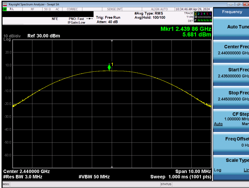
Plot 7-50. Peak Power Plot (Bluetooth (LE), 1Mbps – Ch. 19) – Dual Ant1
