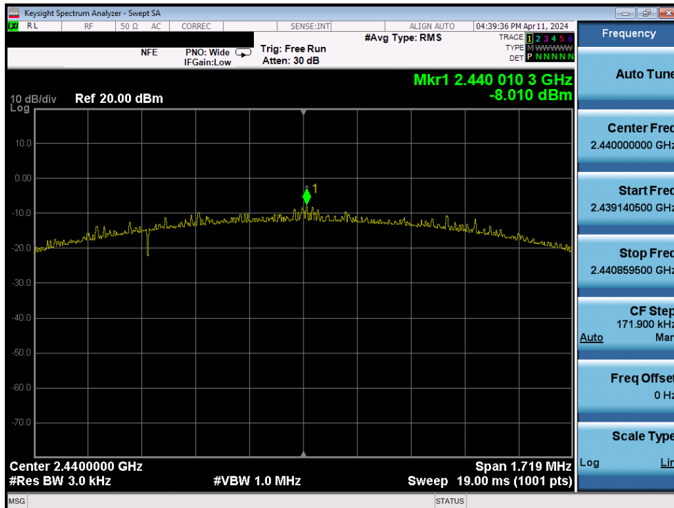
Plot 7-83. Power Spectral Density Plot (Bluetooth (LE), 2Mbps – Ch. 19) – Dual Ant1
