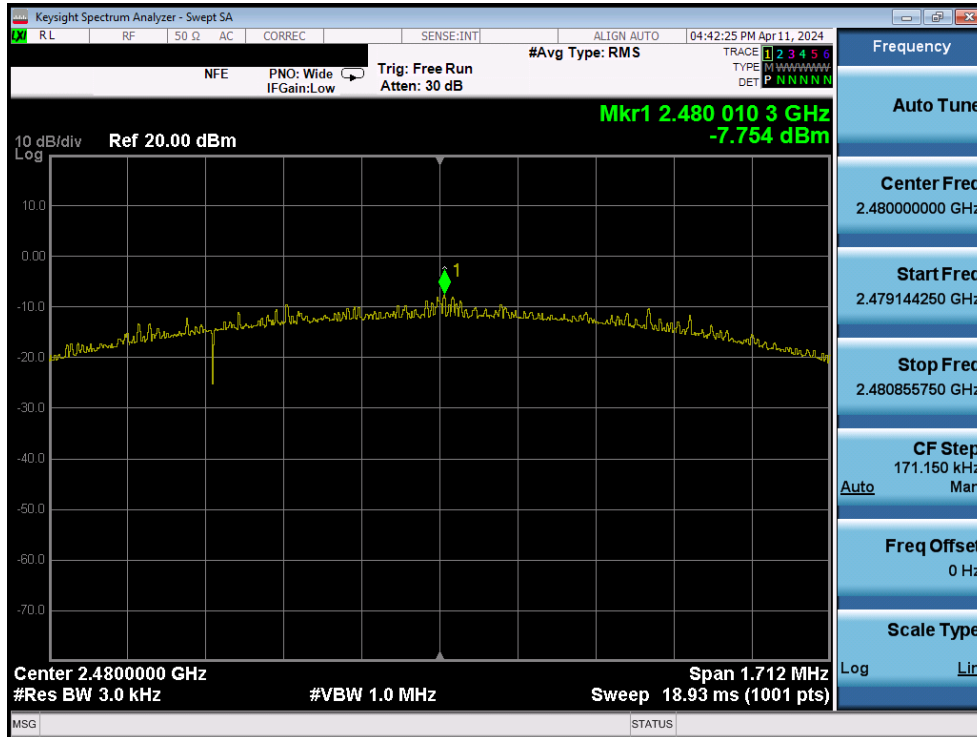
Plot 7-84. Power Spectral Density Plot (Bluetooth (LE), 2Mbps – Ch. 39) – Dual Ant2
