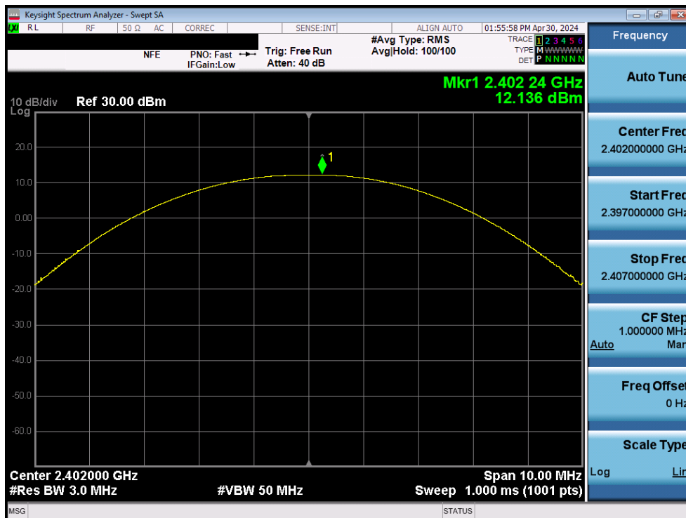
Plot 7-37. Peak Power Plot (Bluetooth (LE), 1Mbps – Ch. 0) – Ant1
