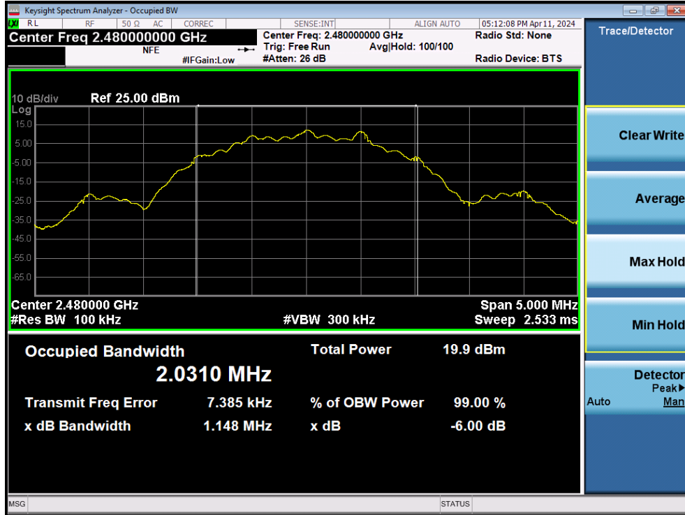
Plot 7-30. 6dB Bandwidth Plot (Bluetooth (LE), 2Mbps – Ch. 39 – Dual Ant2)
