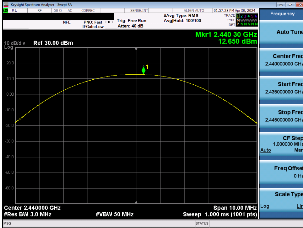
Plot 7-38. Peak Power Plot (Bluetooth (LE), 1Mbps – Ch. 19) – Ant1
