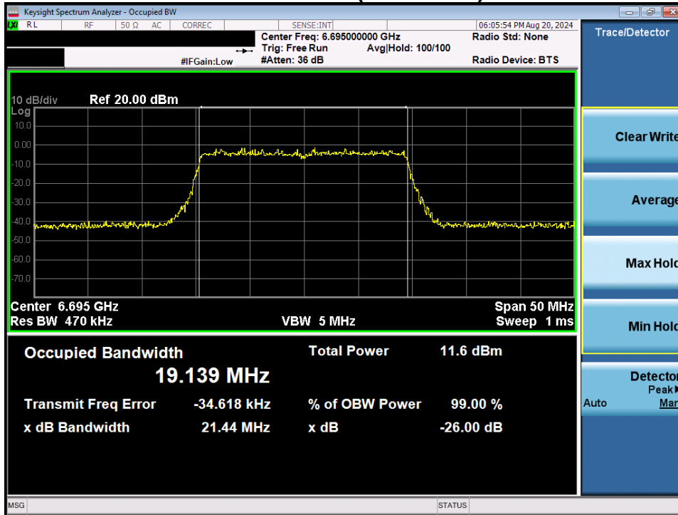
Plot 7-31. Occupied Bandwidth Plot MIMO ANT1 (20MHz BW 802.11ax/be (Full Tones) (UNII Band 7) – Ch. 149)
