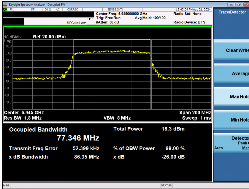
Plot 7-38. Occupied Bandwidth Plot MIMO ANT1 (80MHz BW 802.11ax/be (Full Tones) (UNII Band 8) – Ch. 199)
