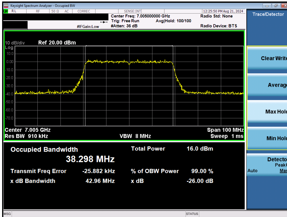
Plot 7-37. Occupied Bandwidth Plot MIMO ANT1 (40MHz BW 802.11ax/be (Full Tones) (UNII Band 8) – Ch. 211)
