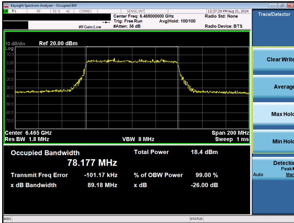
Plot 7-28. Occupied Bandwidth Plot MIMO ANT1 (80MHz BW 802.11ax/be (Full Tones) (UNII Band 6) – Ch. 103)
