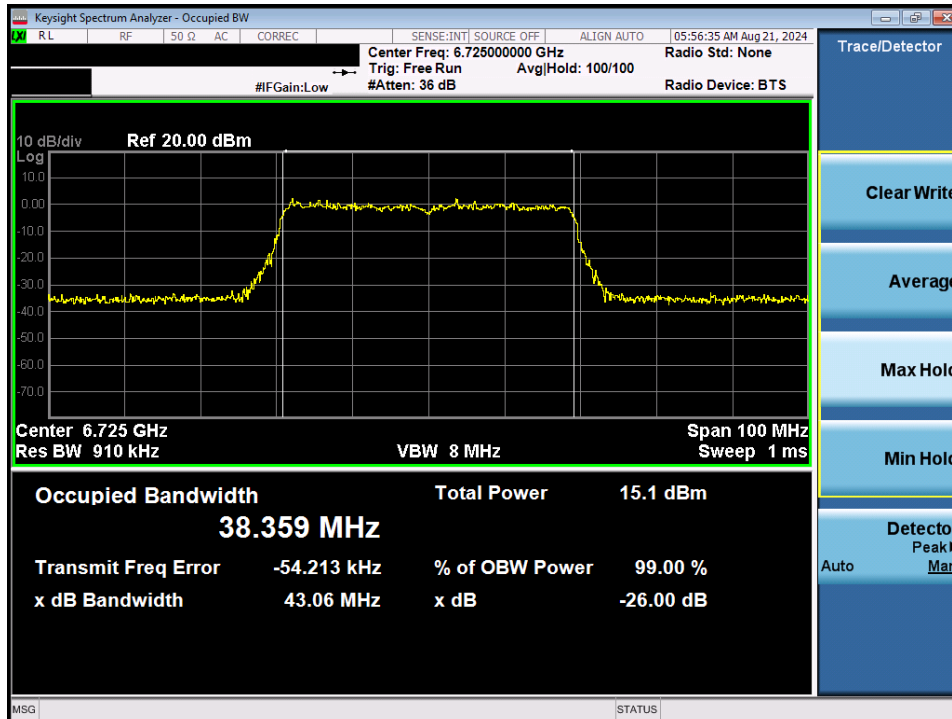
Plot 7-88. Occupied Bandwidth Plot MIMO ANT2 (40MHz BW 802.11ax/be (Full Tones) (UNII Band 7) – Ch. 155)
