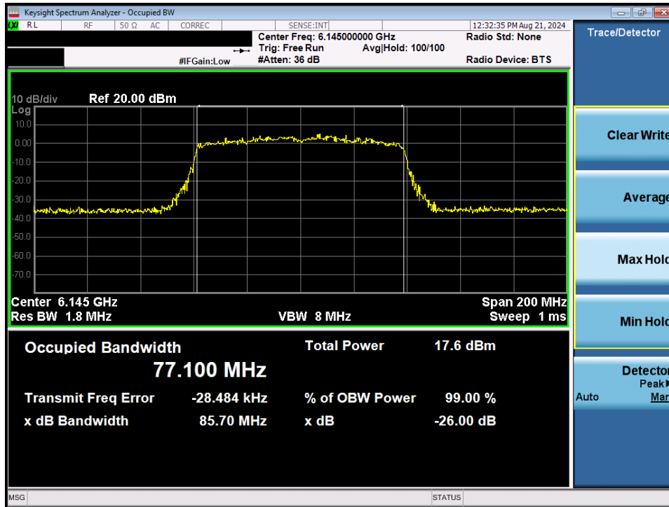
Plot 7-23. Occupied Bandwidth Plot MIMO ANT1 (80MHz BW 802.11ax/be (Full Tones) (UNII Band 5) – Ch. 39)
