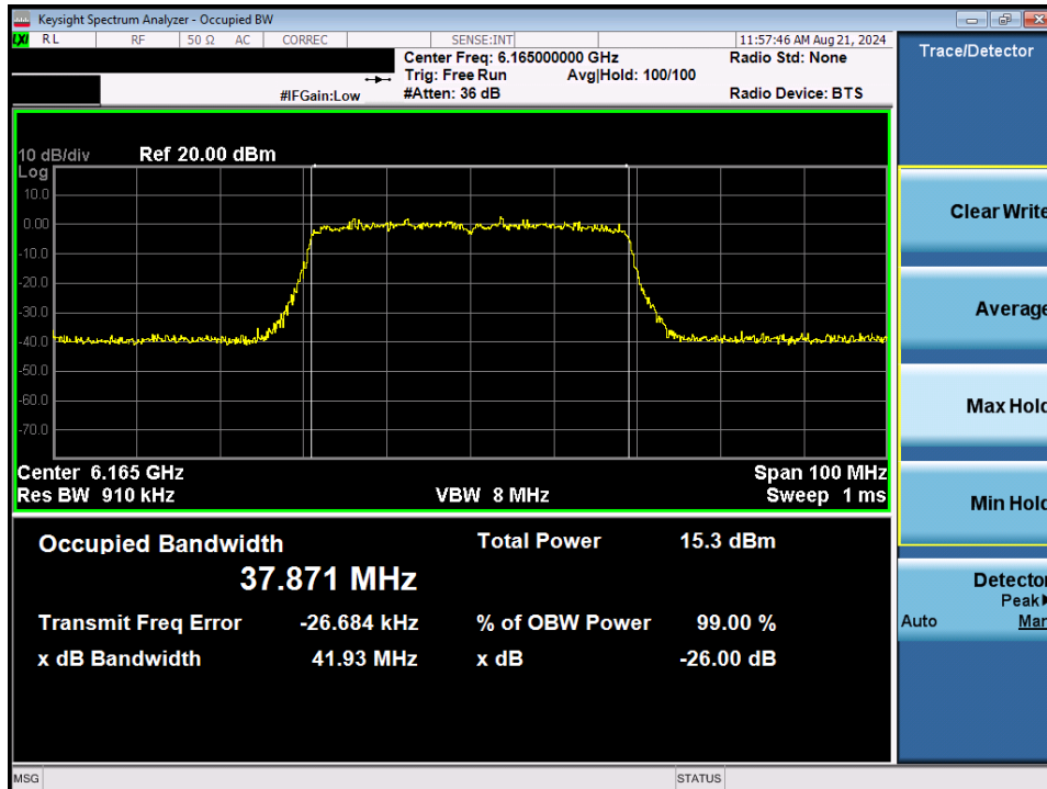
Plot 7-22. Occupied Bandwidth Plot MIMO ANT1 (40MHz BW 802.11ax/be (Full Tones) (UNII Band 5) – Ch. 43)
