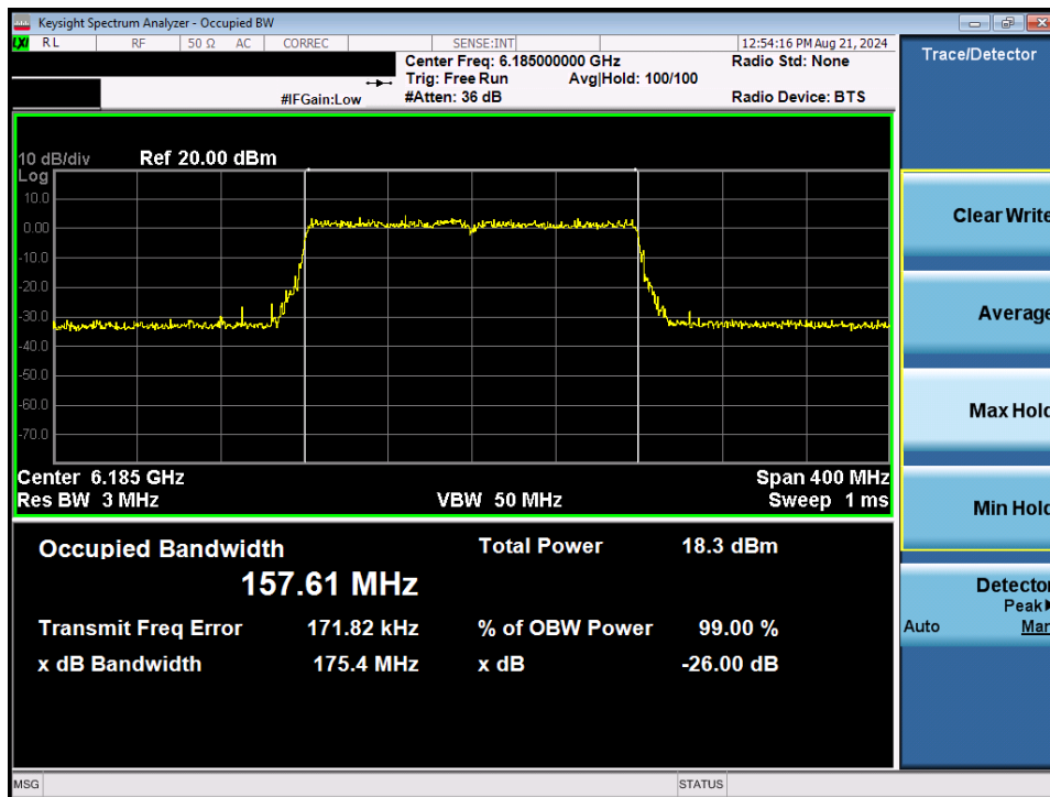
Plot 7-24. Occupied Bandwidth Plot MIMO ANT1 (160MHz BW 802.11ax/be (Full Tones) (UNII Band 5) – Ch. 47)
