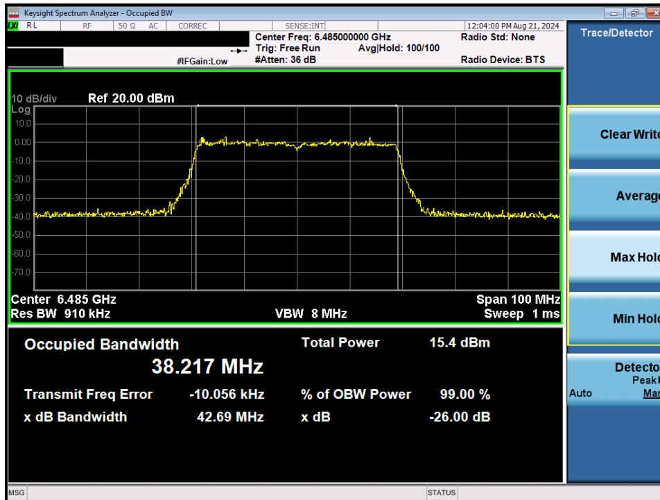
Plot 7-27. Occupied Bandwidth Plot MIMO ANT1 (40MHz BW 802.11ax/be (Full Tones) (UNII Band 6) – Ch. 107)
