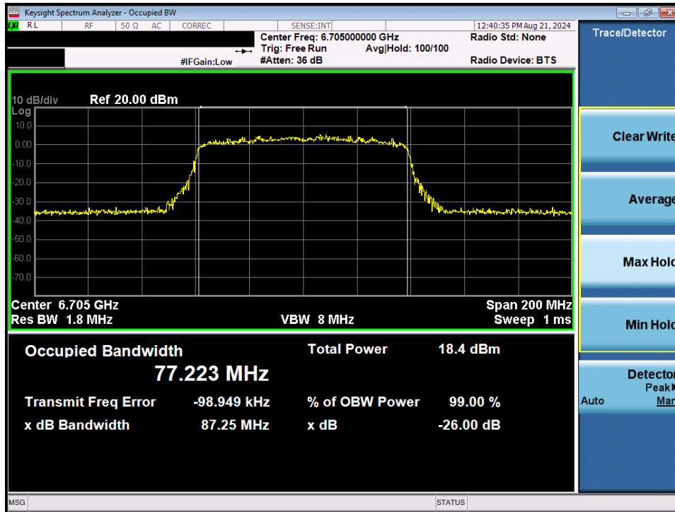
Plot 7-33. Occupied Bandwidth Plot MIMO ANT1 (80MHz BW 802.11ax/be (Full Tones) (UNII Band 7) – Ch. 151)
