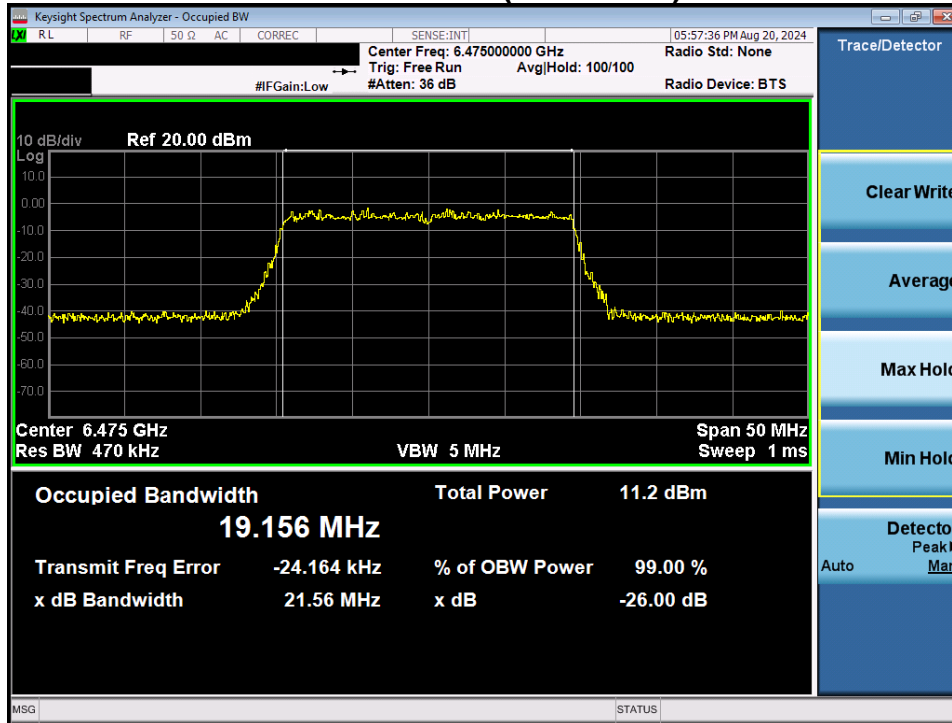
Plot 7-26. Occupied Bandwidth Plot MIMO ANT1 (20MHz BW 802.11ax/be (Full Tones) (UNII Band 6) – Ch. 105)
