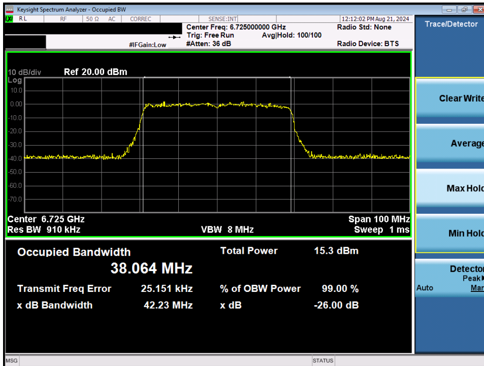
Plot 7-32. Occupied Bandwidth Plot MIMO ANT1 (40MHz BW 802.11ax/be (Full Tones) (UNII Band 7) – Ch. 155)
