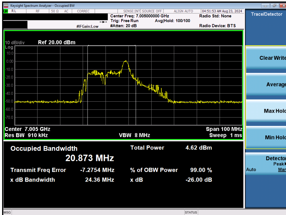
Plot 7-73. Occupied Bandwidth Plot MIMO ANT2 (40MHz BW 802.11ax/be (26 Tones) (UNII Band 8) – Ch. 211)
