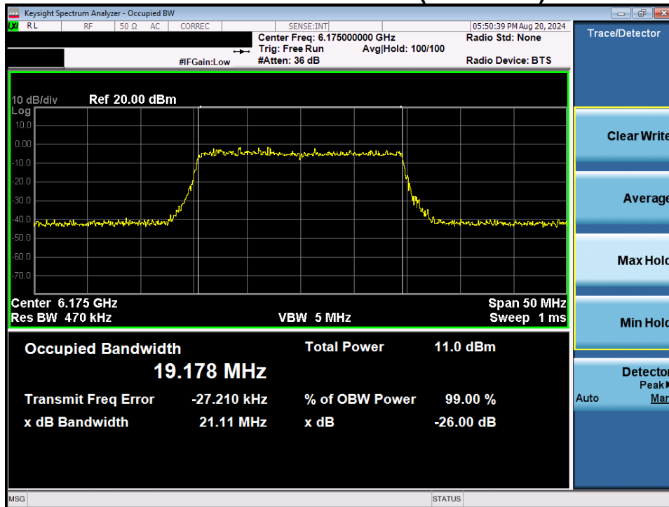
Plot 7-21. Occupied Bandwidth Plot MIMO ANT1 (20MHz BW 802.11ax/be (Full Tones) (UNII Band 5) – Ch. 45)
