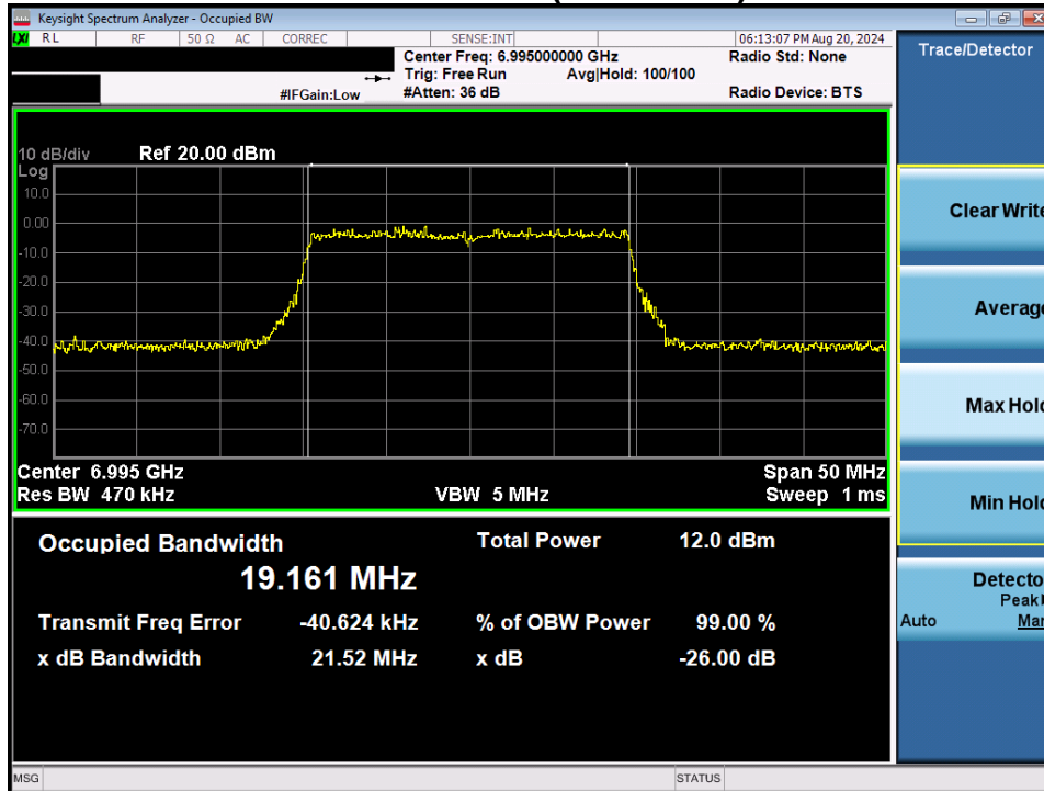
Plot 7-36. Occupied Bandwidth Plot MIMO ANT1 (20MHz BW 802.11ax/be (Full Tones) (UNII Band 8) – Ch. 209)
