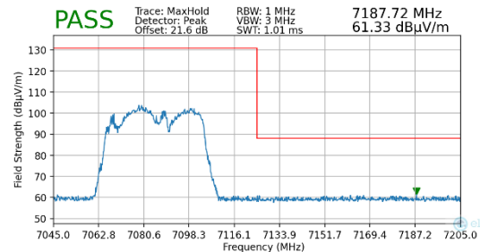
Plot 7-282. Radiated Upper Band Edge Plot MIMO (Peak – UNII Band 8)
