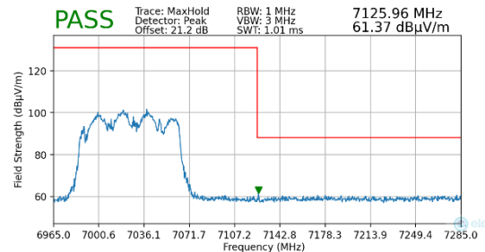
Plot 7-286. Radiated Upper Band Edge Plot MIMO (Peak – UNII Band 8)
