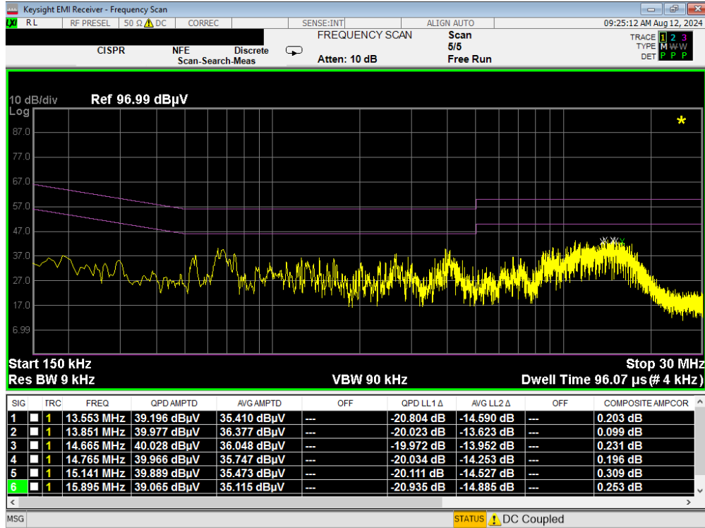
Plot 7-301. Line Conducted Plot with 802.11a UNII Band 8 (L1)
