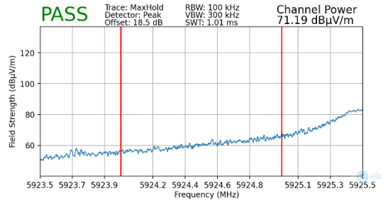
Plot 7-276. Radiated Lower Band Edge Plot MIMO (Peak – UNII Band 5)
