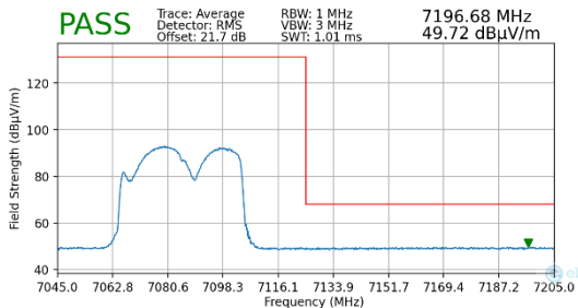
Plot 7-281. Radiated Upper Band Edge Plot MIMO (Average – UNII Band 8)
