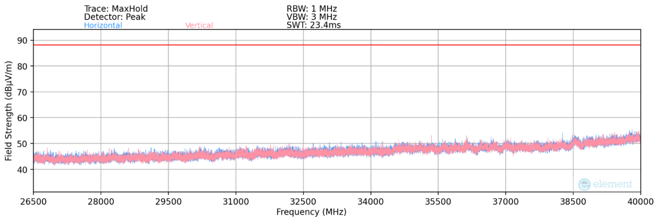
Plot 7-274. Radiated Spurious Plot 26.5GHz - 40GHz (802.11a)
