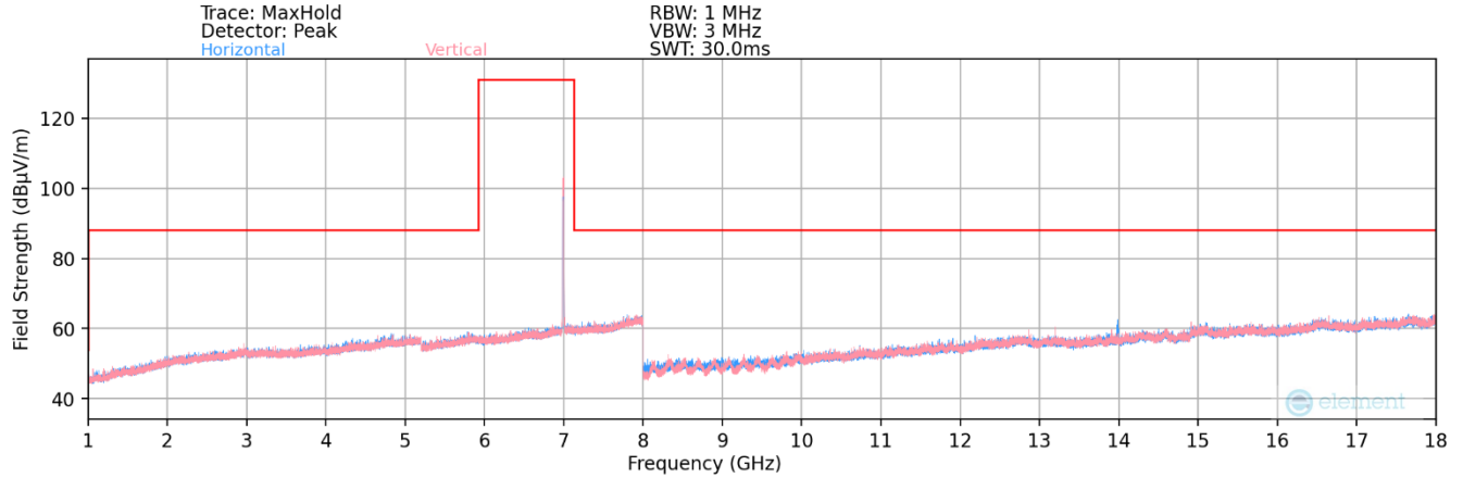
Plot 7-272. Radiated Spurious Plot 1GHz – 18GHz MIMO (802.11a – U Band 8 Ch. 209 – LPI)
