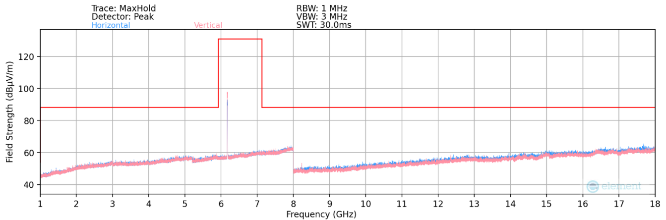
Plot 7-269. Radiated Spurious Plot 1GHz – 18GHz MIMO (802.11a – UNII Band 5 Ch. 45 – LPI/SP)
