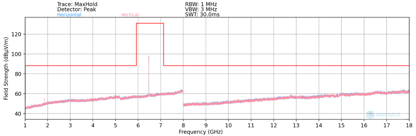
Plot 7-270. Radiated Spurious Plot 1GHz – 18GHz MIMO (802.11a – UNII Band 6 Ch. 105 – LPI)
