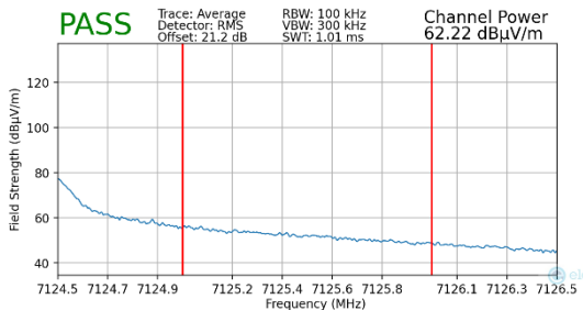
Plot 7-277. Radiated Upper Band Edge Plot MIMO (Average – UNII Band 8)
