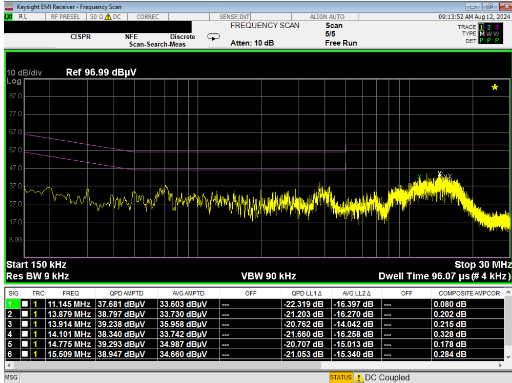
Plot 7-295. Line Conducted Plot with 802.11a UNII Band 5 (L1)
