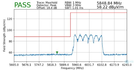
Plot 7-288. Radiated Lower Band Edge Plot MIMO (Peak – UNII Band 5)
