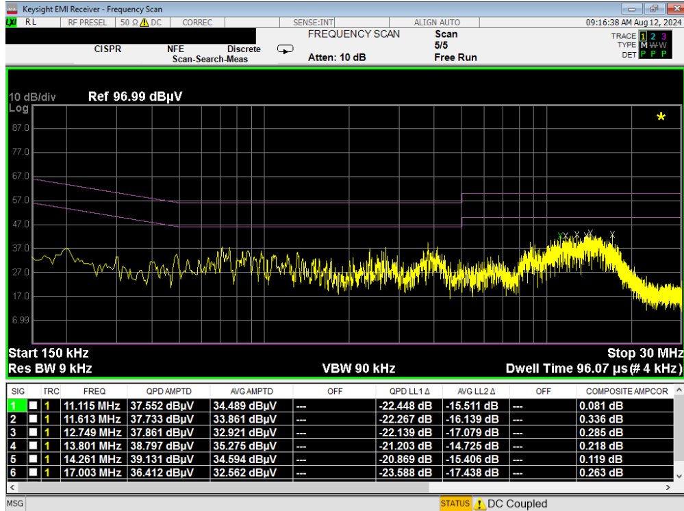
Plot 7-297. Line Conducted Plot with 802.11a UNII Band 6 (L1)
