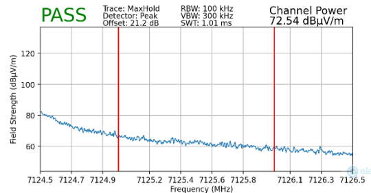
Plot 7-278. Radiated Upper Band Edge Plot MIMO (Peak – UNII Band 8)
