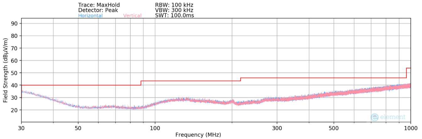
Plot 7-268. Radiated Spurious Plot below 1GHz MIMO (802.11a)
