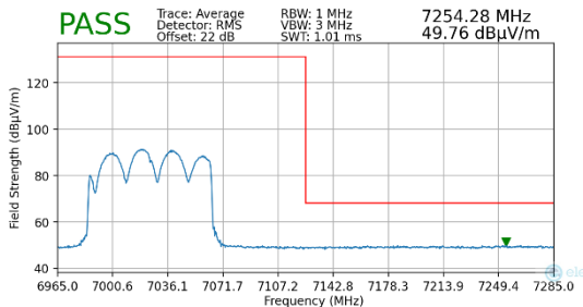
Plot 7-285. Radiated Upper Band Edge Plot MIMO (Average – UNII Band 8)
