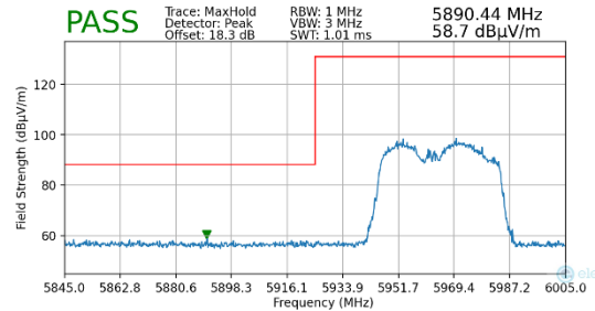
Plot 7-280. Radiated Lower Band Edge Plot MIMO (Peak – UNII Band 5)
