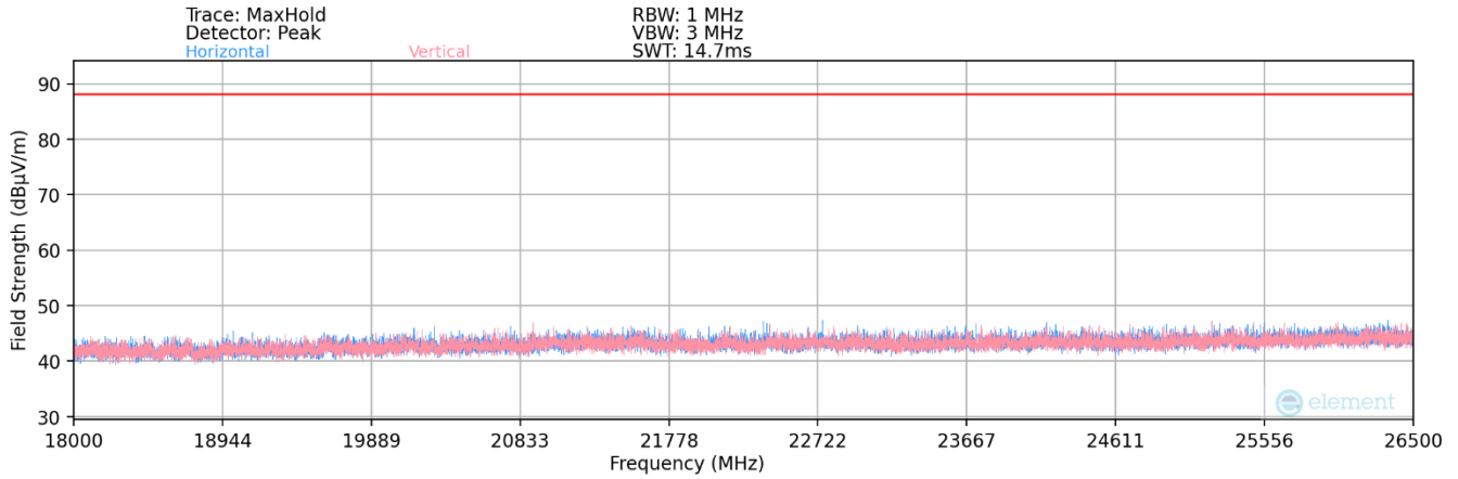
Plot 7-273. Radiated Spurious Plot 18GHz - 26.5GHz (802.11a)
