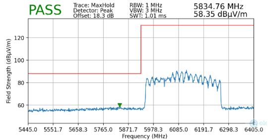
Plot 7-292. Radiated Lower Band Edge Plot MIMO (Peak – UNII Band 5)
