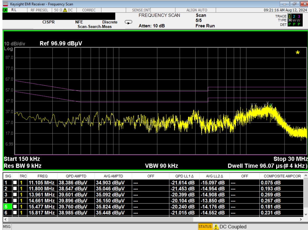
Plot 7-299. Line Conducted Plot with 802.11a UNII Band 7 (L1)
