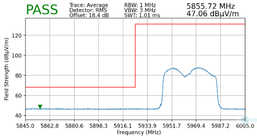
Plot 7-279. Radiated Lower Band Edge Plot MIMO (Average – UNII Band 5)
