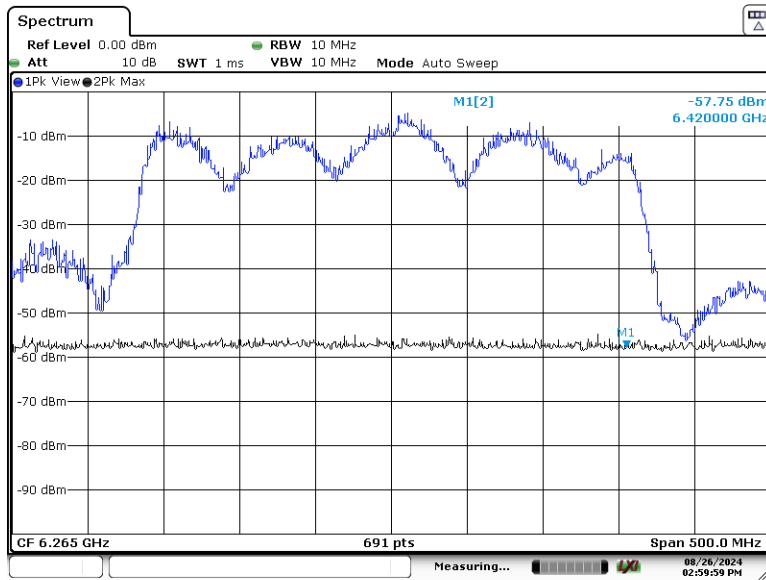
Plot 7-267. CBP 320MHz Channel - Injection Upper Edge – [6420 MHz]
