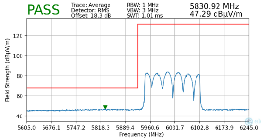
Plot 7-287. Radiated Lower Band Edge Plot MIMO (Average – UNII Band 5)
