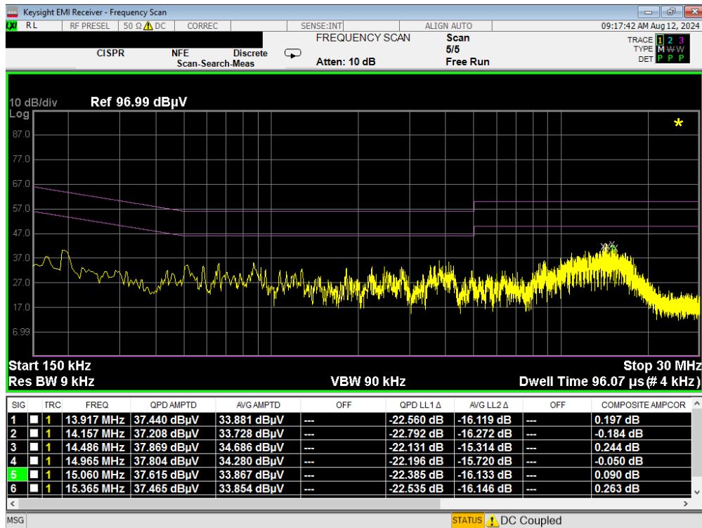
Plot 7-298. Line Conducted Plot with 802.11a UNII Band 6 (N)
