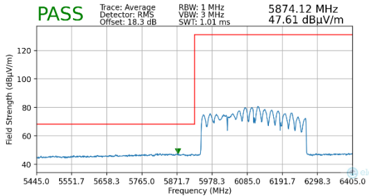
Plot 7-291. Radiated Lower Band Edge Plot MIMO (Average – UNII Band 5)
