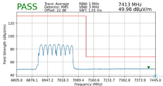
Plot 7-289. Radiated Upper Band Edge Plot MIMO (Average – UNII Band 8)
