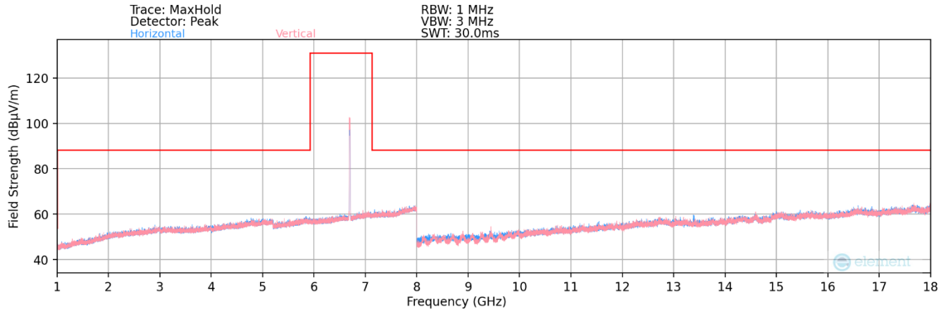
Plot 7-271. Radiated Spurious Plot 1GHz – 18GHz MIMO (802.11a – UNII Band 7 Ch. 149 – LPI/SP)
