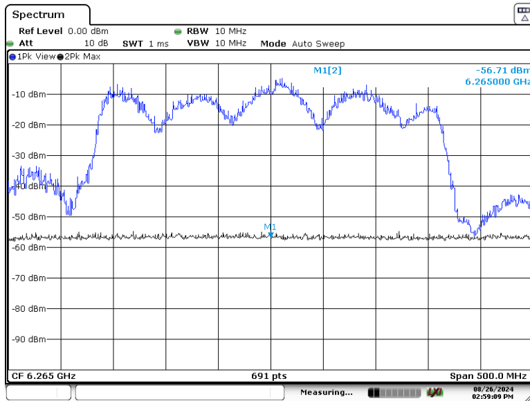
Plot 7-266. CBP 320MHz Channel - Injection Center – [6265 MHz]
