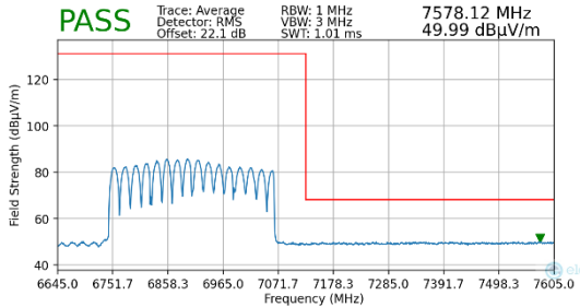
Plot 7-293. Radiated Upper Band Edge Plot MIMO (Average – UNII Band 8)
