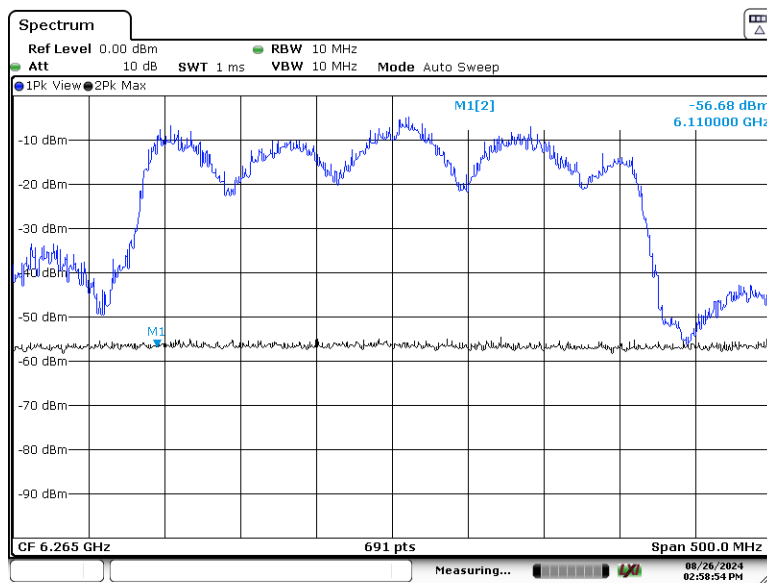
Plot 7-265. CBP 320MHz Channel - Injection Lower Edge – [6110 MHz]
