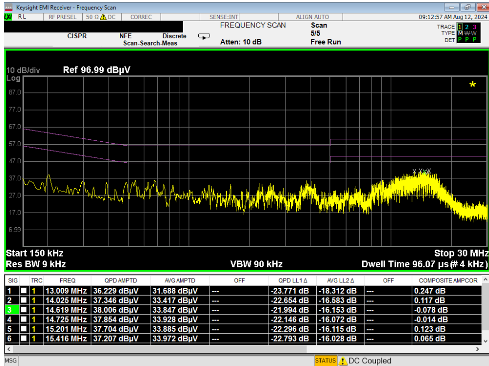
Plot 7-296. Line Conducted Plot with 802.11a UNII Band 5 (N)
