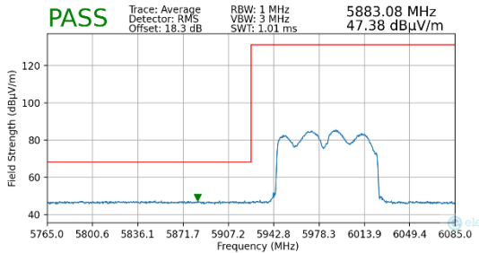
Plot 7-283. Radiated Lower Band Edge Plot MIMO (Average – UNII Band 5)
