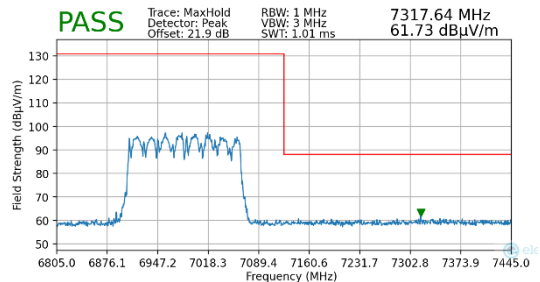
Plot 7-290. Radiated Upper Band Edge Plot MIMO (Peak – UNII Band 8)
