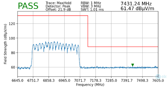
Plot 7-294. Radiated Upper Band Edge Plot MIMO (Peak – UNII Band 8)
