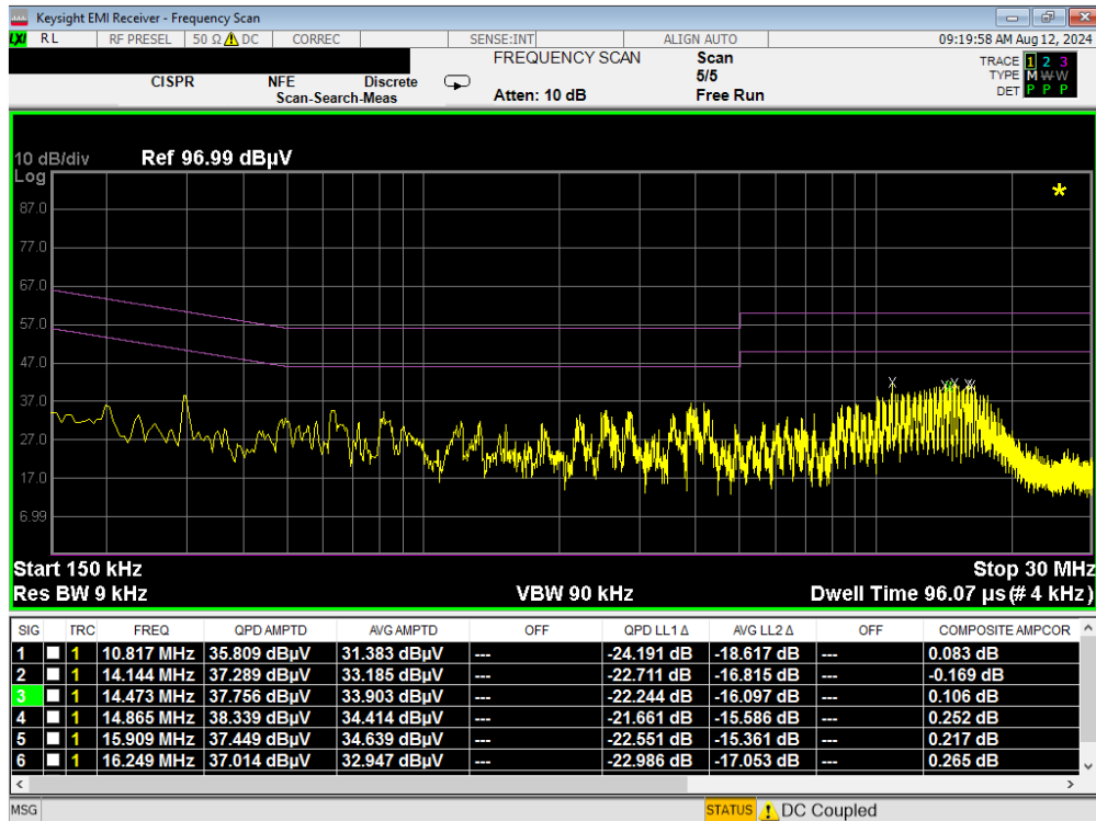
Plot 7-300. Line Conducted Plot with 802.11a UNII Band 7 (N)
