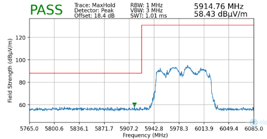
Plot 7-284. Radiated Lower Band Edge Plot MIMO (Peak – UNII Band 5)
