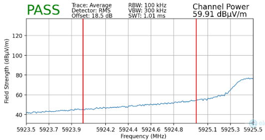
Plot 7-275. Radiated Lower Band Edge Plot MIMO (Average – UNII Band 5)
