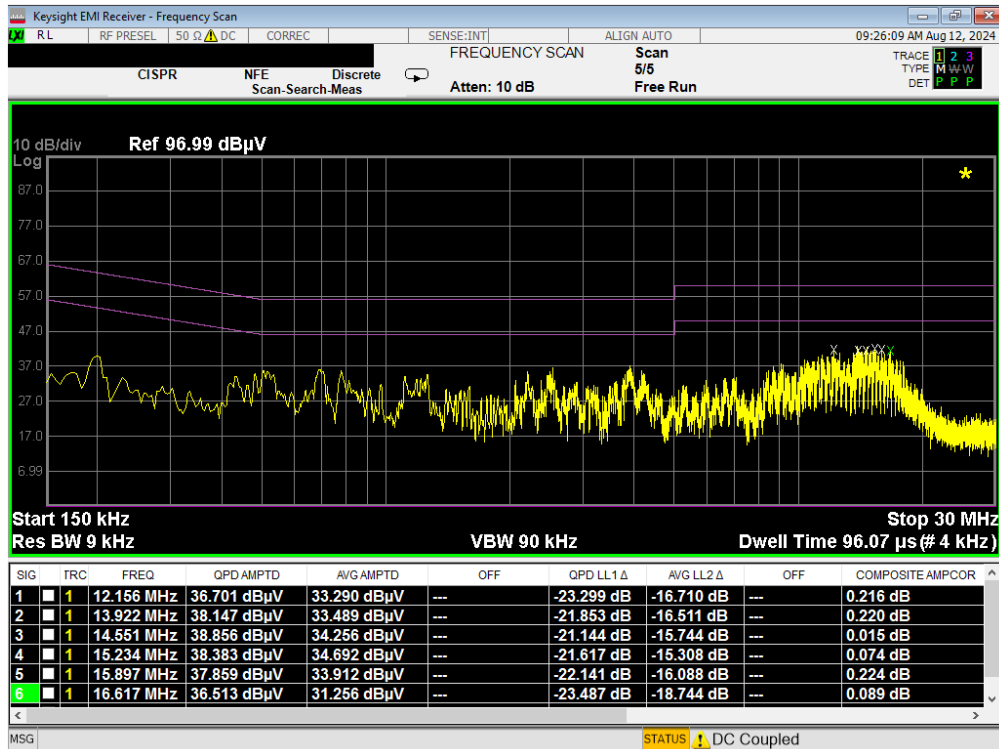
Plot 7-302. Line Conducted Plot with 802.11a UNII Band 8 (N)
