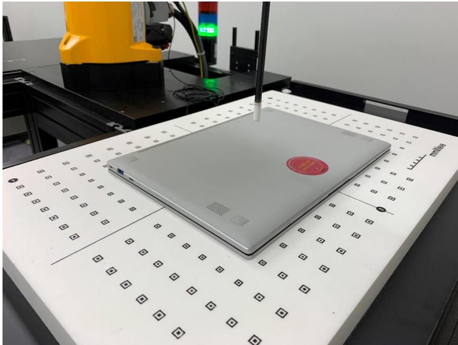
Rear (S2) View of the DUT
