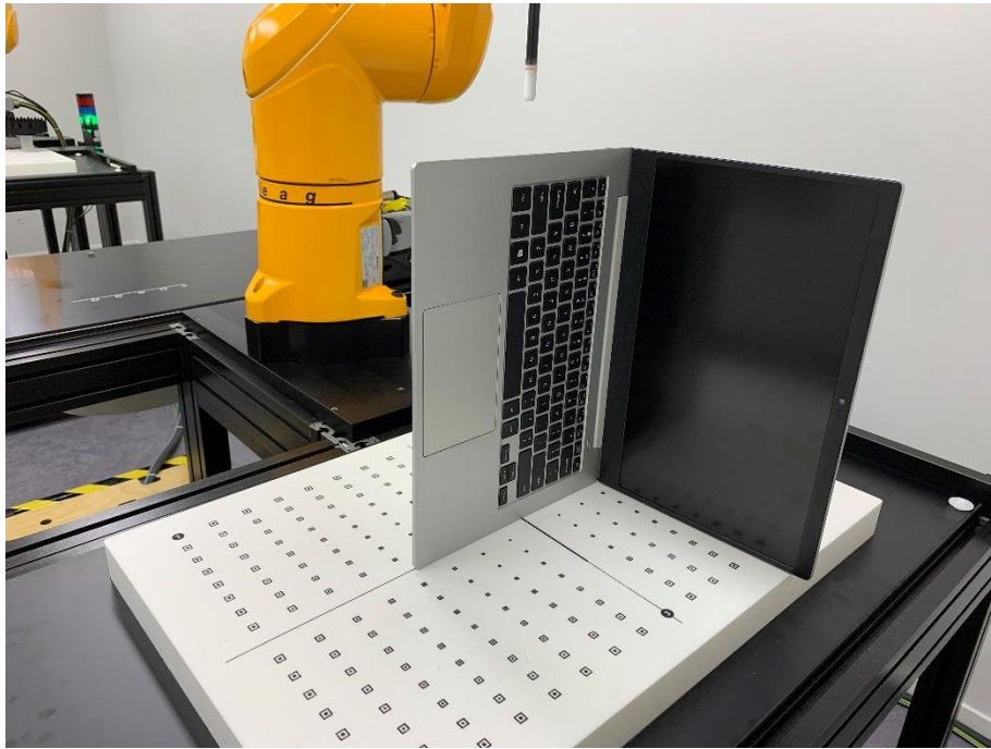
Left (S4) View of the DUT
