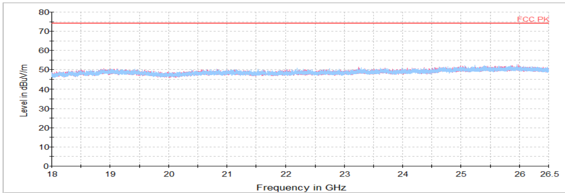
Horizontal/Vertical for 18 GHz ~ 26.5 GHz
