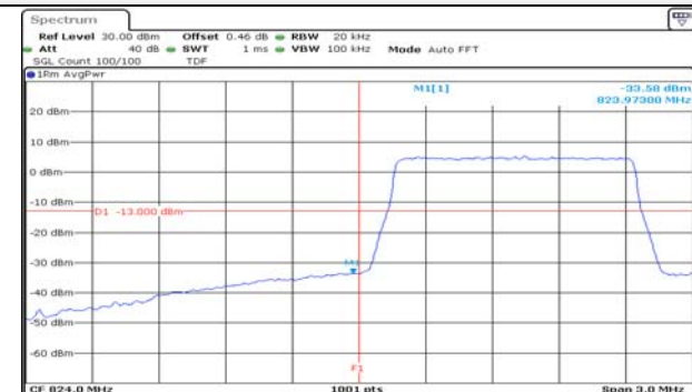
1.4M BW 16QAM Low ch. FRB
