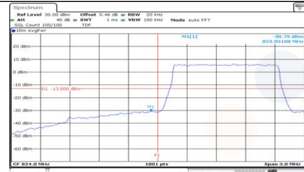
1.4M BW QPSK Low ch. FRB
