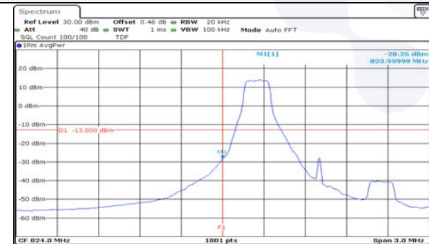
1.4M BW 16QAM Low ch. 1RB
