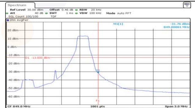
1.4M BW 16QAM High ch. 1RB
