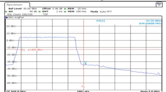
1.4M BW 16QAM High ch. FRB
