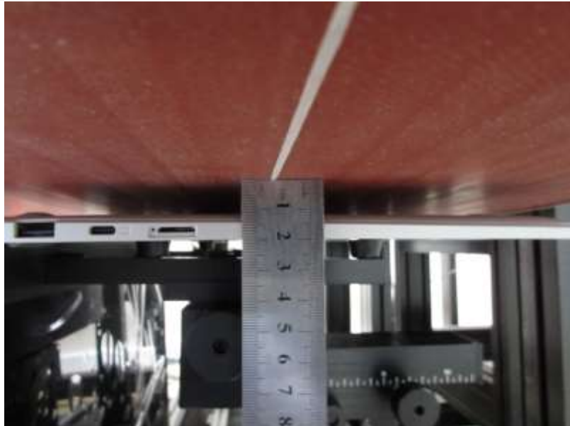
Distance of 6 mm from the EUT (WiFi ANT.1)
