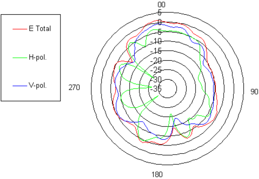
Main antenna @5.15 GHz
