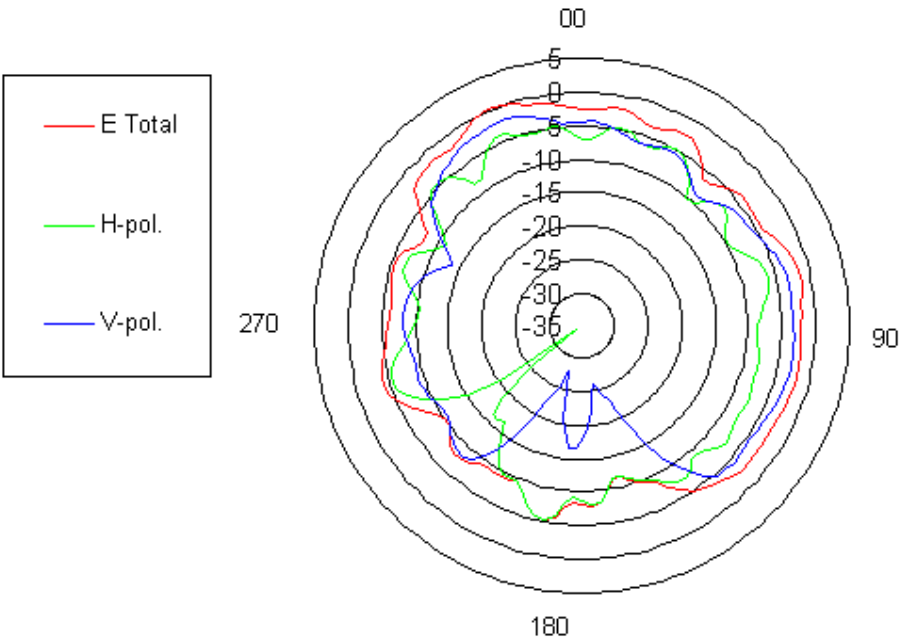
Main antenna @5.47 GHz
