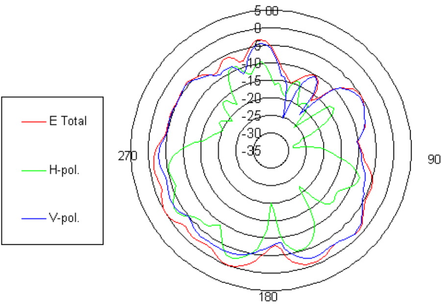
Aux antenna @5.25 GHz
