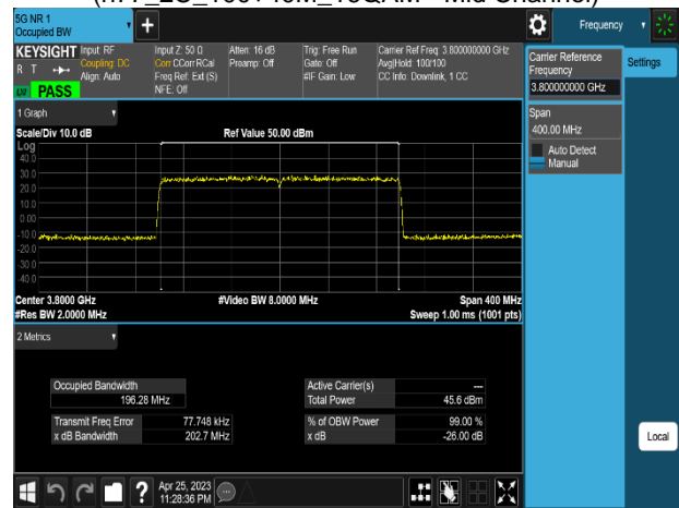
Plot 8-12. Occupied Bandwidth Plot (n77_2C_100+100M_16QAM - Mid Channel)
