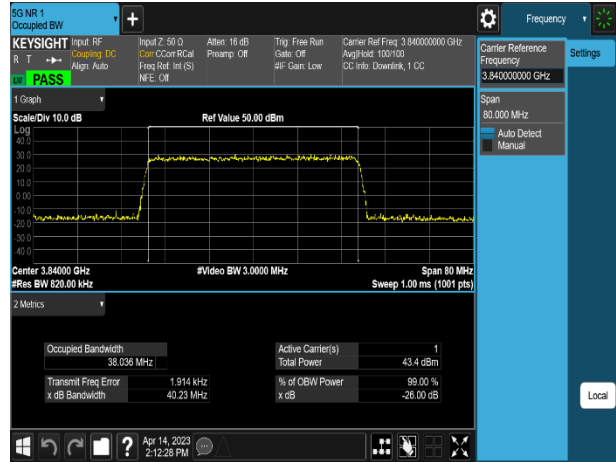
Plot 8-2. Occupied Bandwidth Plot (n77_1C_40M_256QAM - Mid Channel)
