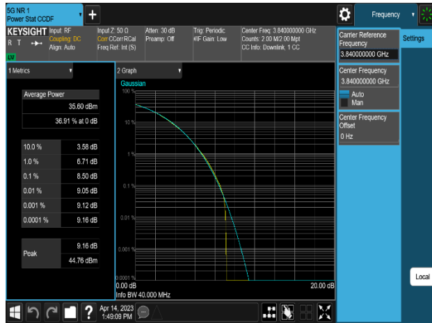
Plot 8-25. Peak To Average Power Ratio Plot (n77_1C_40M_16QAM - Mid Channel)
