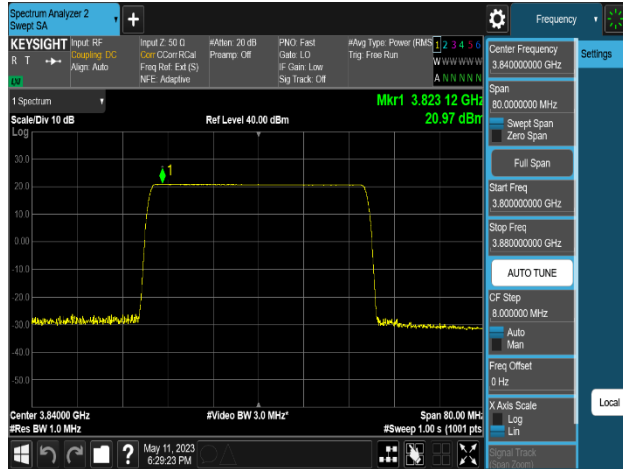
Plot 8-13. Power Spectral Density Plot (n77_1C_40M_QPSK - Mid Channel, Port 57)
