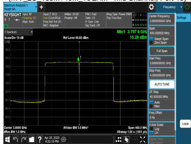
Plot 8-24. Power Spectral Density Plot (n77_2C_100M+100M_16QAM - Mid Channel, Port 19)
