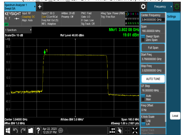
Plot 8-17. Power Spectral Density Plot (n77_1C_80M_QPSK - Mid Channel, Port 19)
