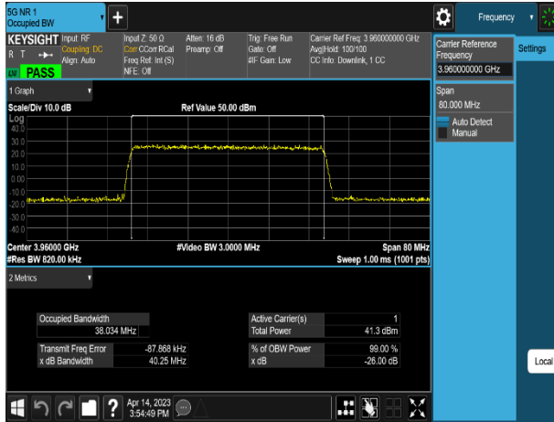
Plot 8-1. Occupied Bandwidth Plot (n77_1C_40M_QPSK - High Channel)
