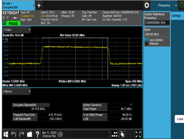
Plot 8-7. Occupied Bandwidth Plot (n77_1C_100M_QPSK - High Channel)
