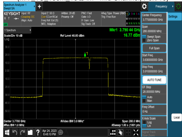
Plot 8-22. Power Spectral Density Plot (n77_2C_100M+40M_16QAM - Mid Channel, Port 19)
