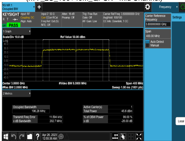
Plot 8-11. Occupied Bandwidth Plot (n77_2C_100+100M_QPSK - Mid Channel)
