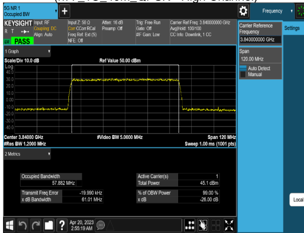
Plot 8-3. Occupied Bandwidth Plot (n77_1C_60M_QPSK - Mid Channel)
