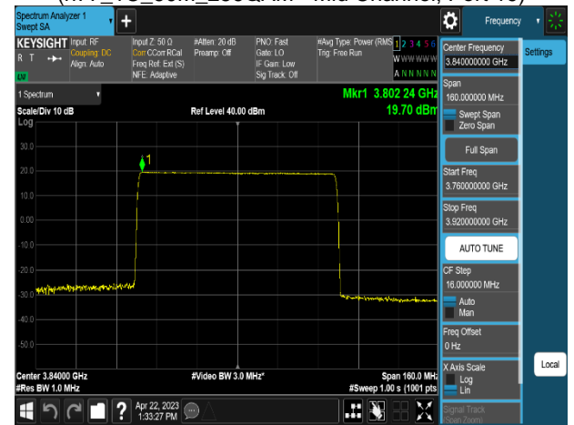
Plot 8-18. Power Spectral Density Plot (n77_1C_80M_64QAM - Mid Channel, Port 19)
