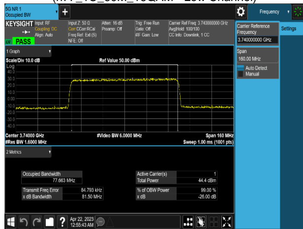
Plot 8-6. Occupied Bandwidth Plot (n77_1C_80M_16QAM - Low Channel)
