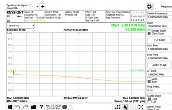
3981 MHz - 4000 MHz
