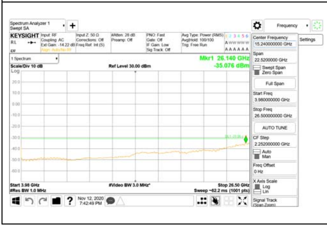
3980 MHz - 26.5 GHz
