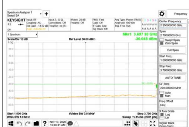
1000 MHz - 3700 MHz
