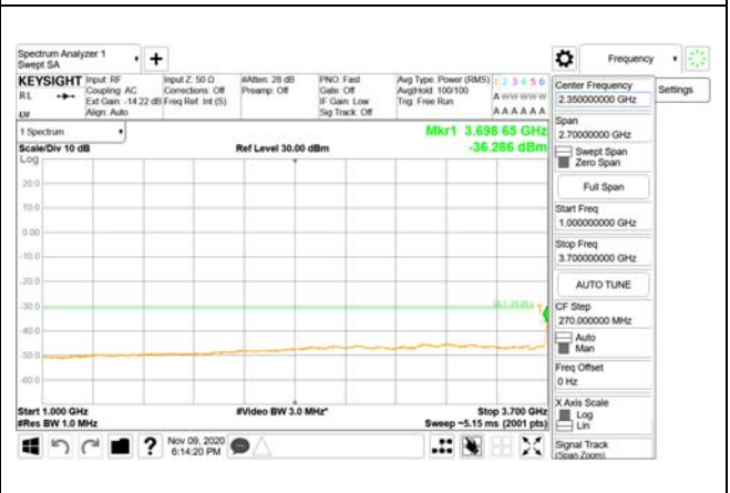
1000 MHz - 3700 MHz
