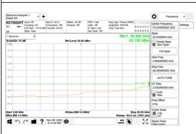
3980 MHz - 26.5 GHz
