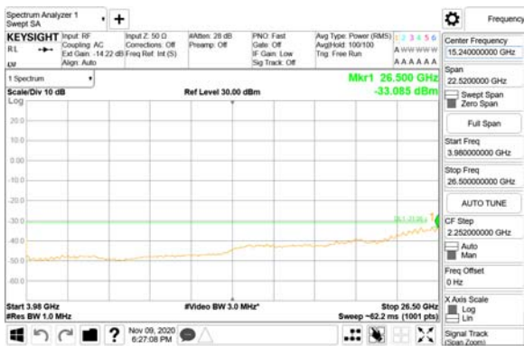
3980 MHz - 26.5 GHz
