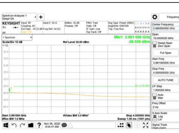
3981 MHz - 4000 MHz
