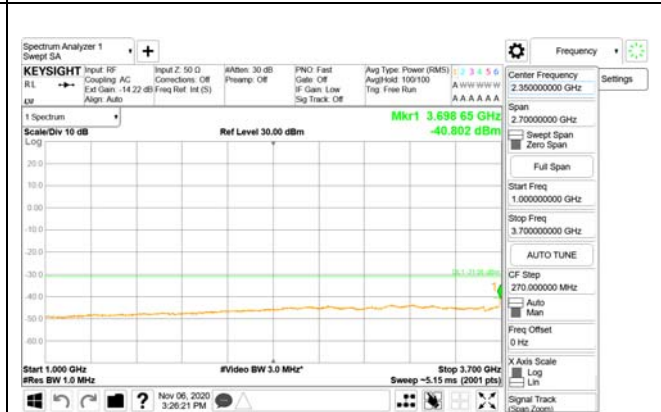
1000 MHz - 3700 MHz
