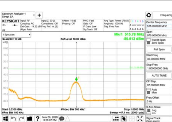
30 MHz - 1000 MHz
