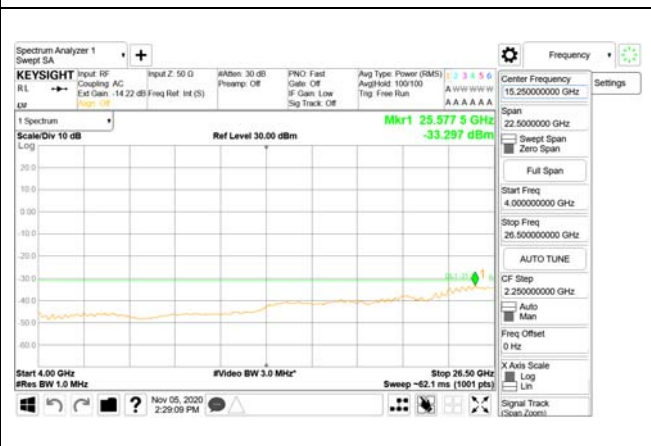
4000 MHz - 26.5 GHz
