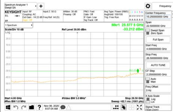
4000 MHz - 26.5 GHz
