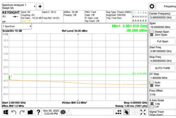
3981 MHz - 4000 MHz
