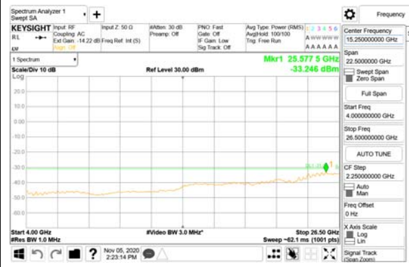
4000 MHz - 26.5 GHz
