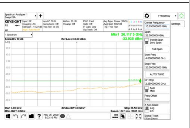
4000 MHz - 26.5 GHz
