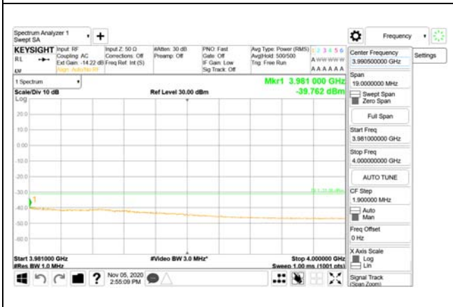
3981 MHz - 4000 MHz
