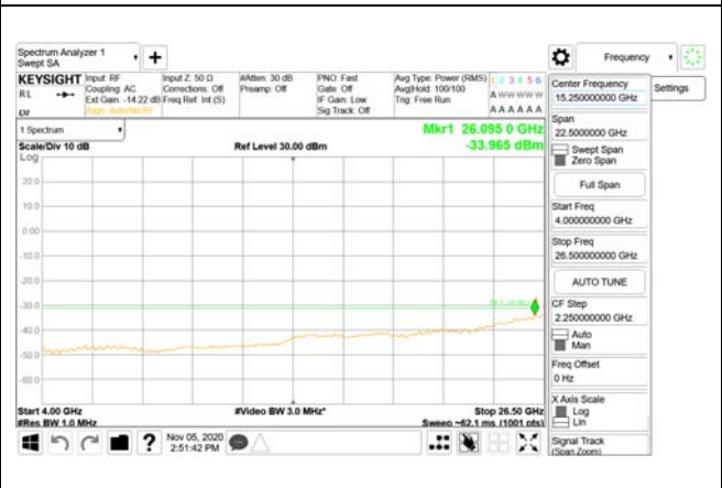
4000 MHz - 26.5 GHz
