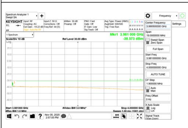
3981 MHz - 4000 MHz
