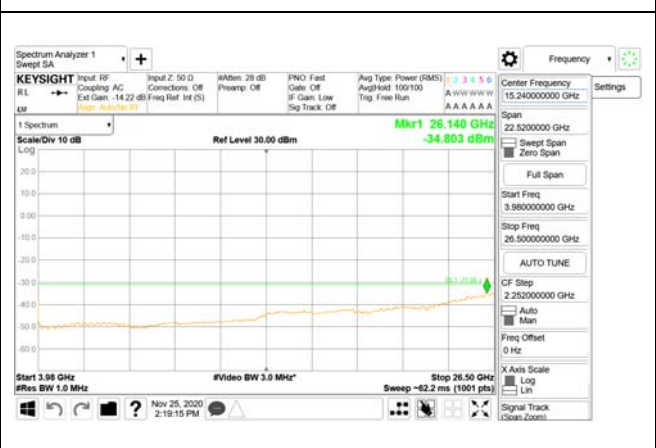
3980 MHz - 26.5 GHz
