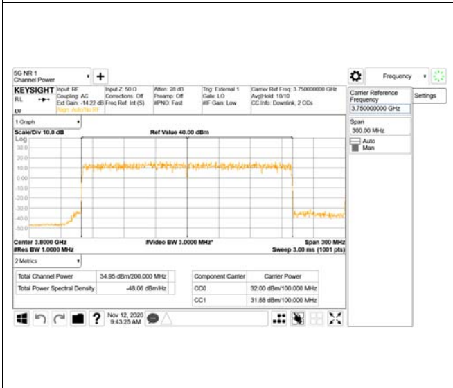
64QAM
