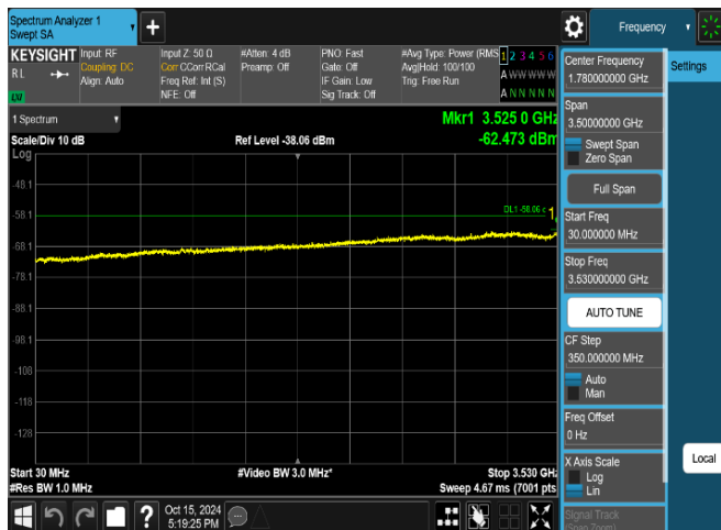
Plot 8-51. Conducted Spurious Emission Plot 30 MHz to 3.53 GHz (NR_3NC_40M+20M+20M_QPSK – Mid Channel, Port 48)
