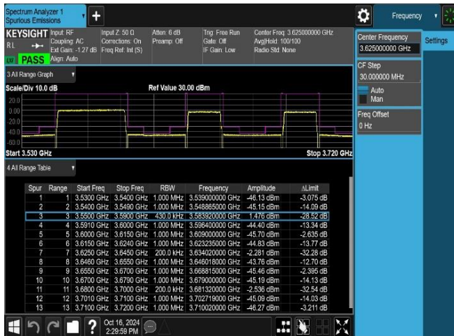
Plot 8-37. Channel Edge Emission Plot (NR_3NC_40M+20M+20M_QPSK– Mid Channel, Port 4)
