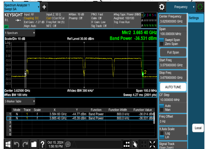
Plot 8-32. Channel Edge Emission Plot (RBW 1% of fundamental for measurements within 1 MHz band power) (NR_3C_40M+20M+20M_QPSK– Mid Channel, Port 4)
