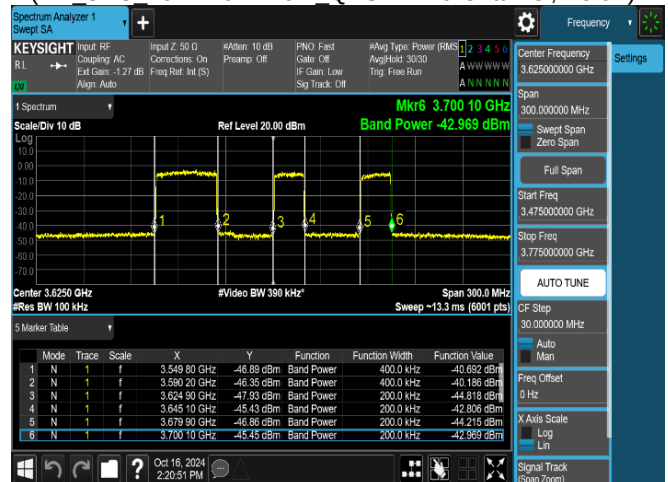
Plot 8-38. Channel Edge Emission Plot (RBW 1% of fundamental for measurements within 1 MHz band power) (NR_3NC_40M+20M+20M_QPSK– Mid Channel, Port 4)
