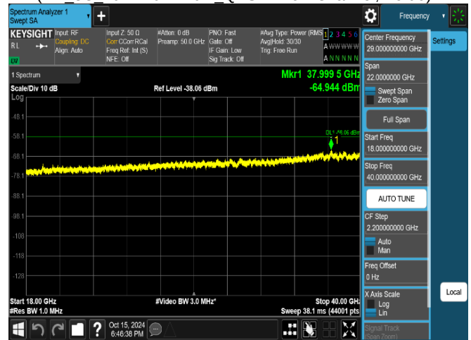
Plot 8-42. Conducted Spurious Emission Plot 18 GHz to 40 GHz (NR_3C_20M+20M+20M_QPSK - Low Channel, Port 9)
