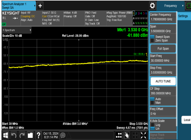
Plot 8-39. Conducted Spurious Emission Plot 30 MHz to 3.53 GHz (NR_3C_20M+20M+20M_QPSK - Low Channel, Port 9)
