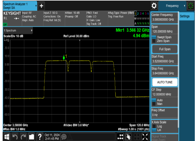
Plot 8-6. Power Spectral Density Plot (NR_3C_20M+20M+20M_16QAM - Low Channel, Port 1)
