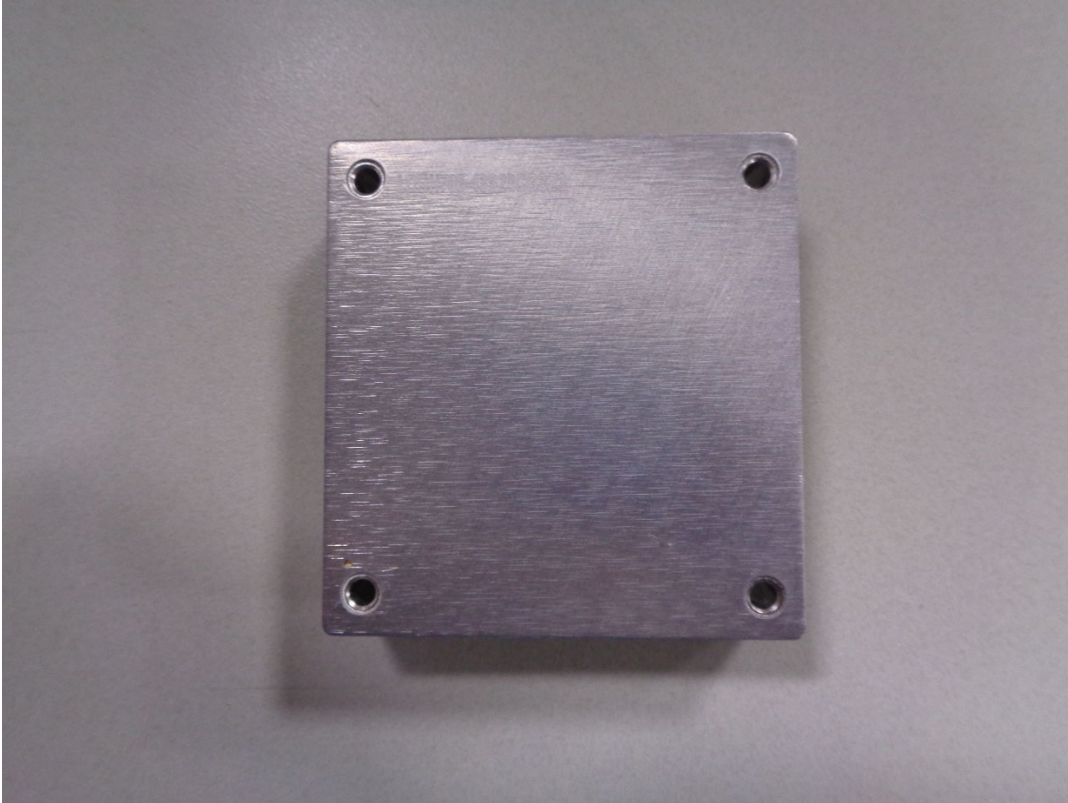
Al Base Plate (Top)
