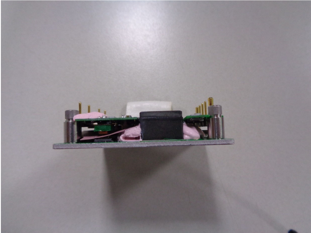
Side View with Plastic Housing Removed
