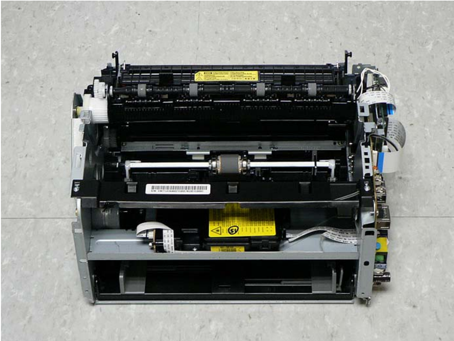
ML-1670_Internal_Front Side
