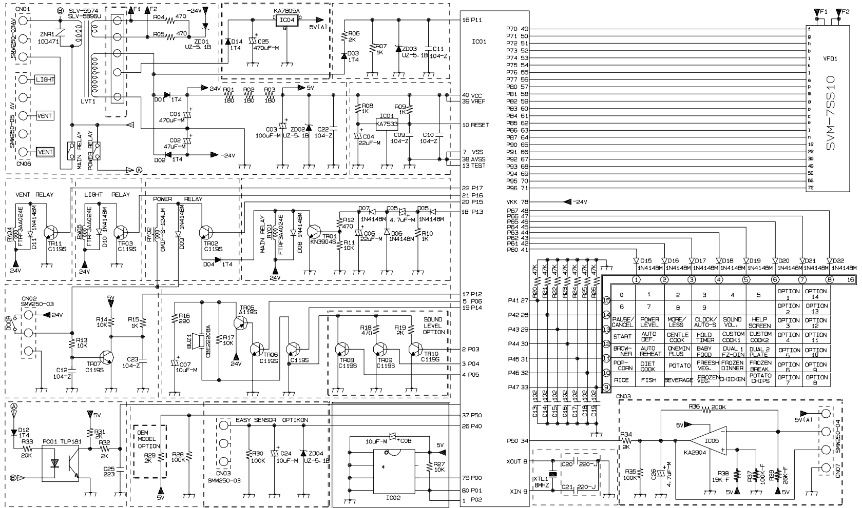
S22USA SCHEMATIC
