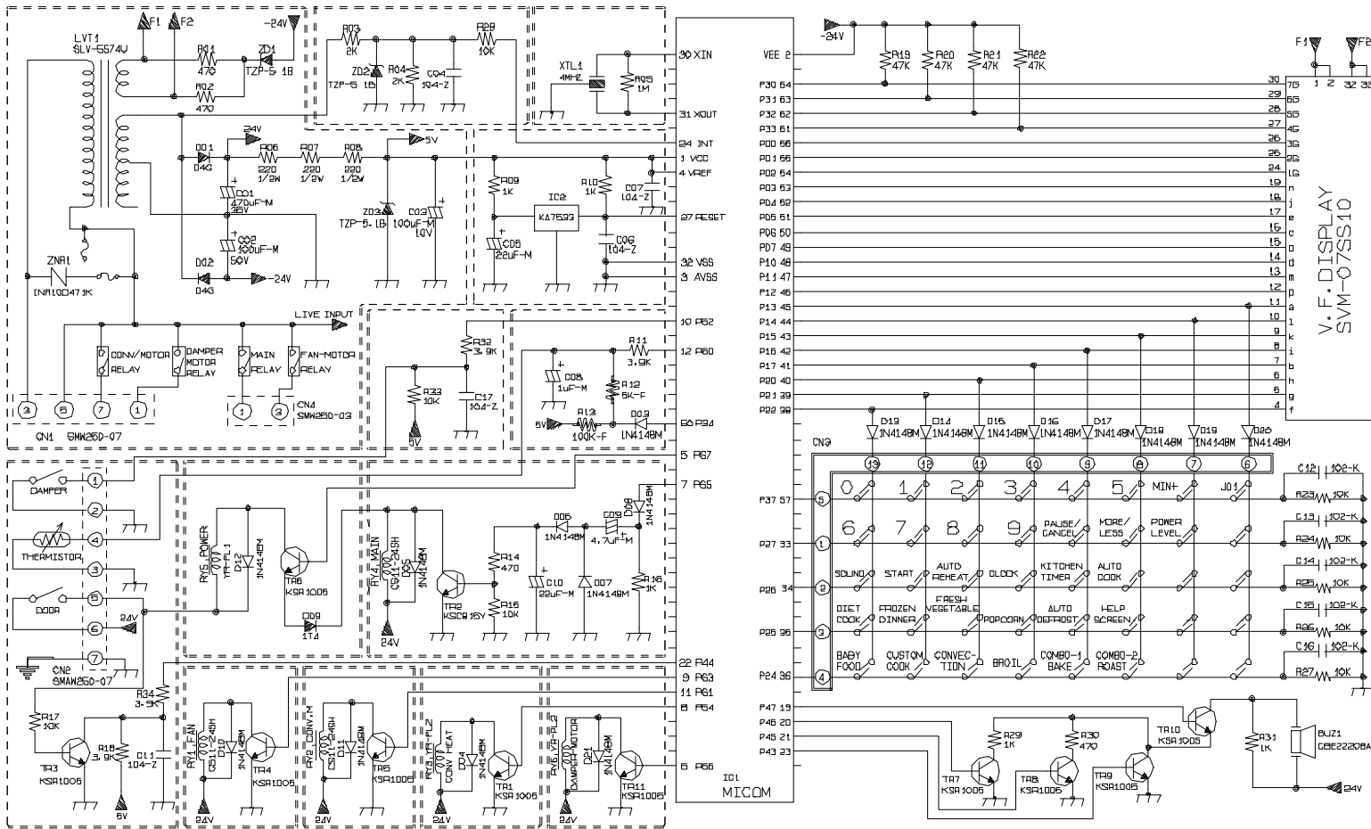
ELECTRIC-DIAGRAM MC5694
