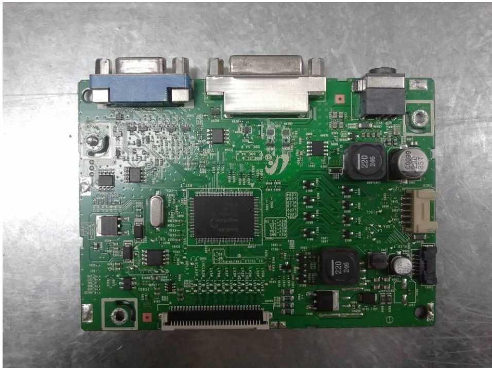
(Main Board )
