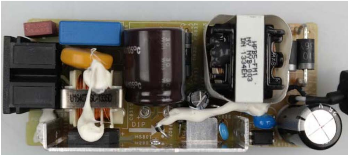
Before change A2514_DSM external rear view
