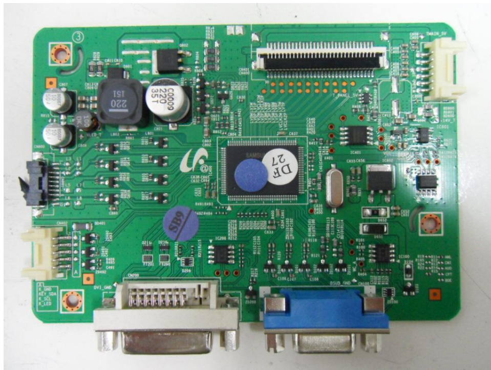
(Board 1)
