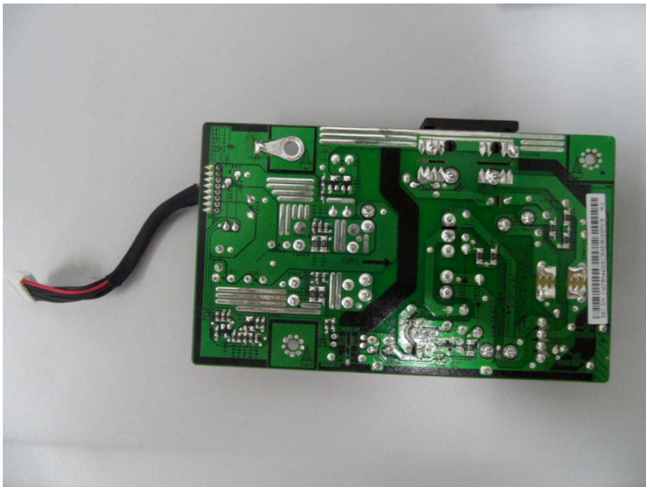
Before change IP-35185A(old) internal front view
