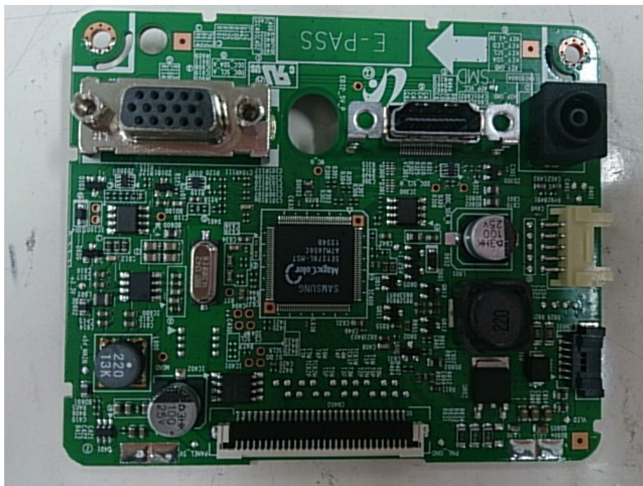
(Main Board )
