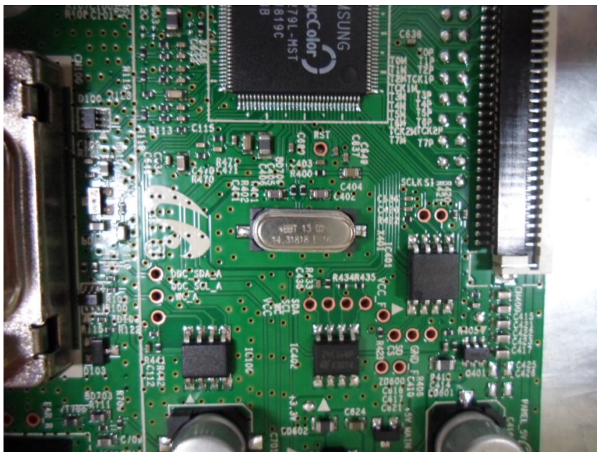
(Crystal Main Board)
