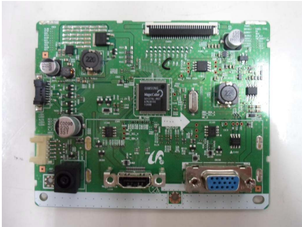
Before change BN41-01962A internal front view
