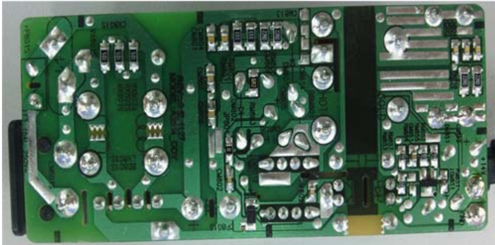
Back change A2514_DDY internal rear view
