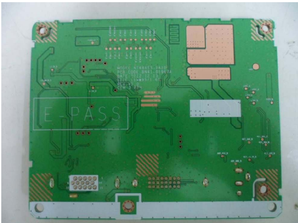
Before change BN41-01967A (VGA+DVI) Internal rear view
