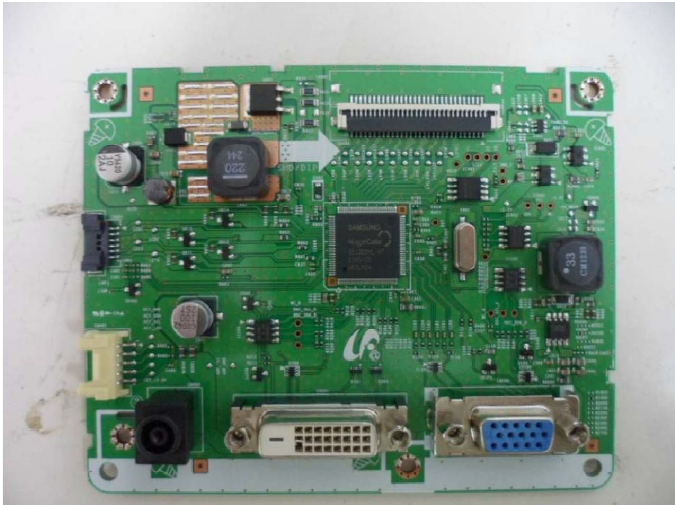
Before change BN41-01967A (VGA+DVI) Internal front view
