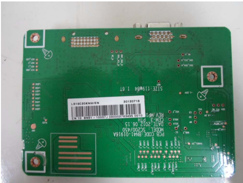
Before change SC200/450 (VGA) rear view
