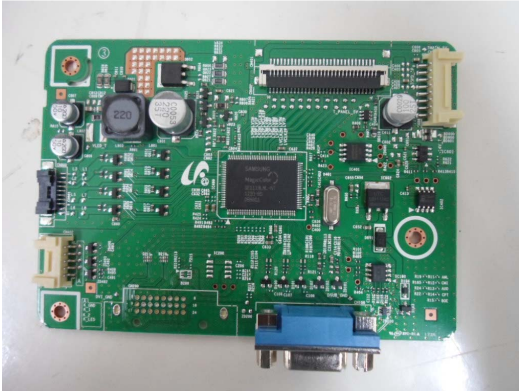
Before change SC200/450 (VGA) front view
