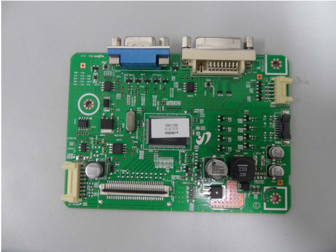
Back change SC200/450 (VGA+DVI) front view
