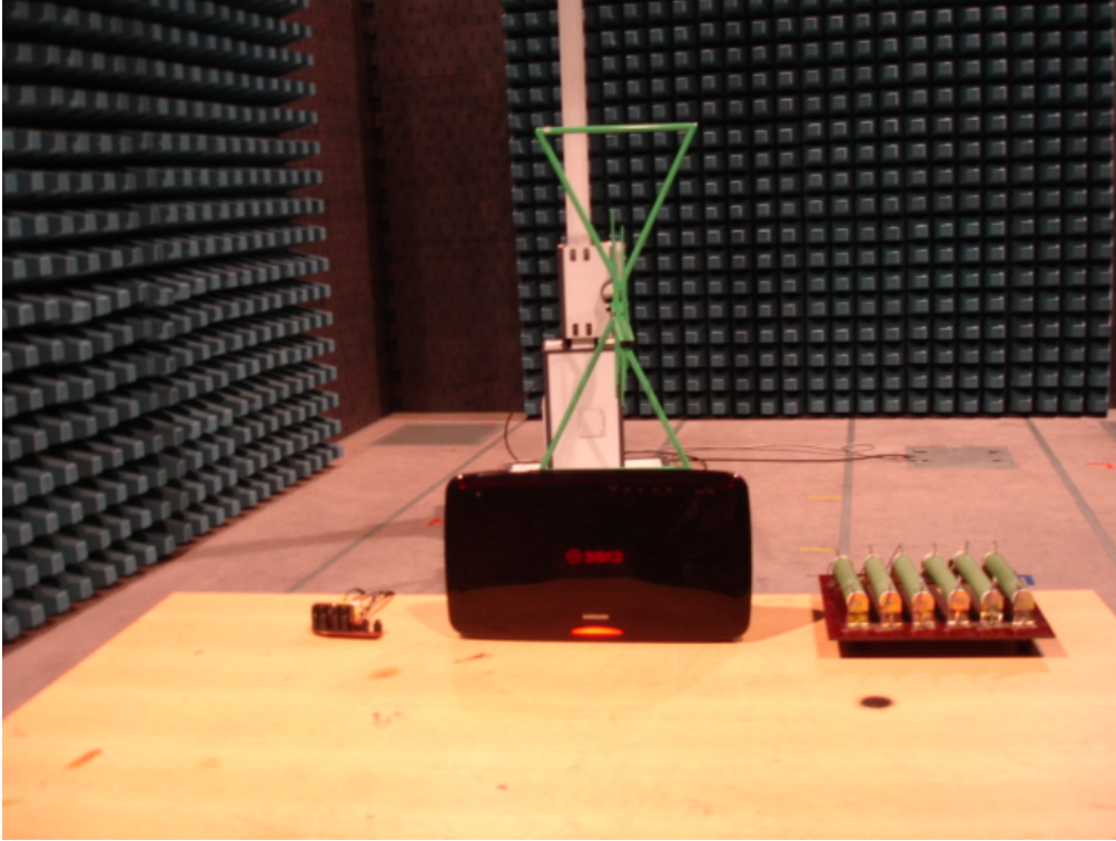
Photo 3 Radiated disturbances Test
