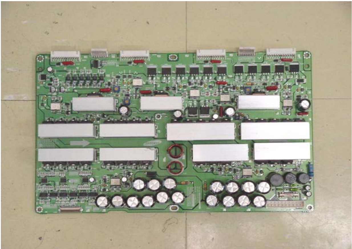
Y - BOARD TOP VIEW
