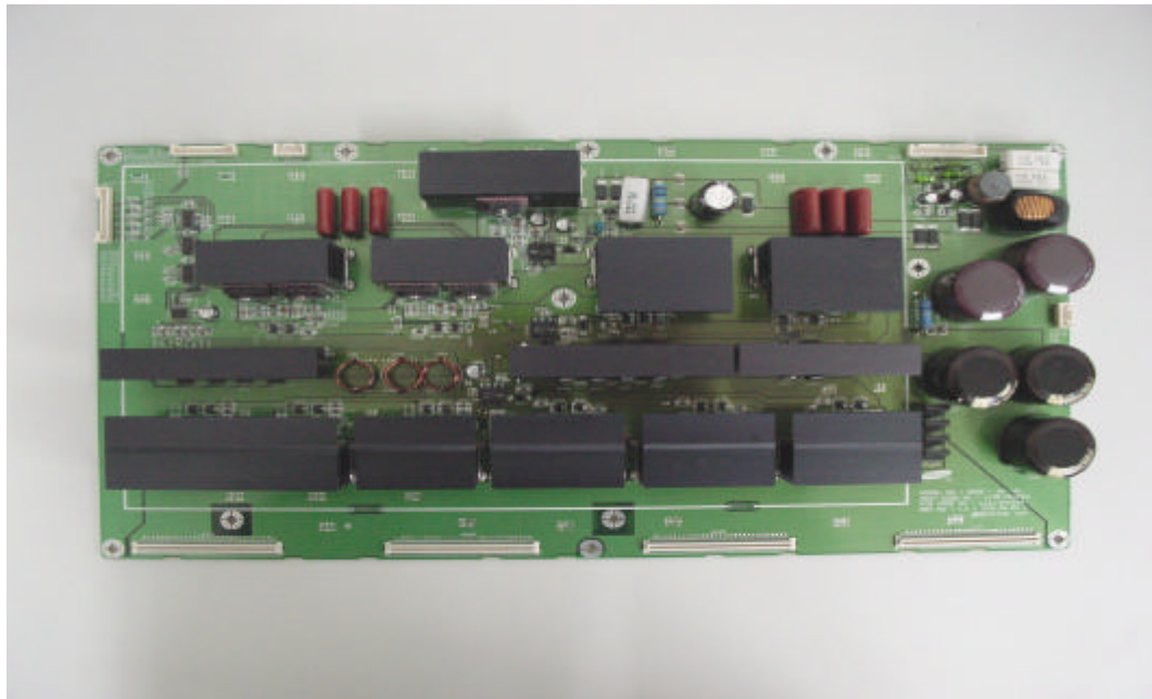
X-DRIVER BOARD TOP VIEW
