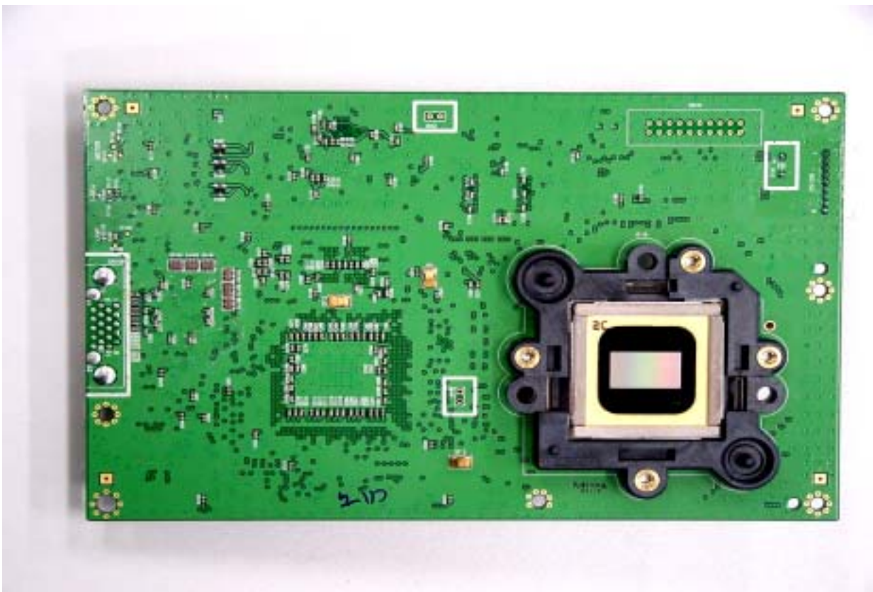
DMD BOARD BOTTOM VIEW
