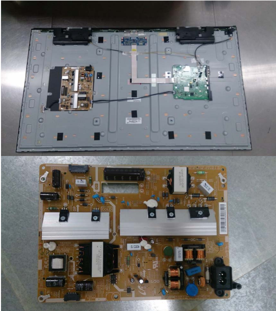
(Power Board)
