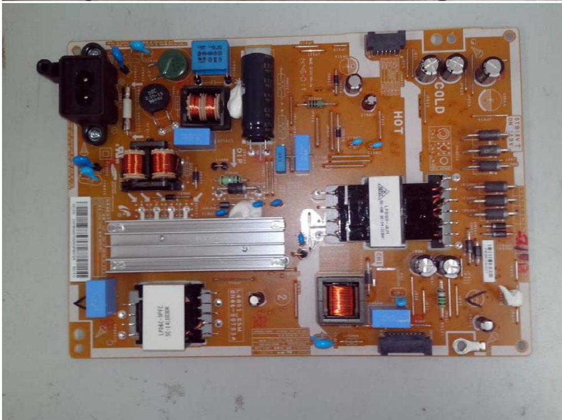
(Power Board)
